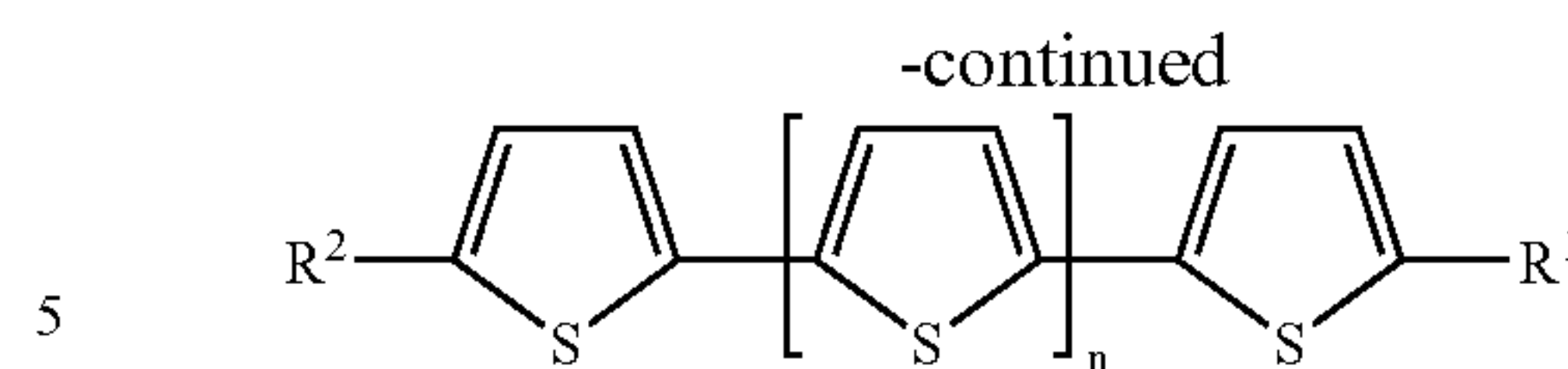
Oligothiophene
