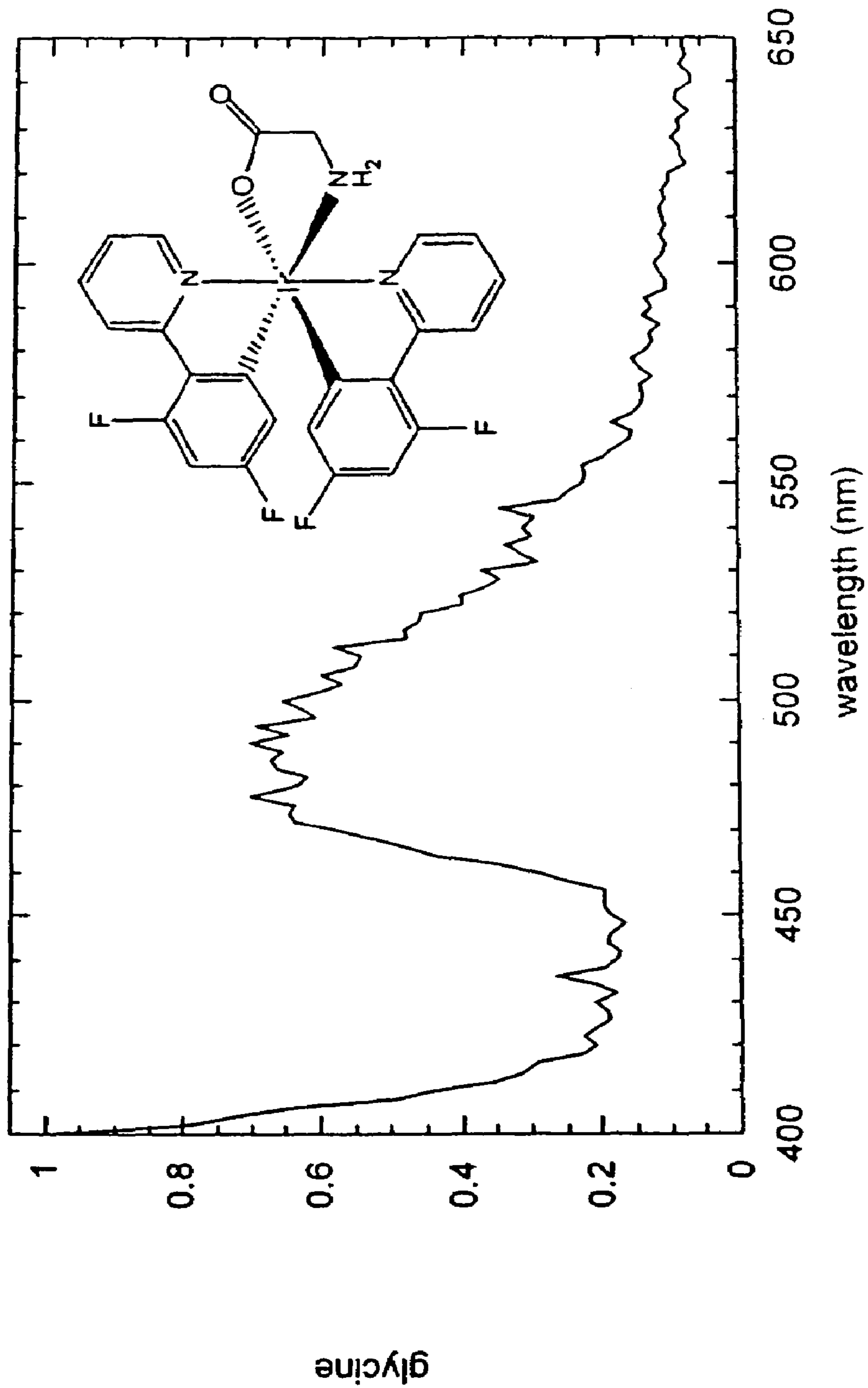
(4,6-F2ppy)2Ir(glycine)
