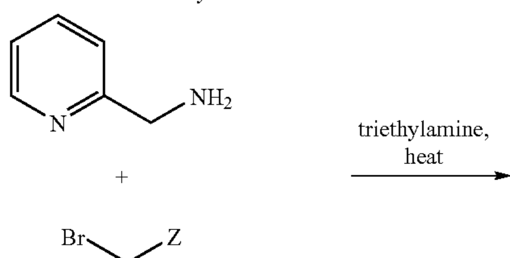
Scheme 1. Synthesis of various DPMA derivatives.
