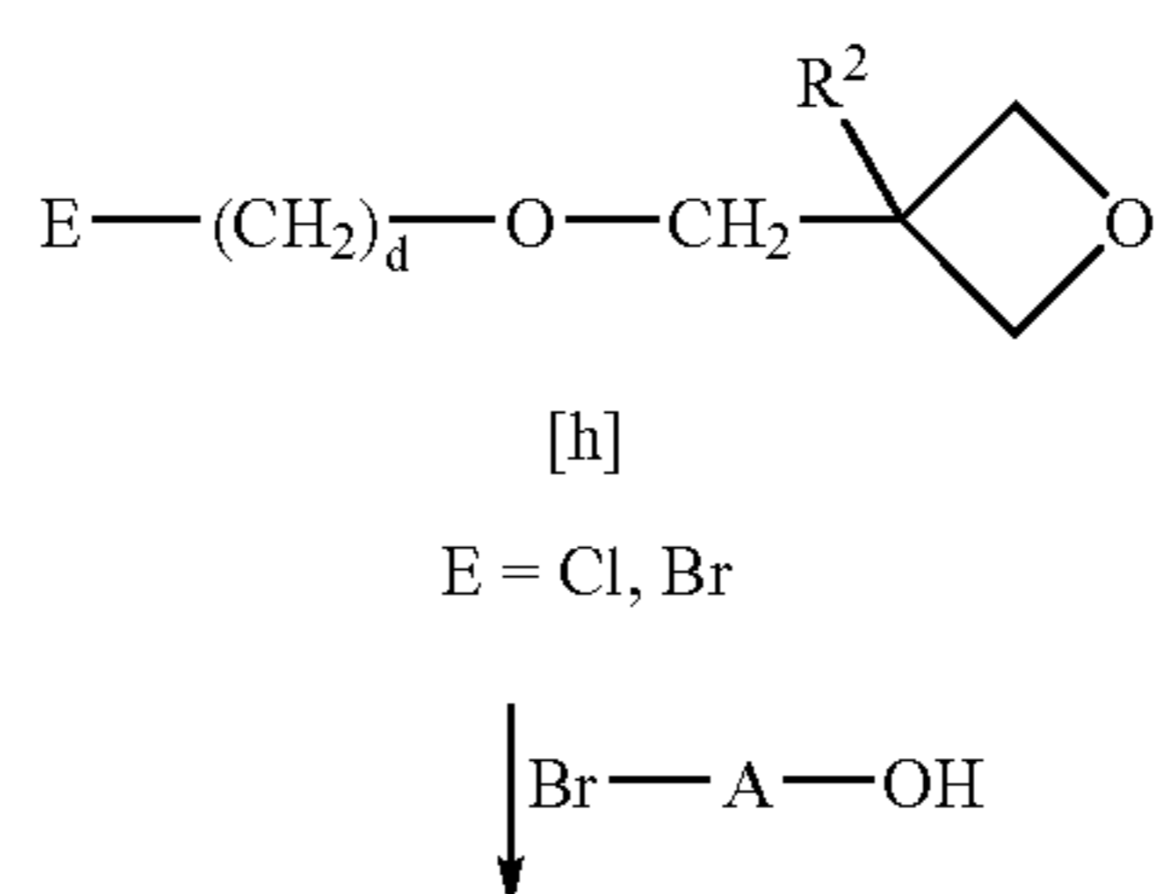
Scheme 3. Synthesis of the compound (8a) or (8b)
