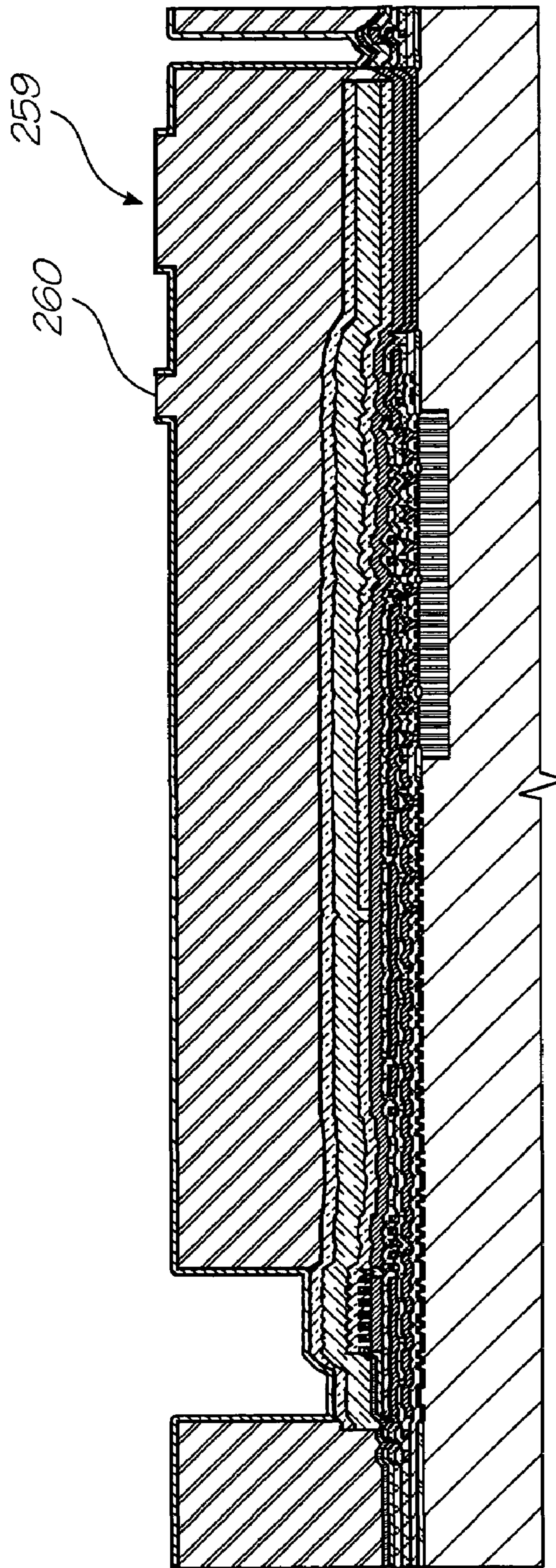
Form self-aligned nozzles using CMP
