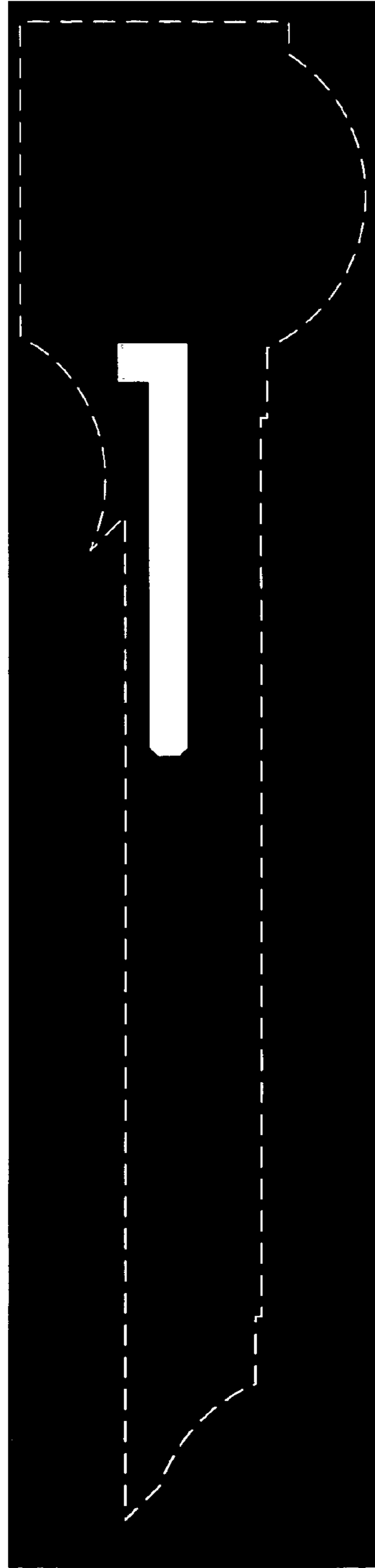
N-Well mask
