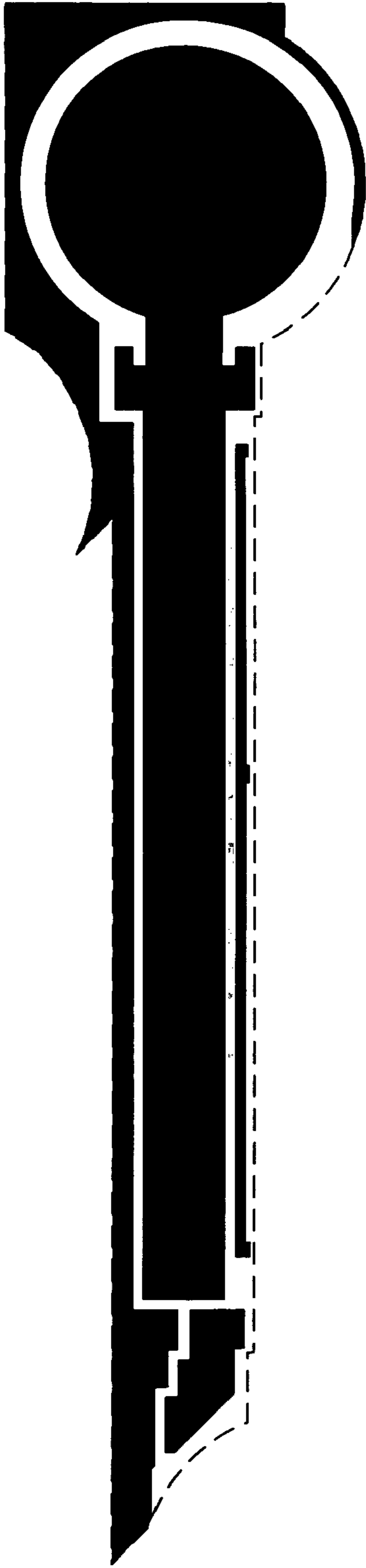
Metal 3 mask
