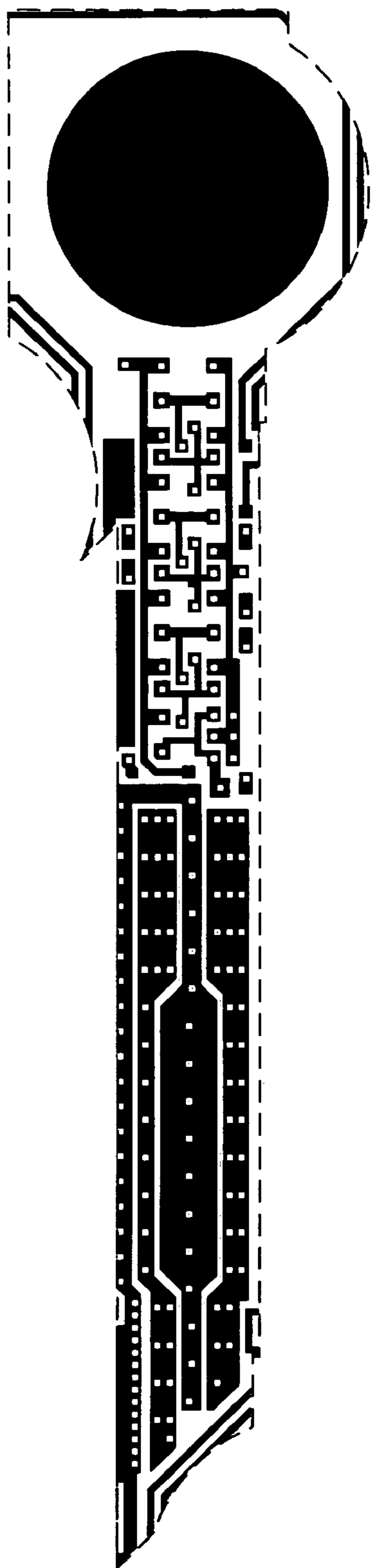
Metal 1 mask
