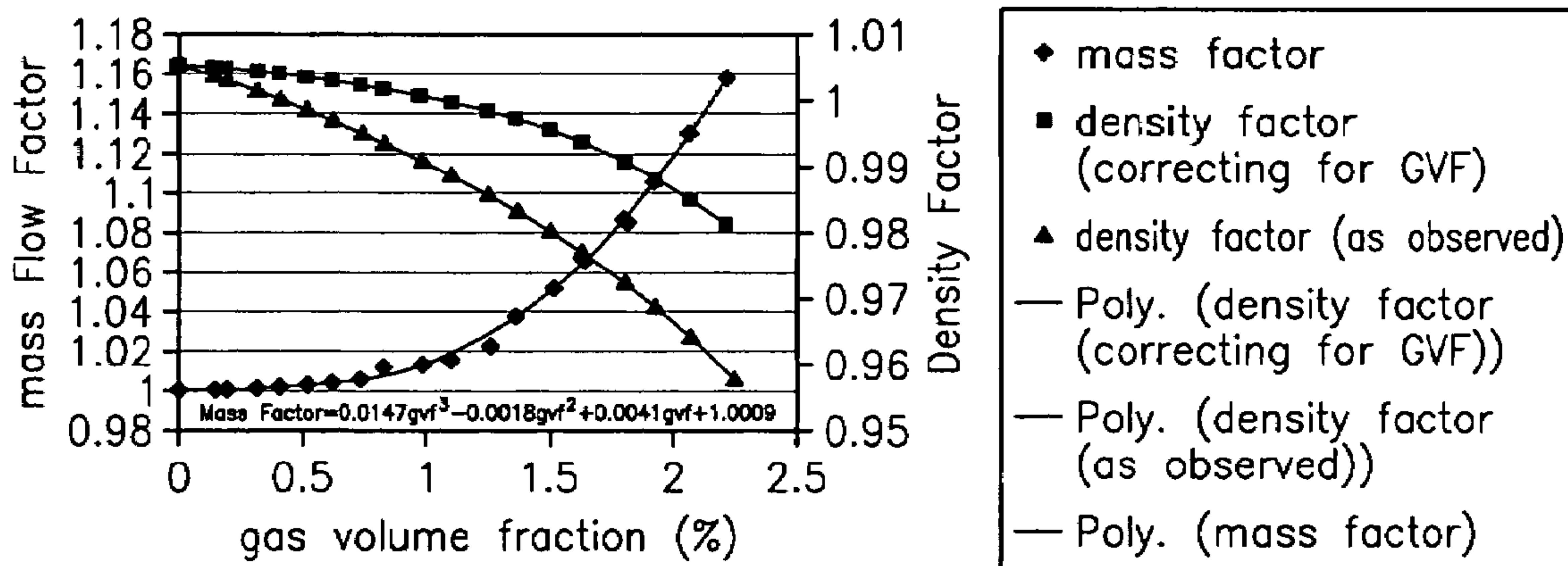
Effect of Entrained Air on Coriolis meter
