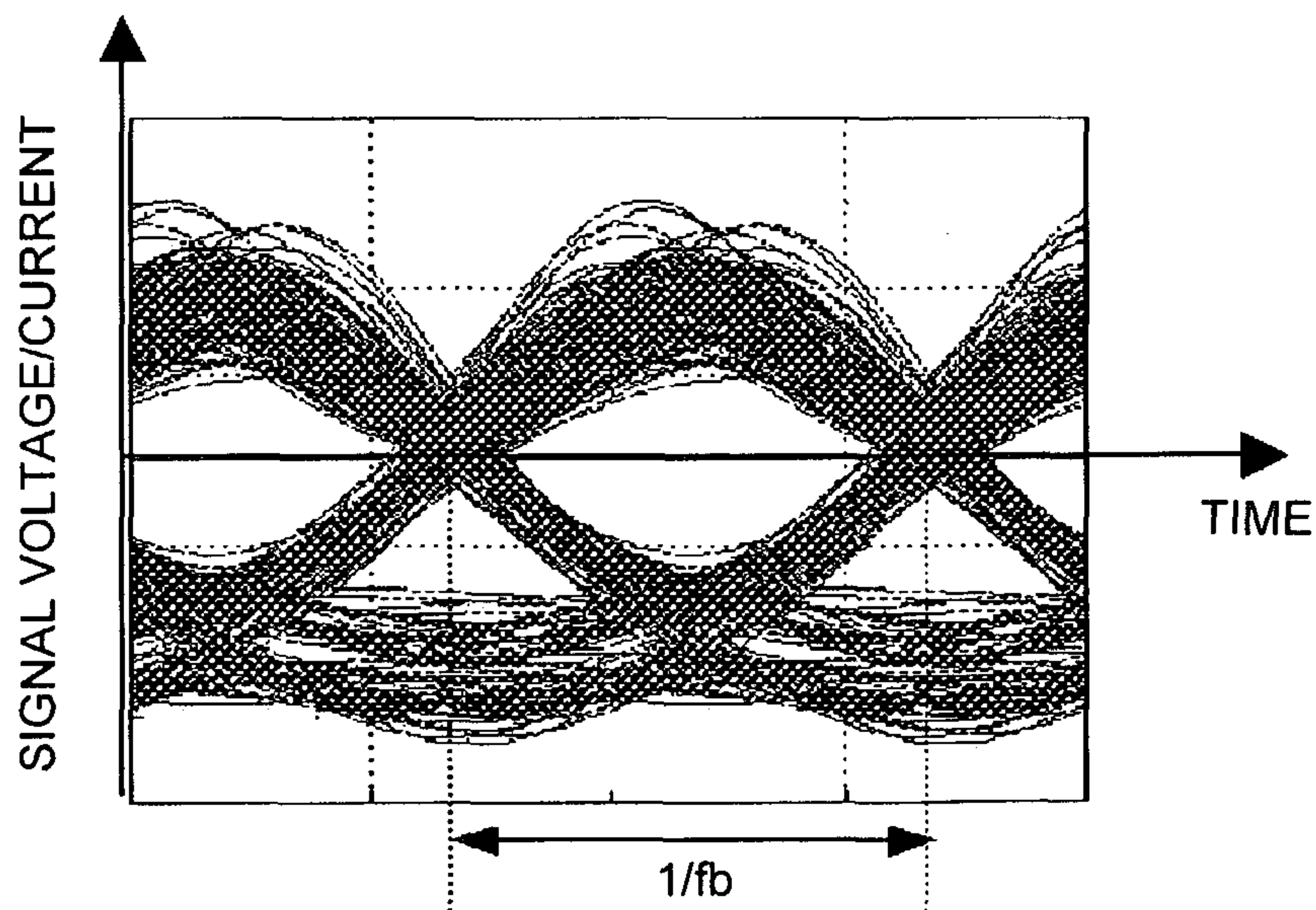
SIGNAL EYE PATTERN (WHEN REDUNDANT FREQUENCY COMPONENTS ARE FILTERED OUT)
