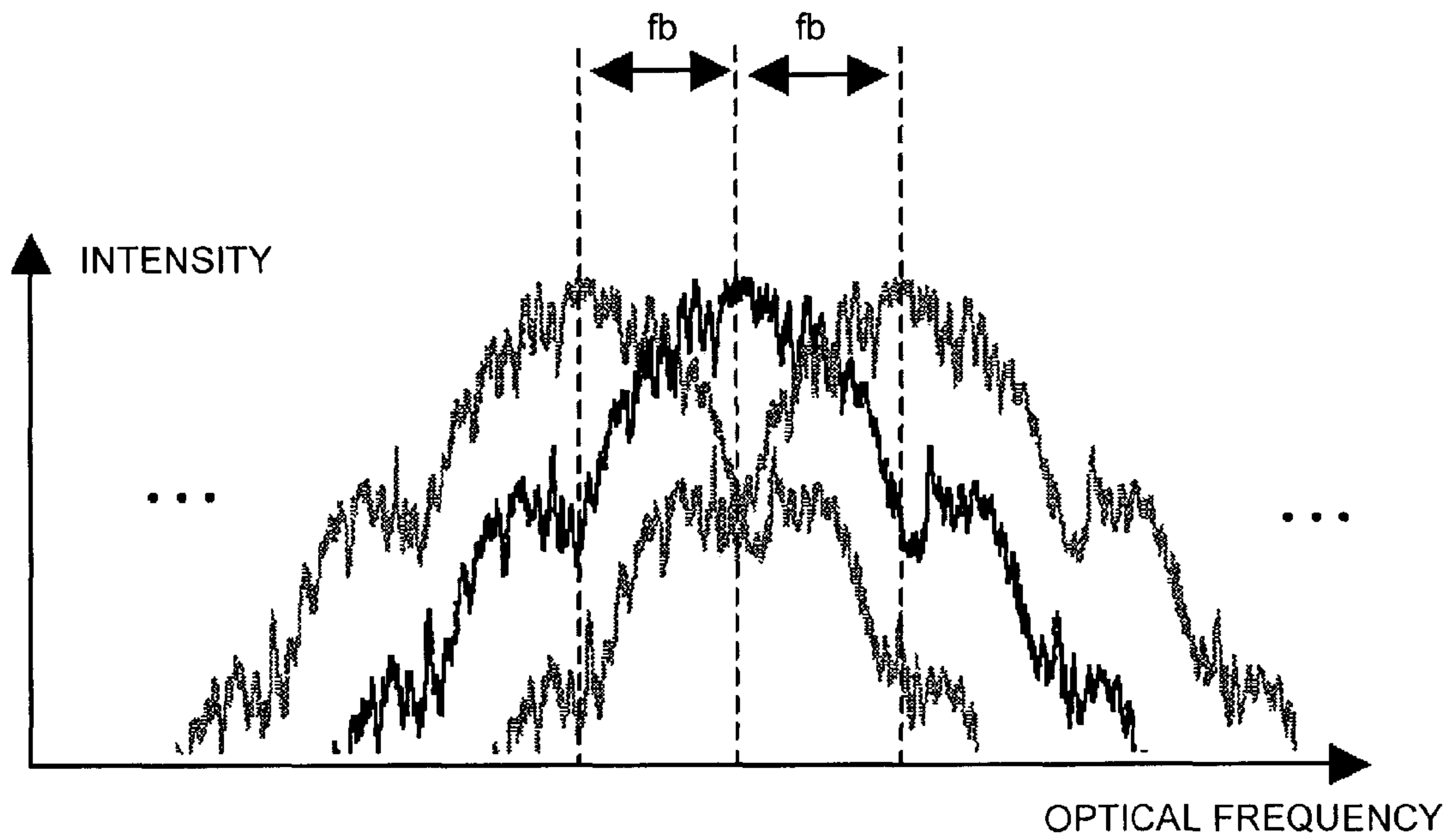
WAVELENGTH-MULTIPLIED SPECTRUM (WHEN REDUNDANT FREQUENCY COMPONENTS ARE NOT FILTERED OUT)
