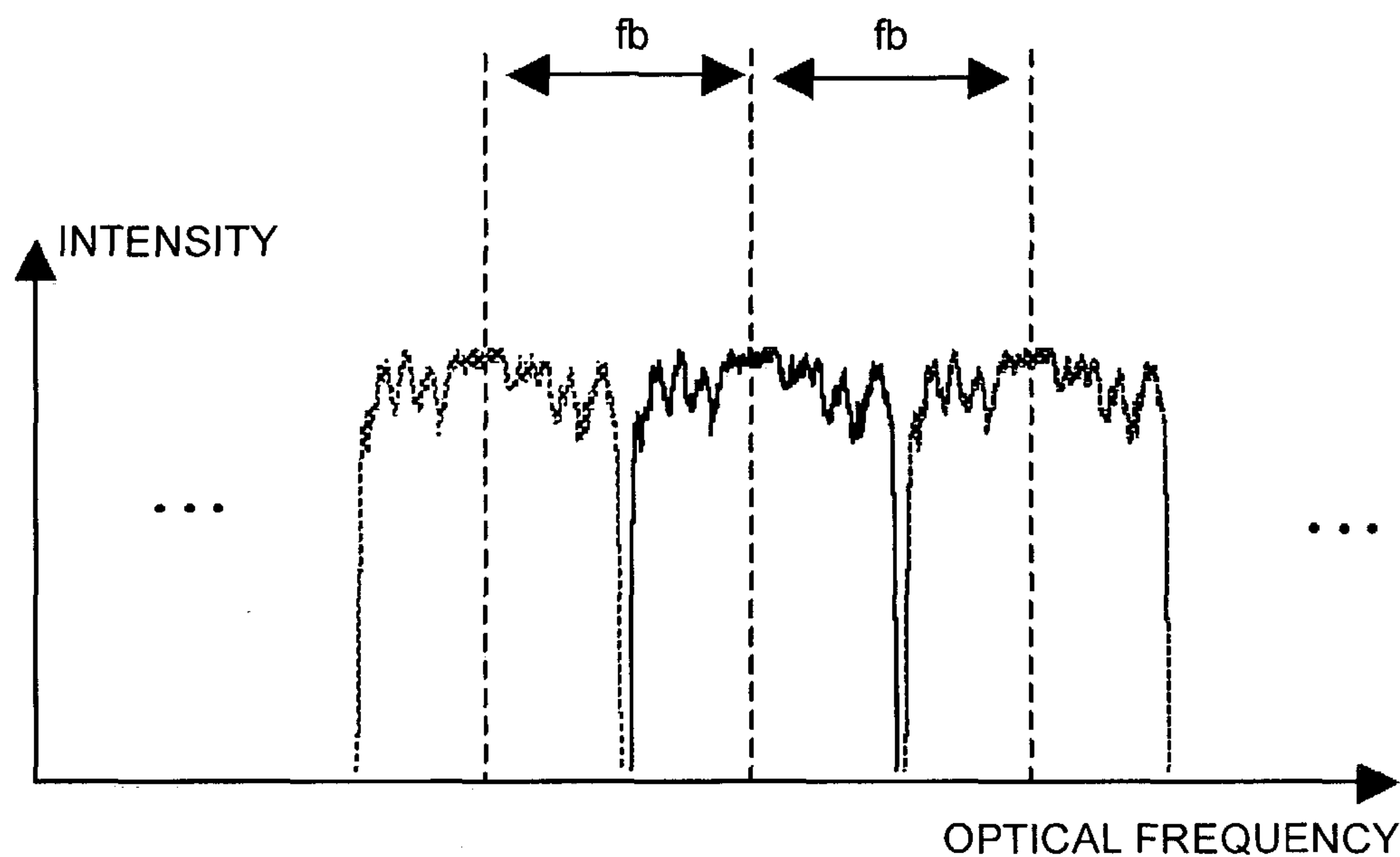
WAVELENGTH-MULTIPLEXED SPECTRUM (WHEN REDUNDANT FREQUENCY COMPONENTS ARE FILTERED OUT)
