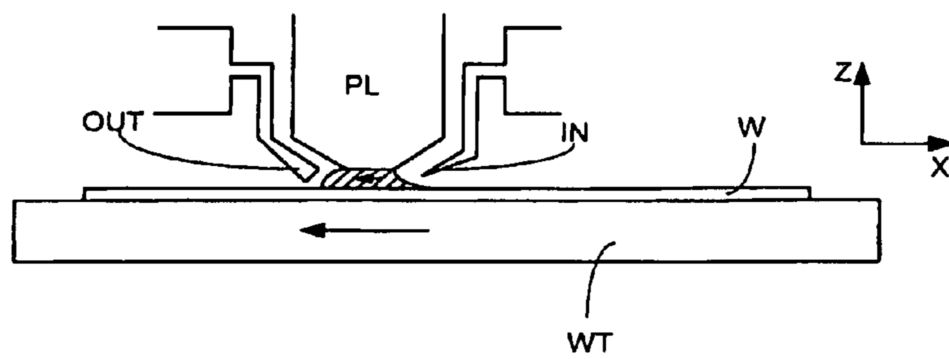
Fig. 2 (Prior Art)
