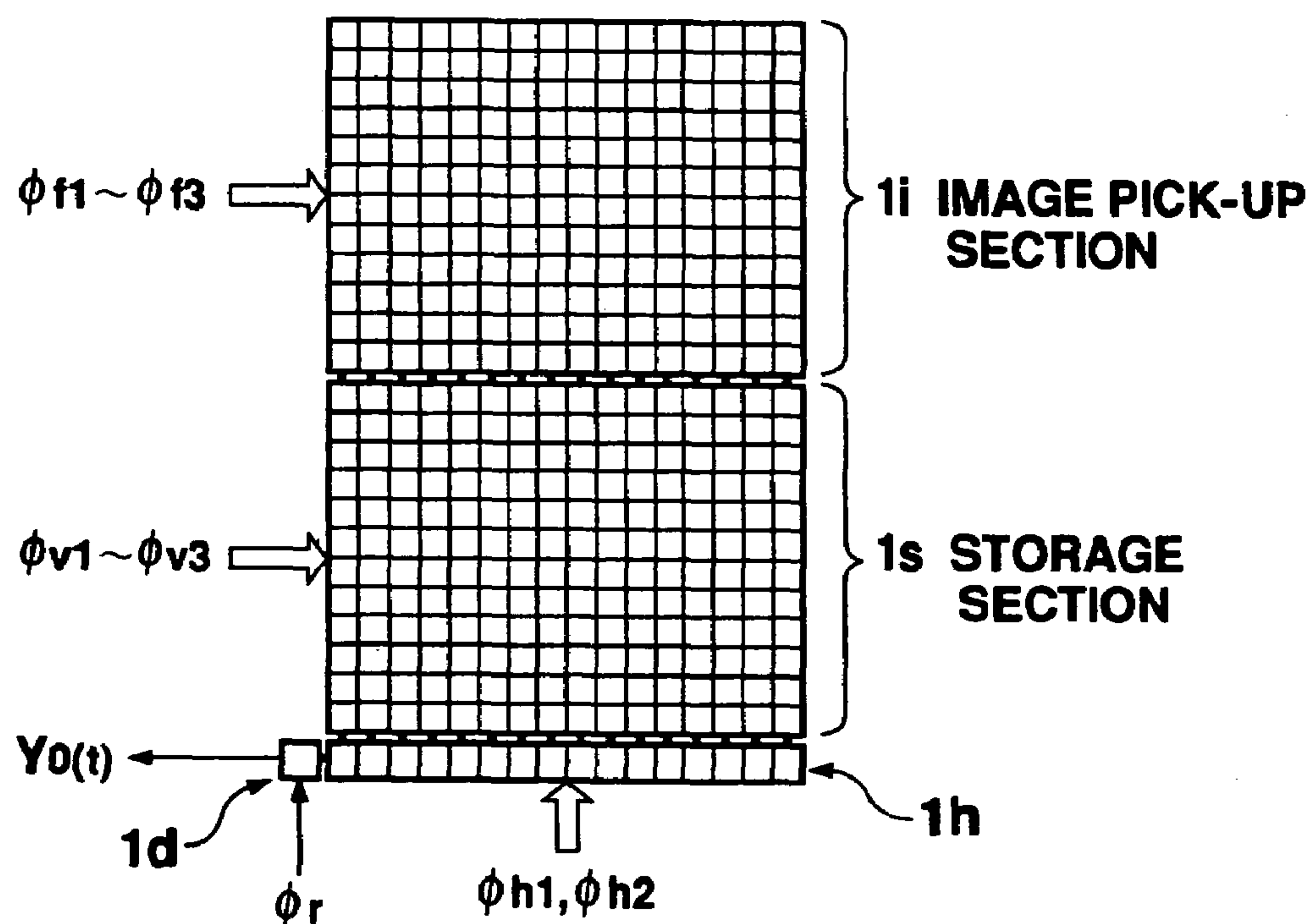
Fig. 2 PRIOR ART
