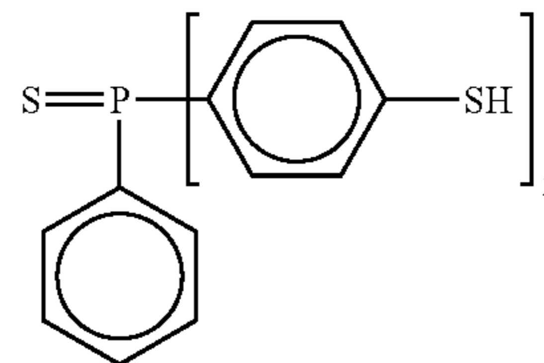
Bis(4-thiophenyl)phenyl phosphine sulfide (BTPPS)
