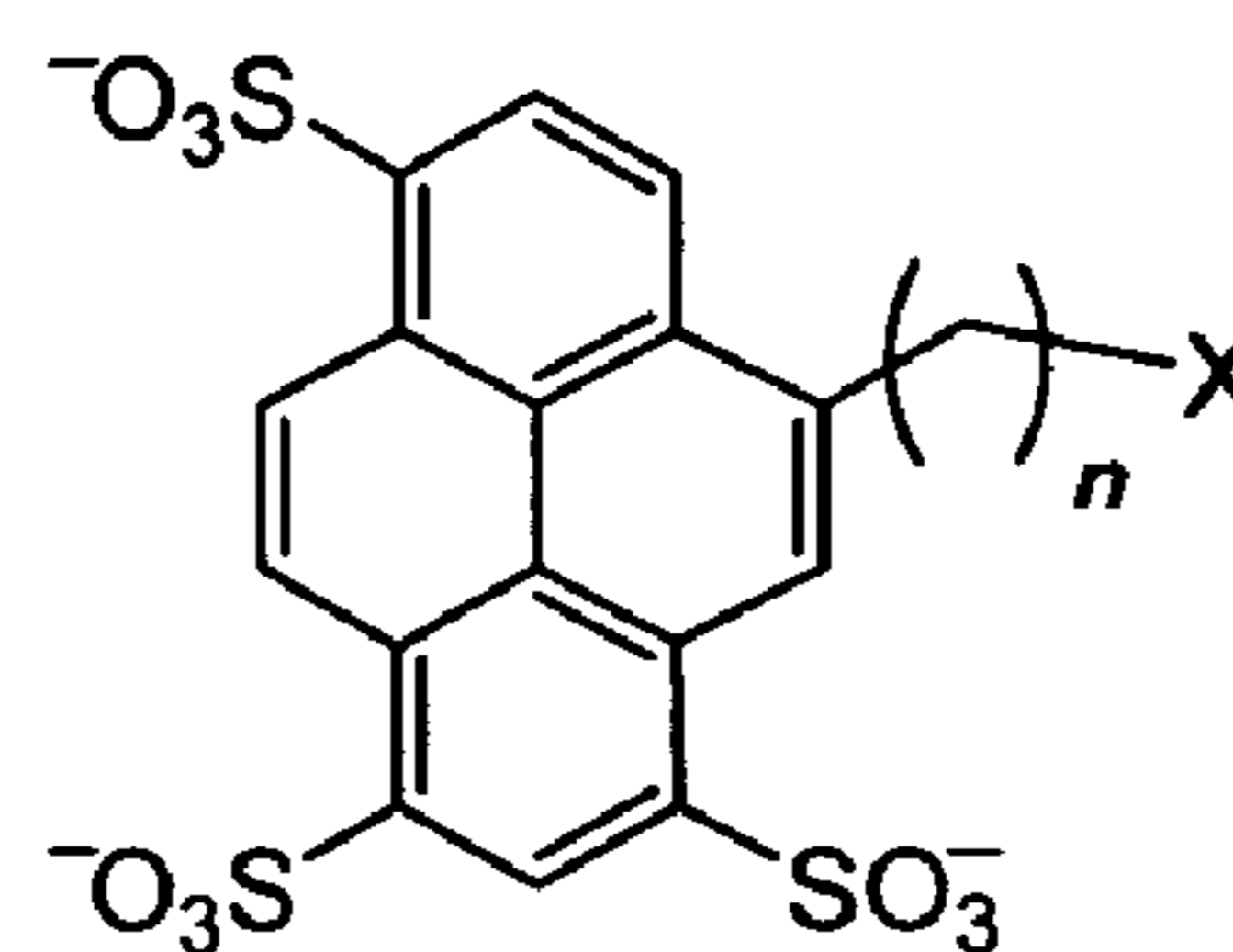
DYE126
