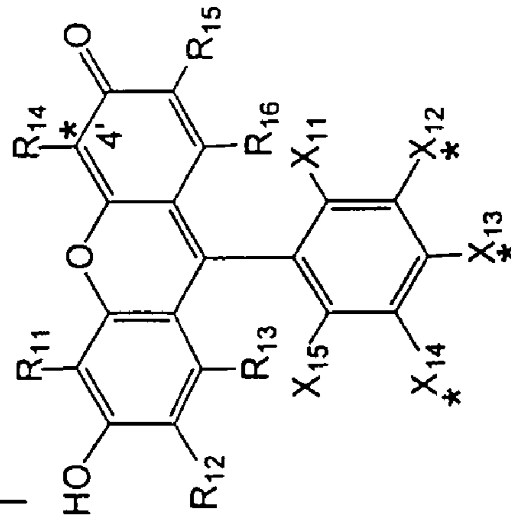
FLUORESCIN
