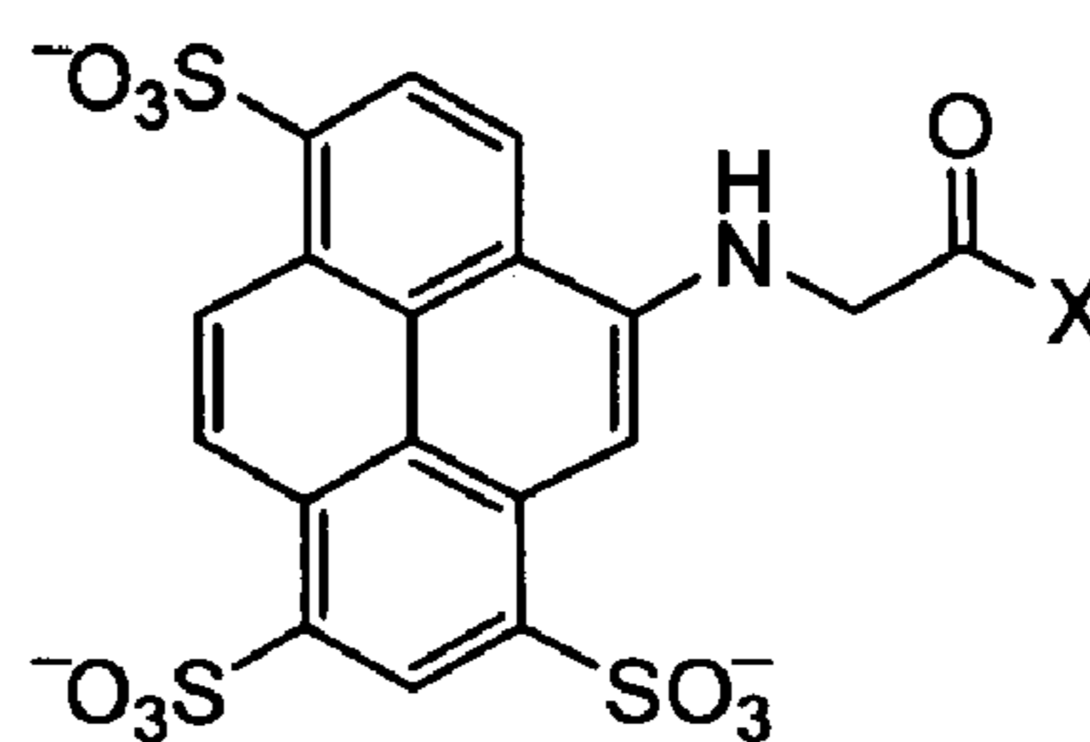
DYE122
