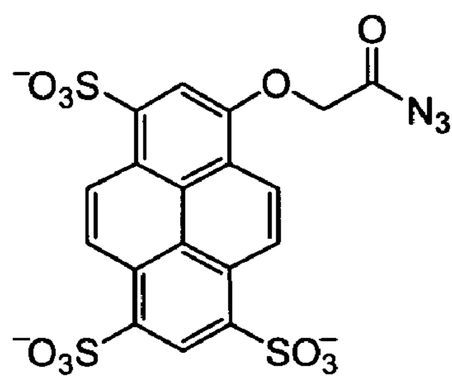
DYE110
