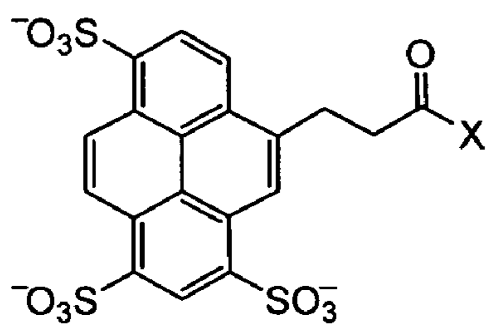
DYE124
