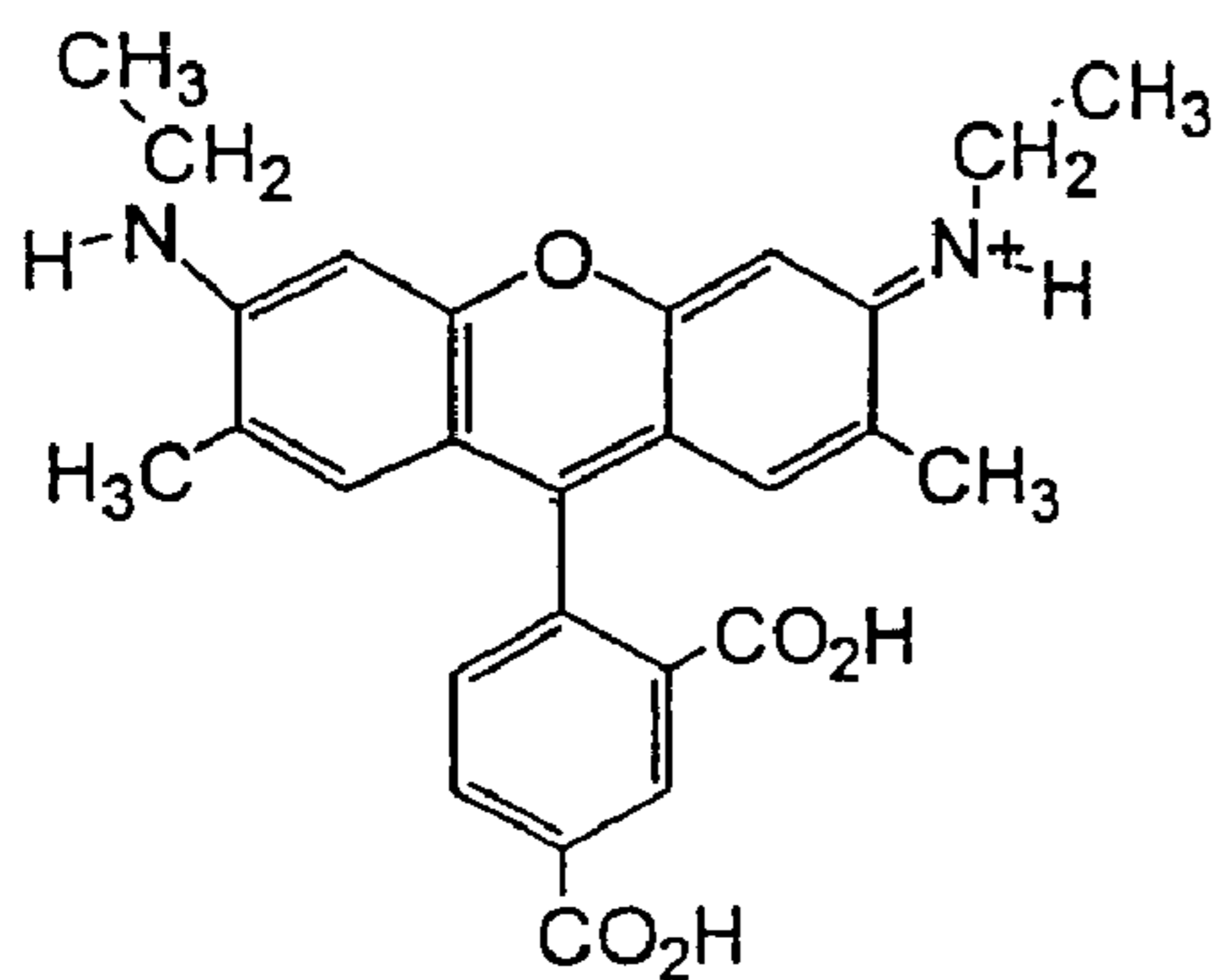
RG6
