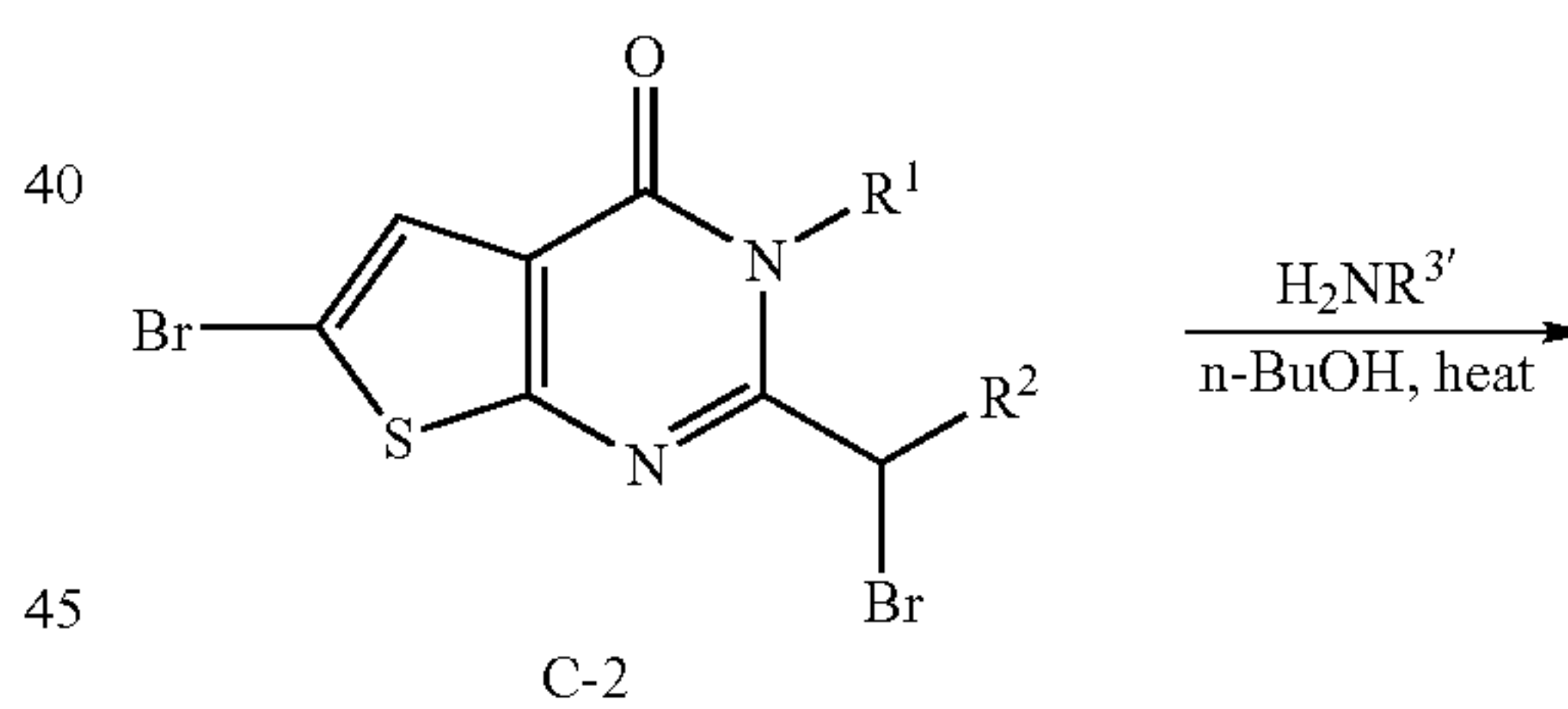
SCHEME D
