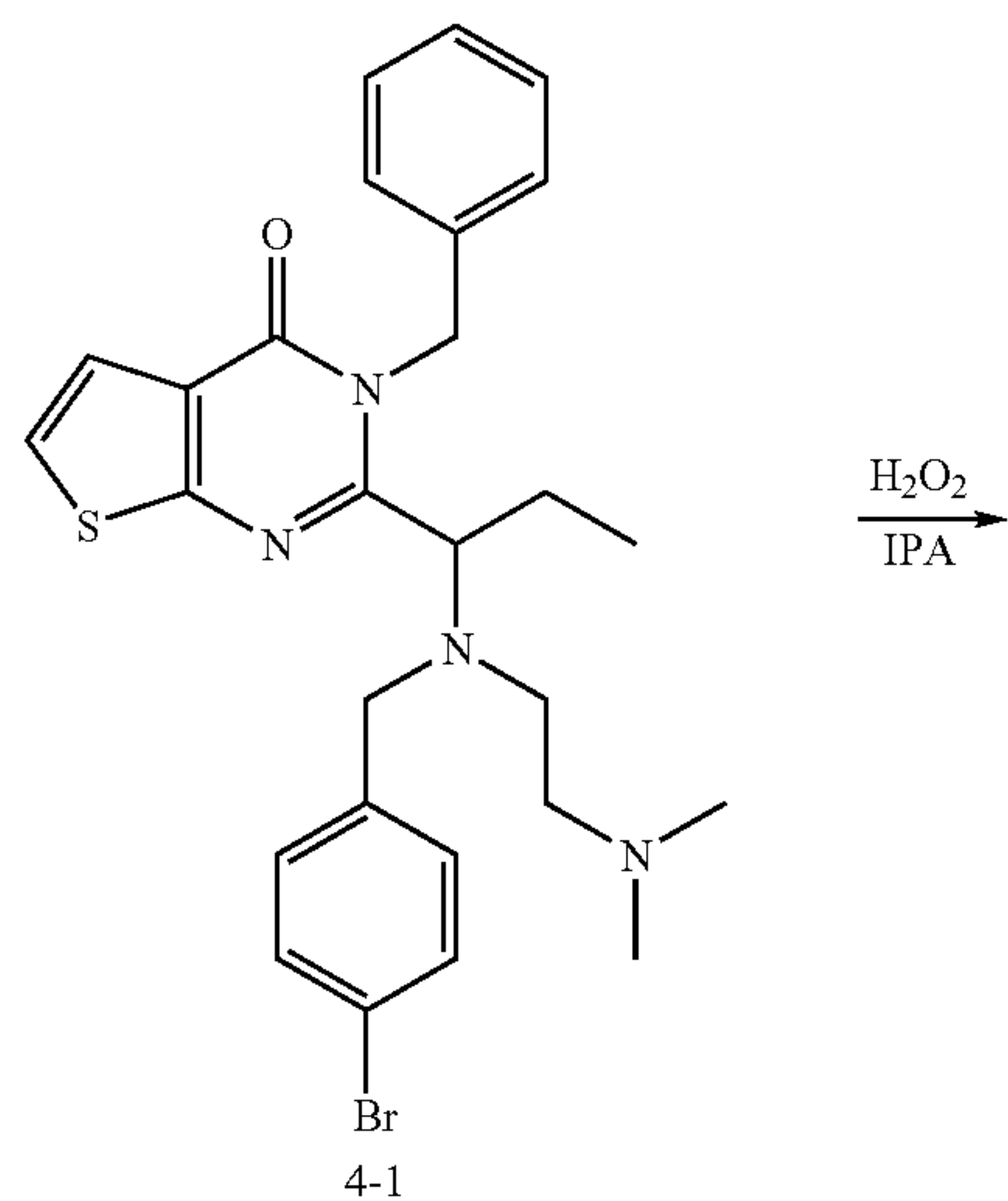
SCHEME 5
