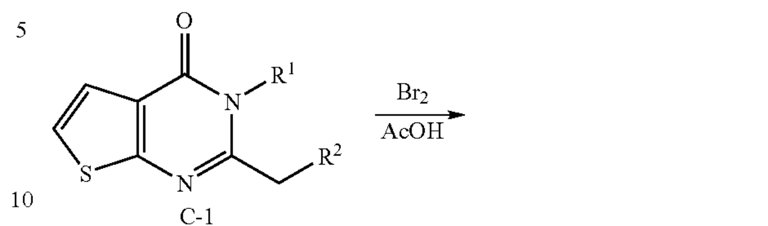
SCHEME C
