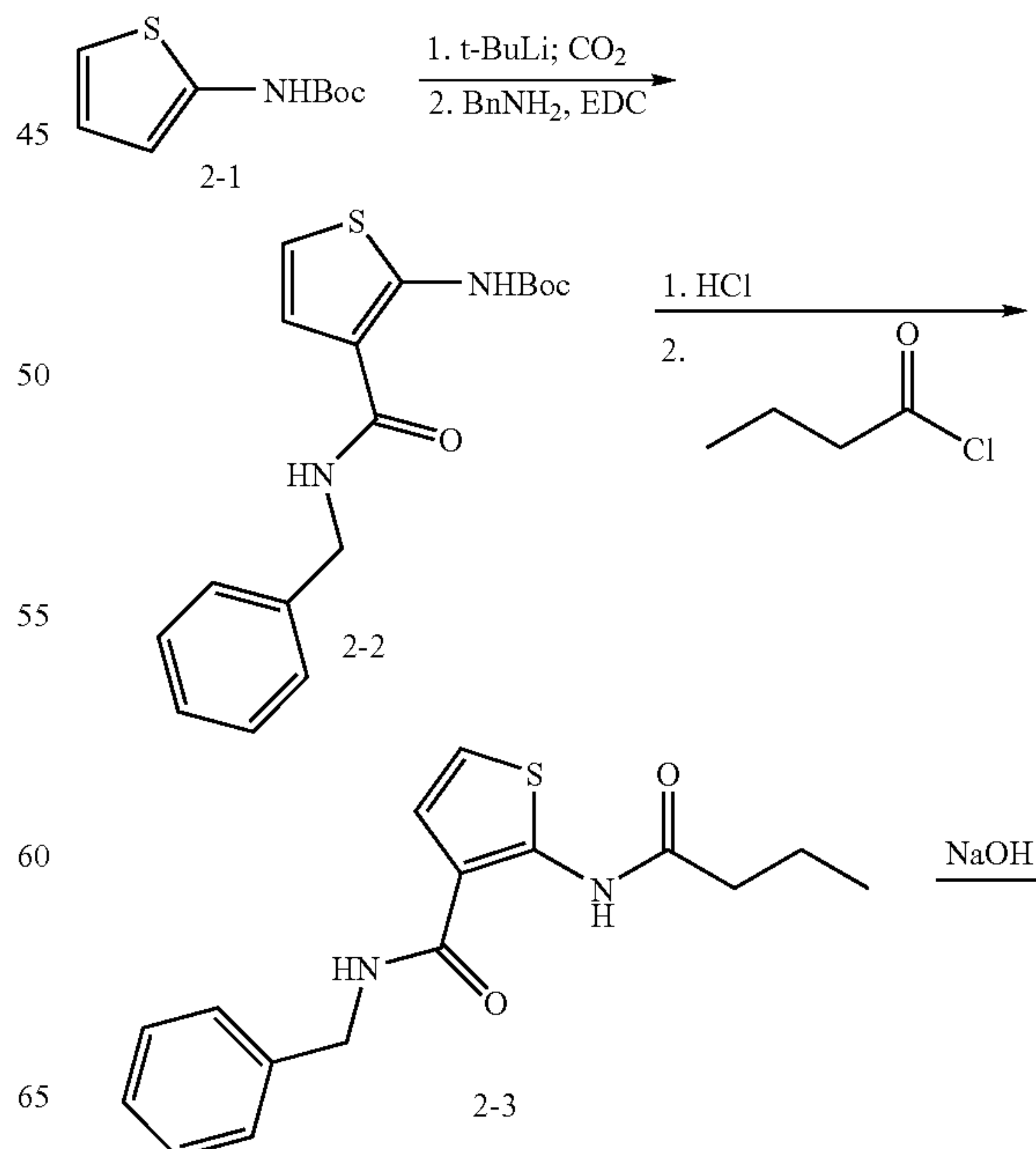
SCHEME 2
