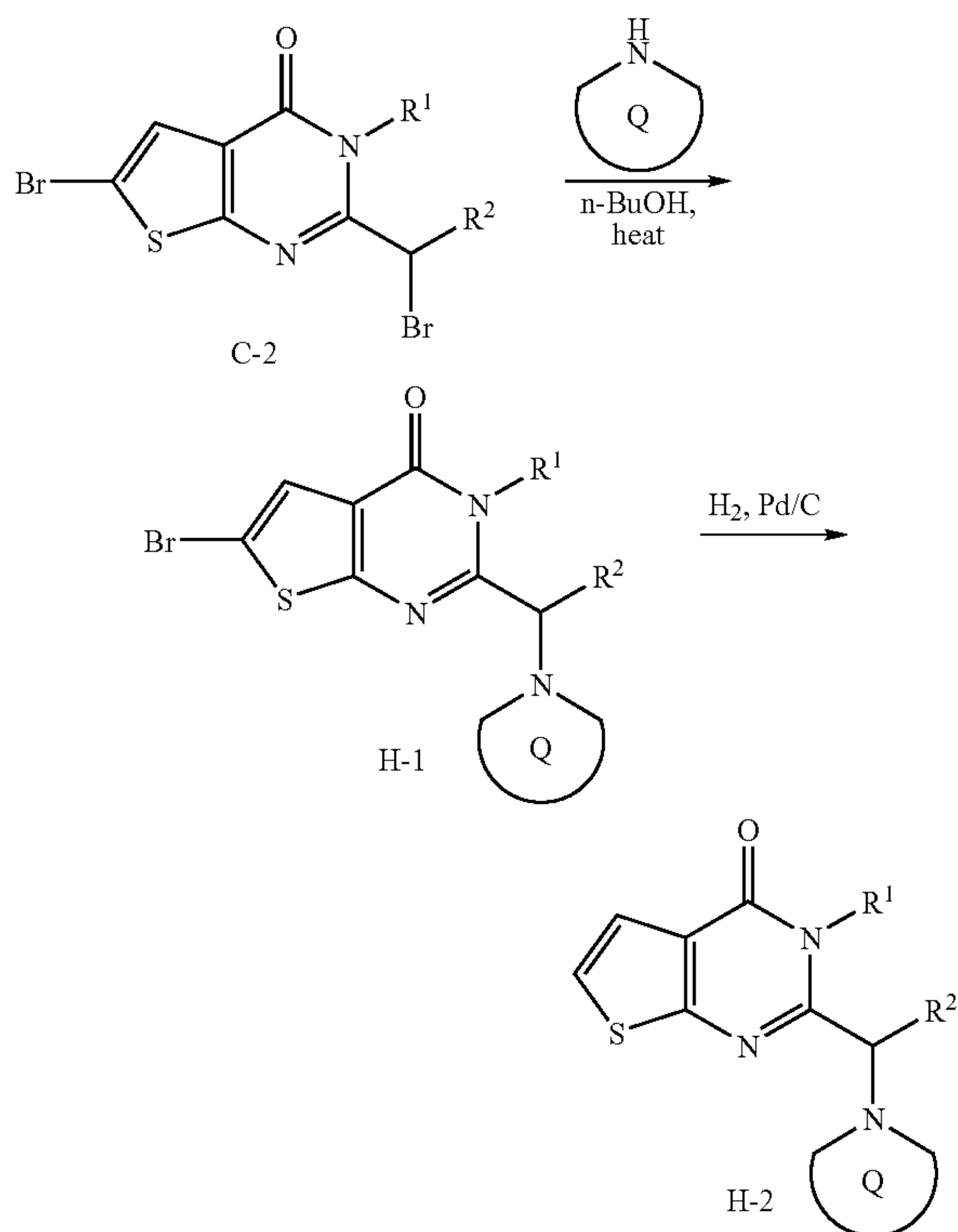
SCHEME H
