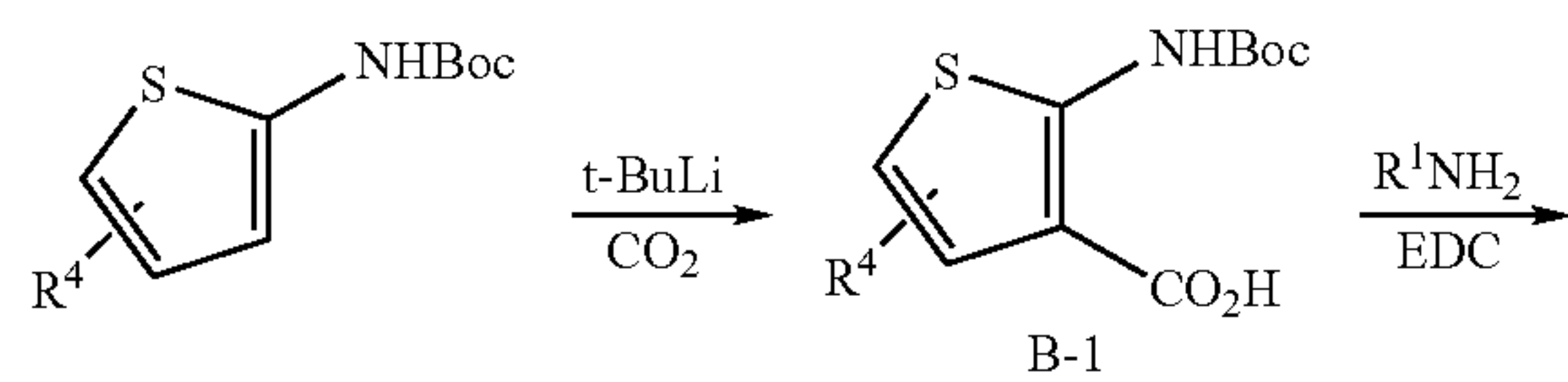
SCHEME B
