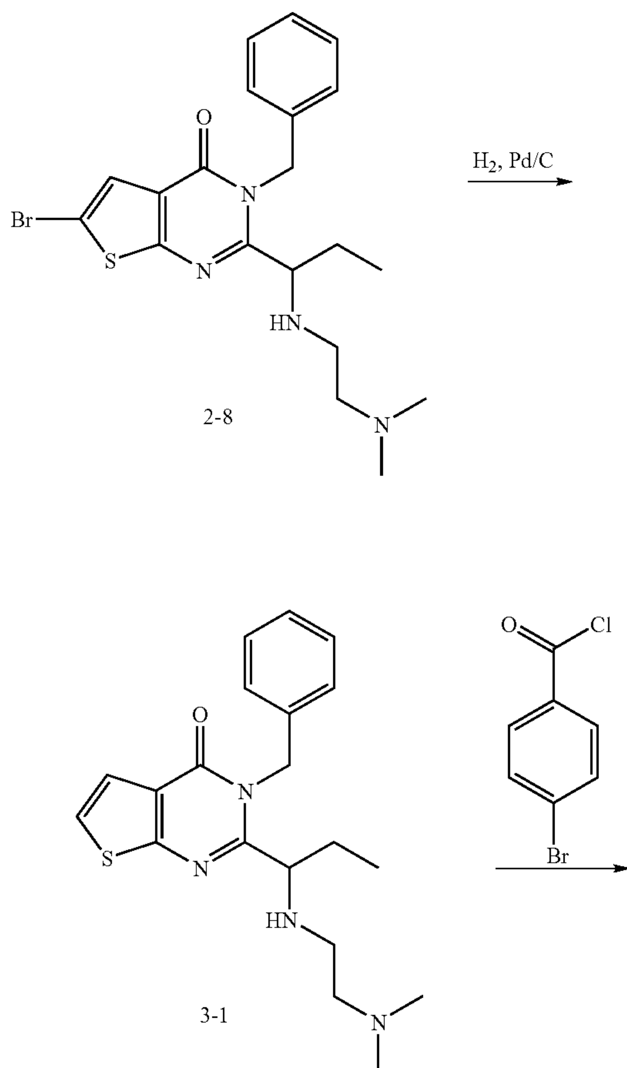
SCHEME 3
