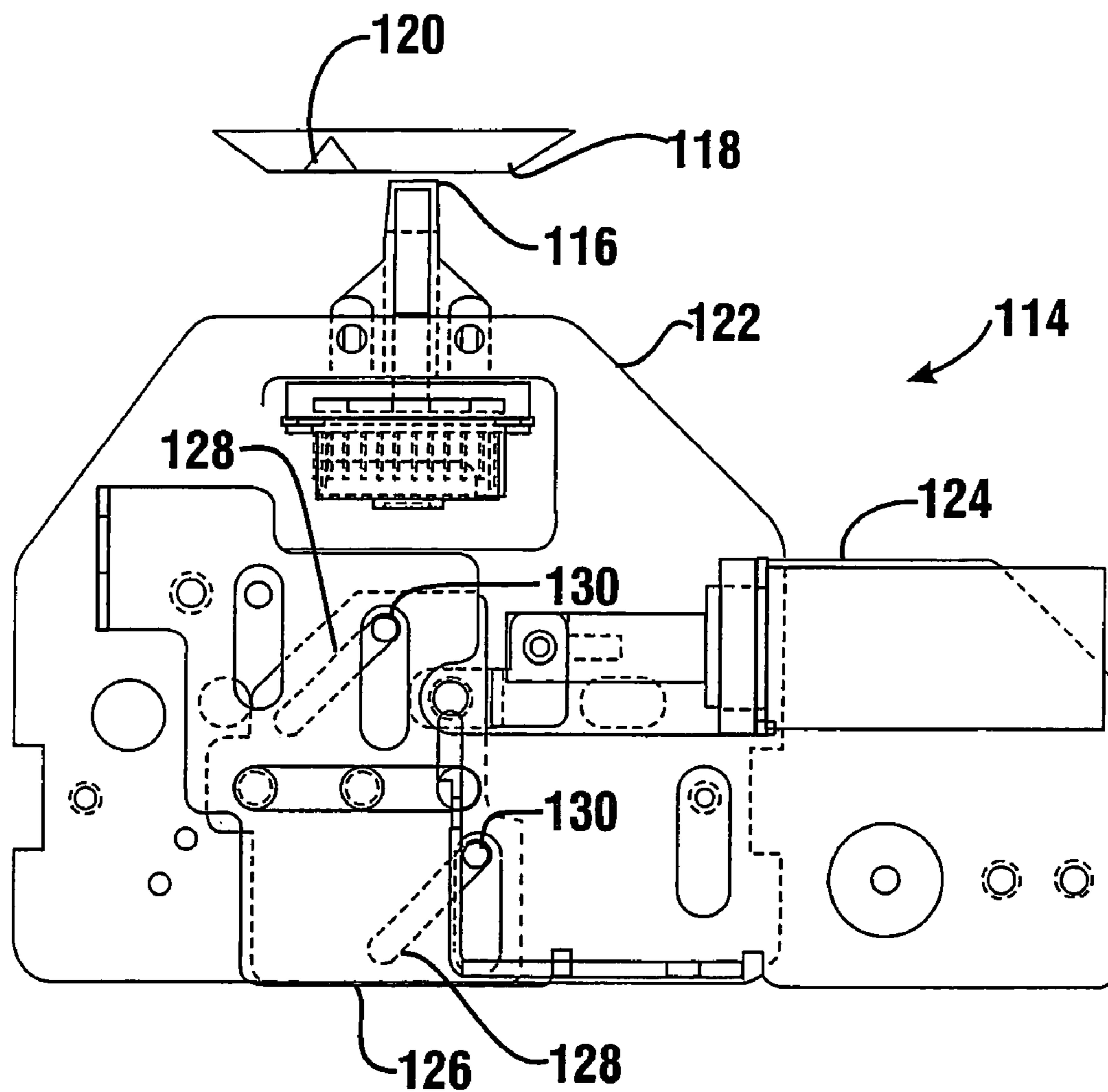
Printing Position
