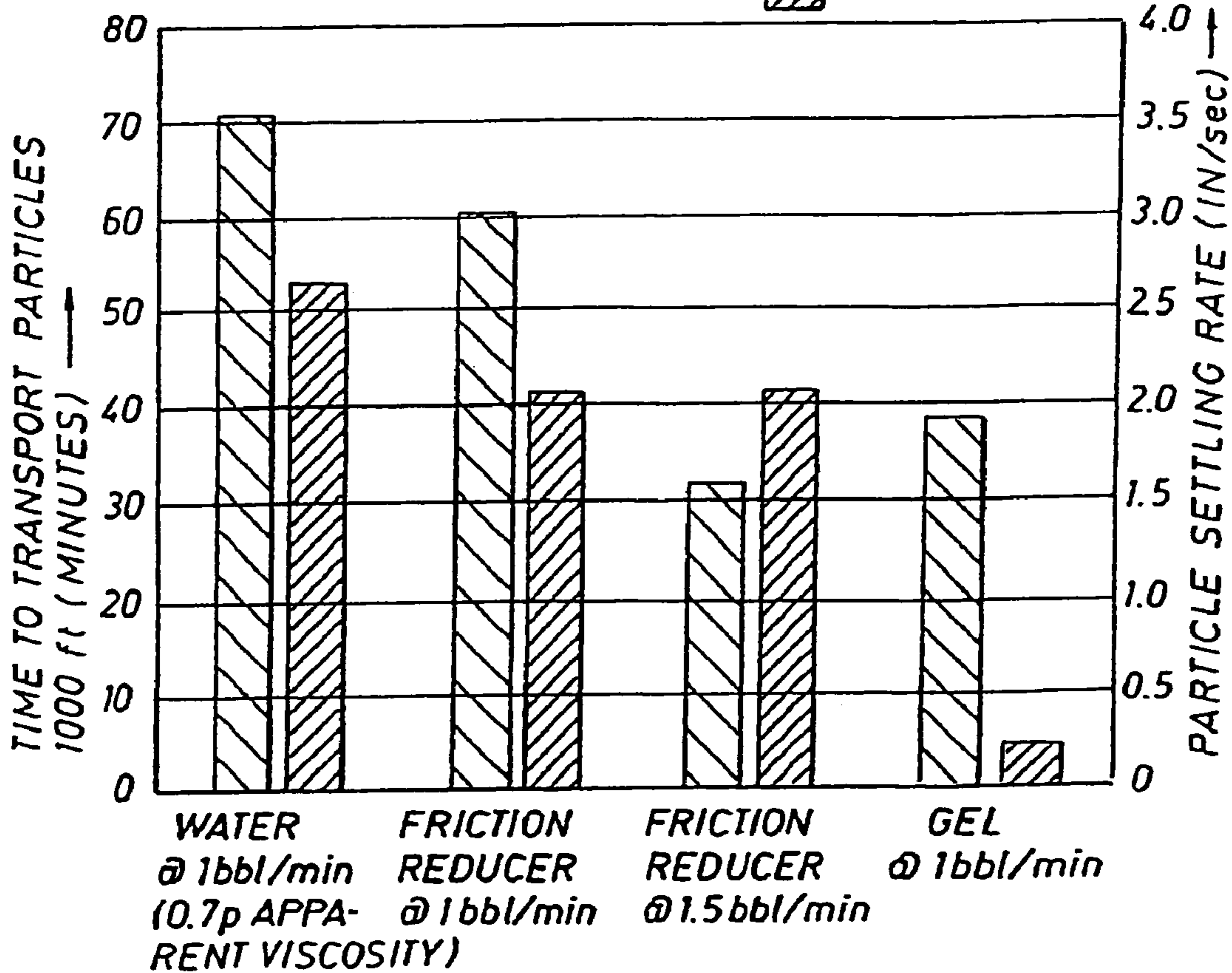
FIG. 5 (Prior Art)
