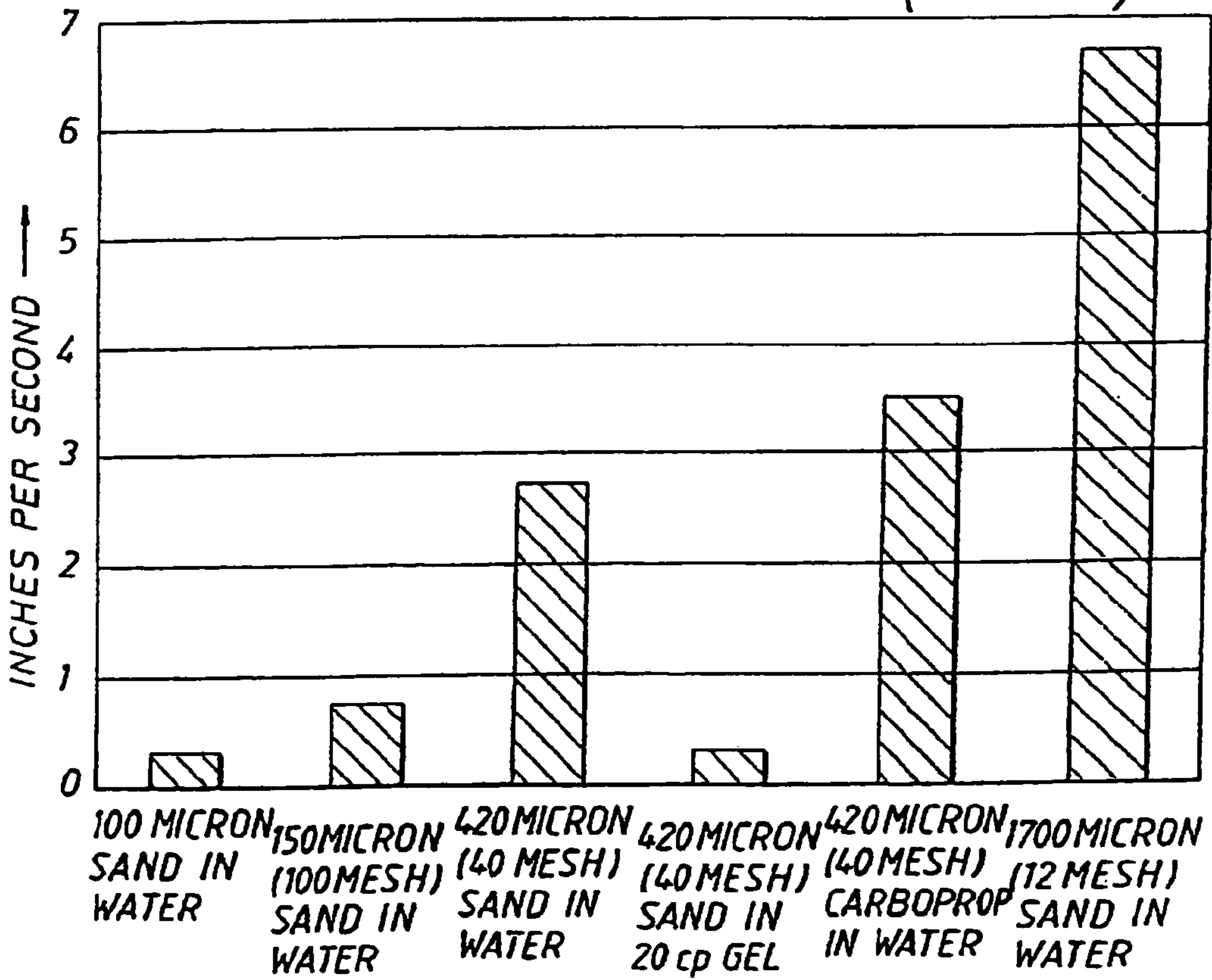
FIG. 8 (Prior Art)
