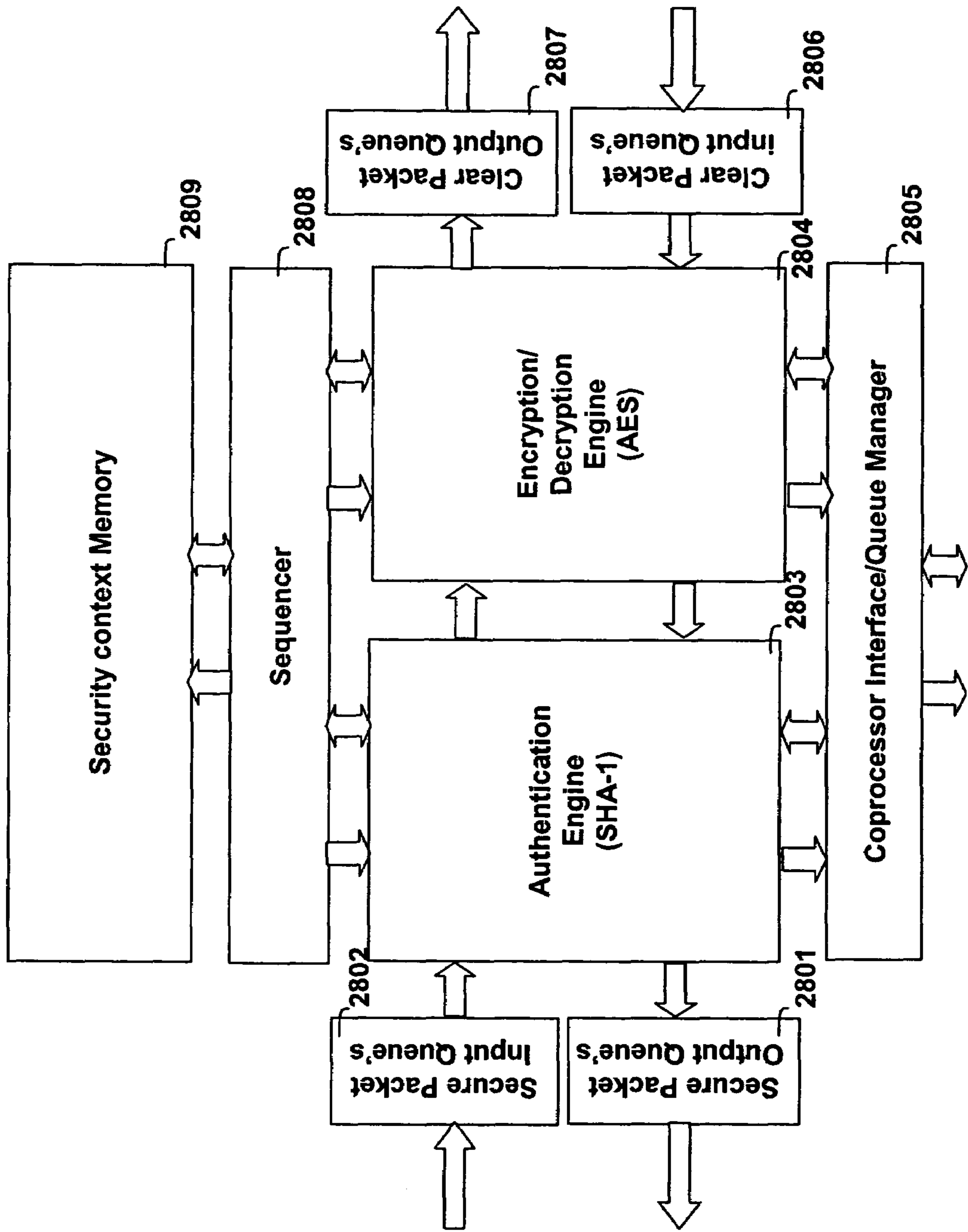
Fig. 28 Security Engine
