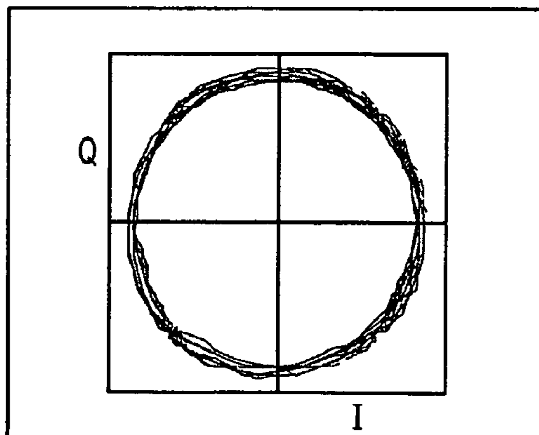
FQPSK-B. VECTOR CONSTELLATION FIG. 19E
