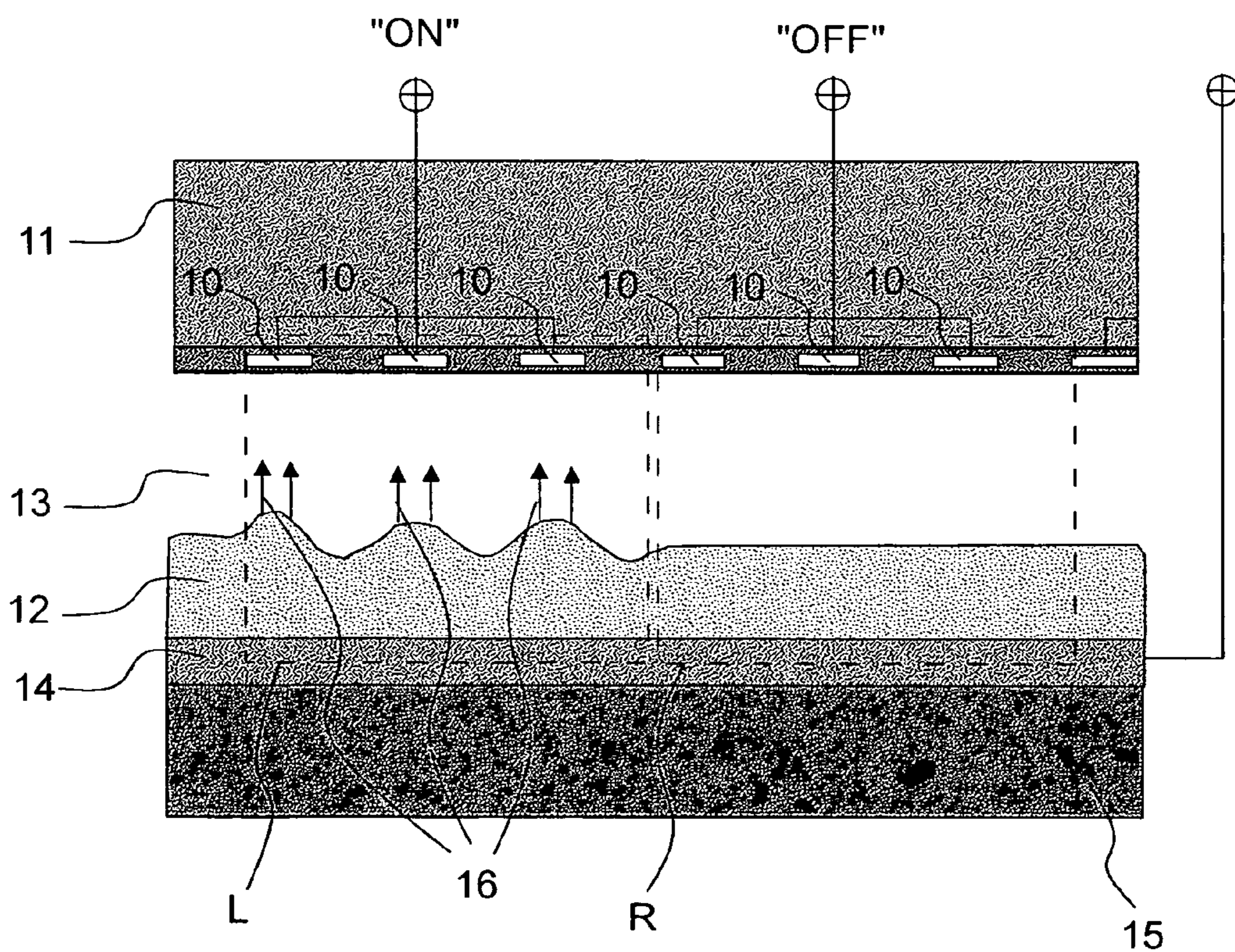
Fig. 2 Prior Art
