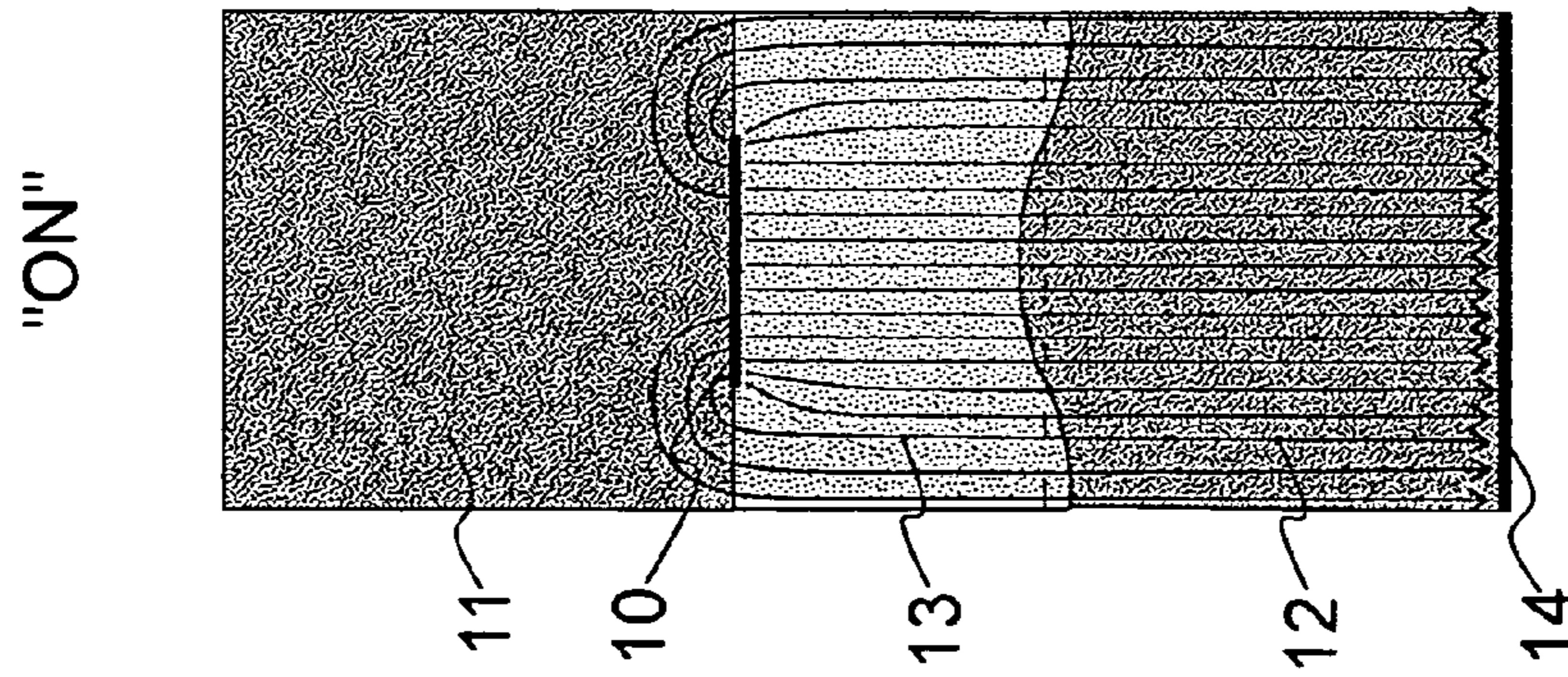
Fig. 3 Prior Art
