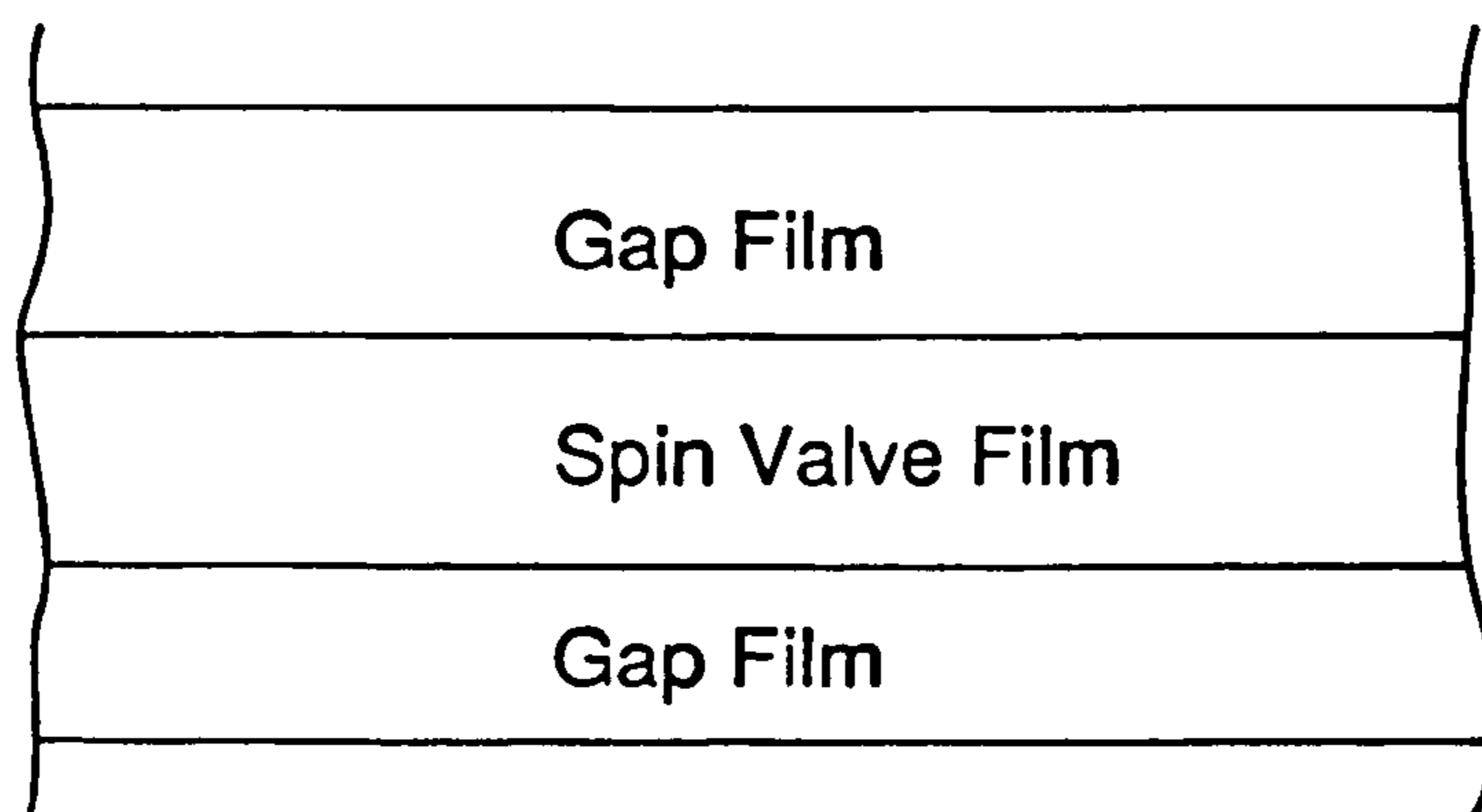
SECTIONAL VIEW OF SPIN VALVE ELEMENT PART
