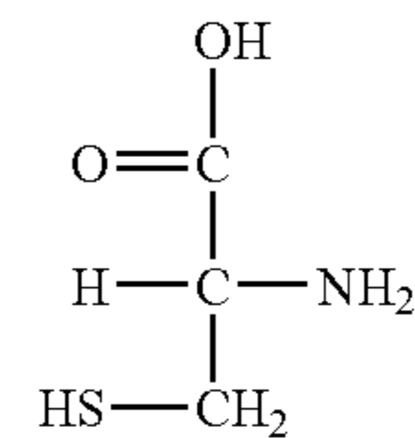
Cysteine
