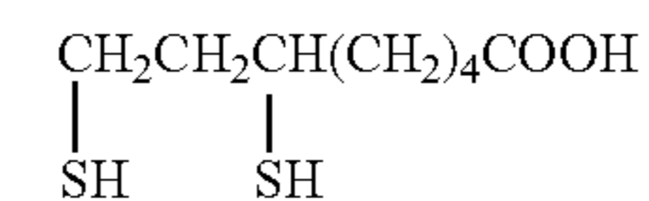
6,8-dimercaptoctanoic acid
