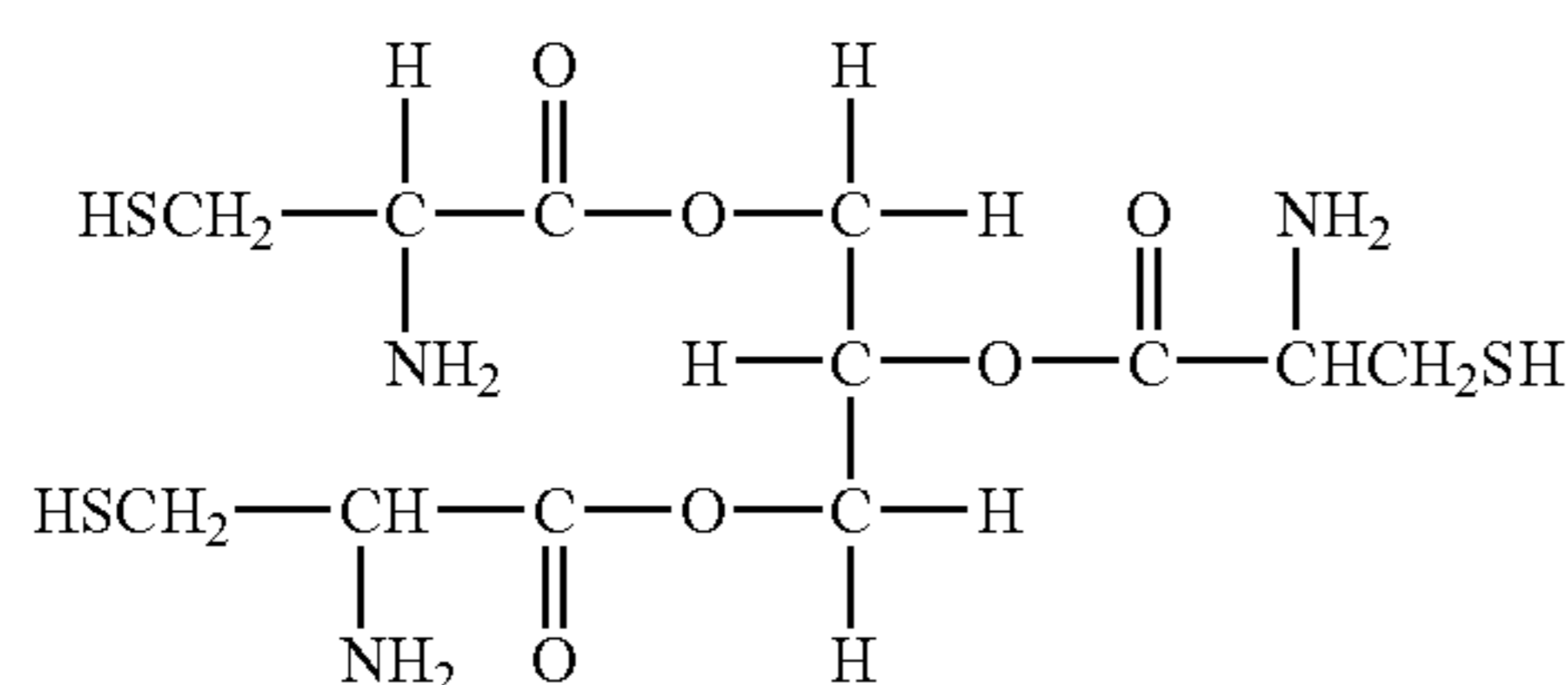
glycerol tricysteinate
