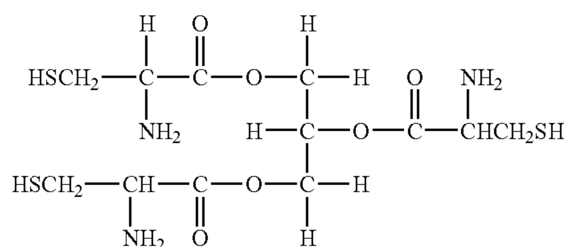
glycerol tricysteinate
