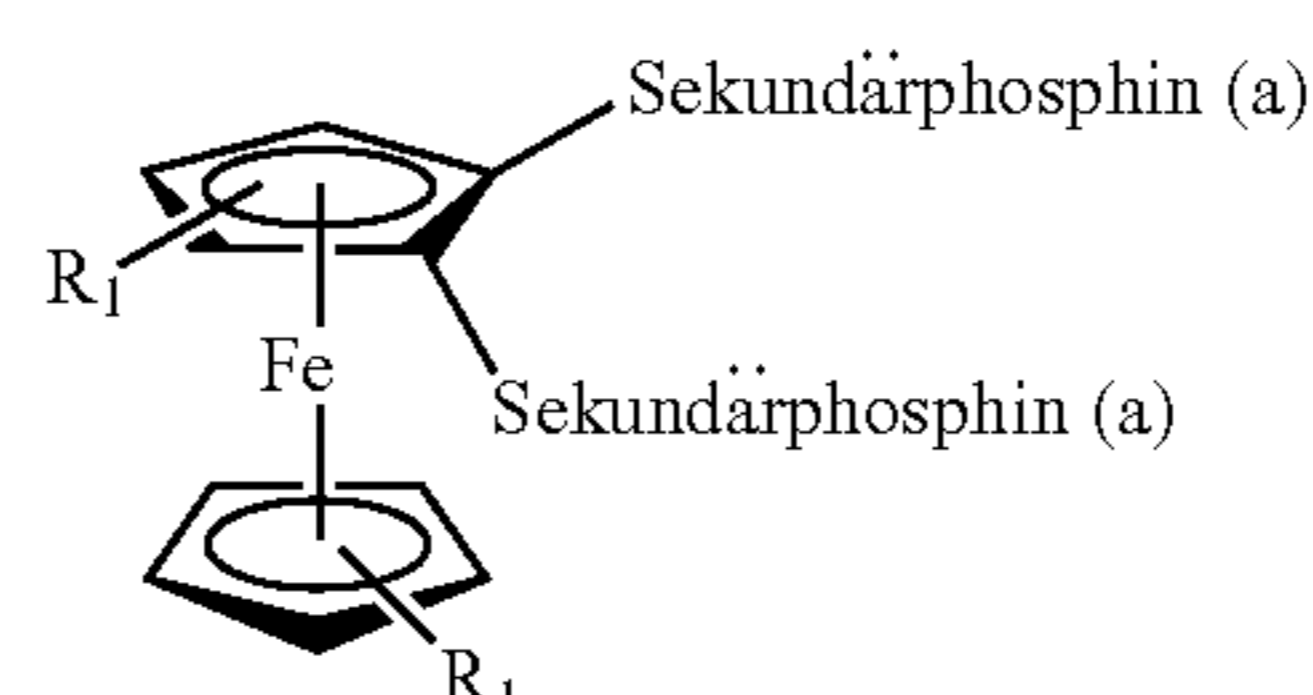
(a) SECONDARY PHOSPHINE.
