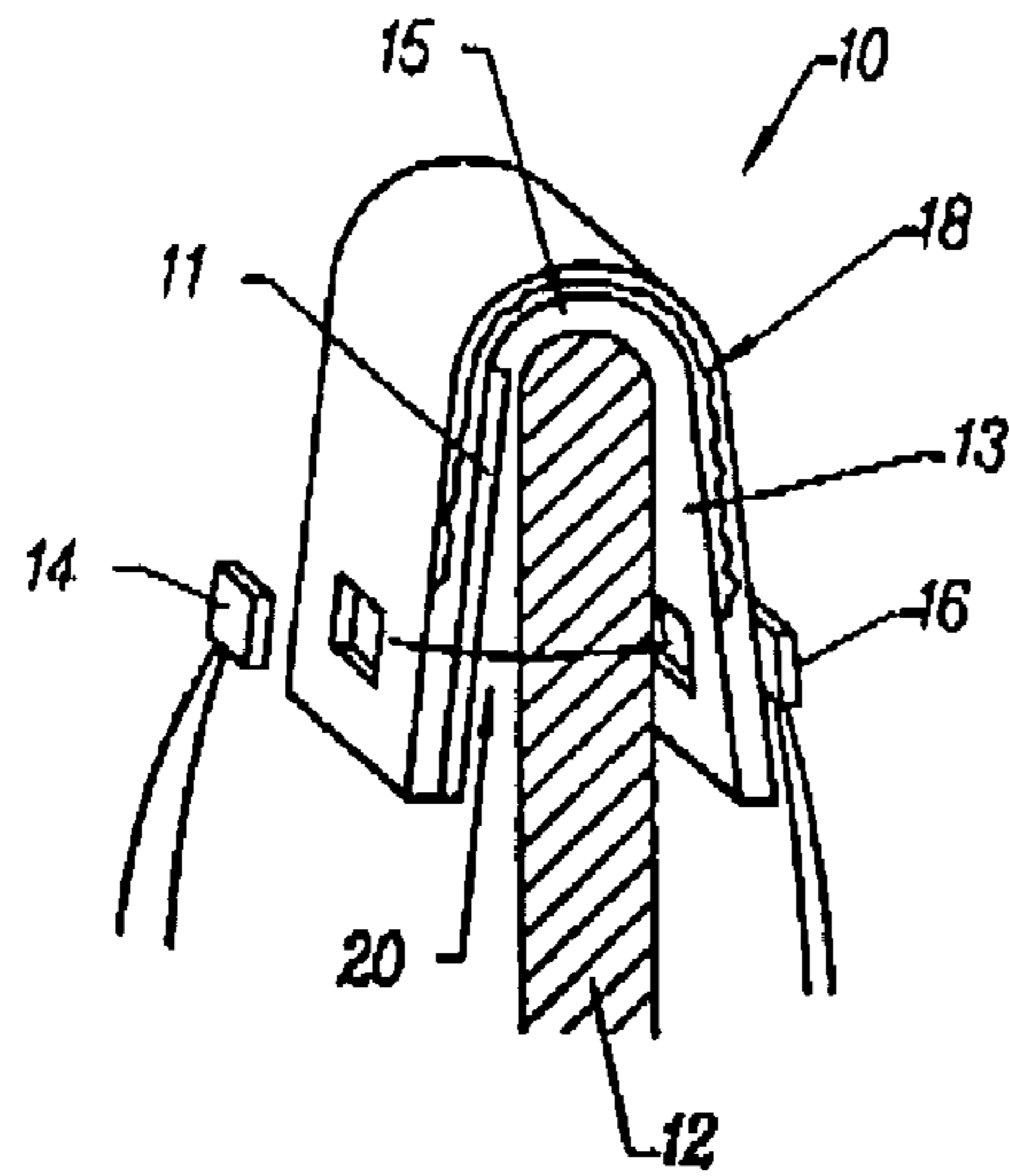
FIG. 1 PRIOR ART
