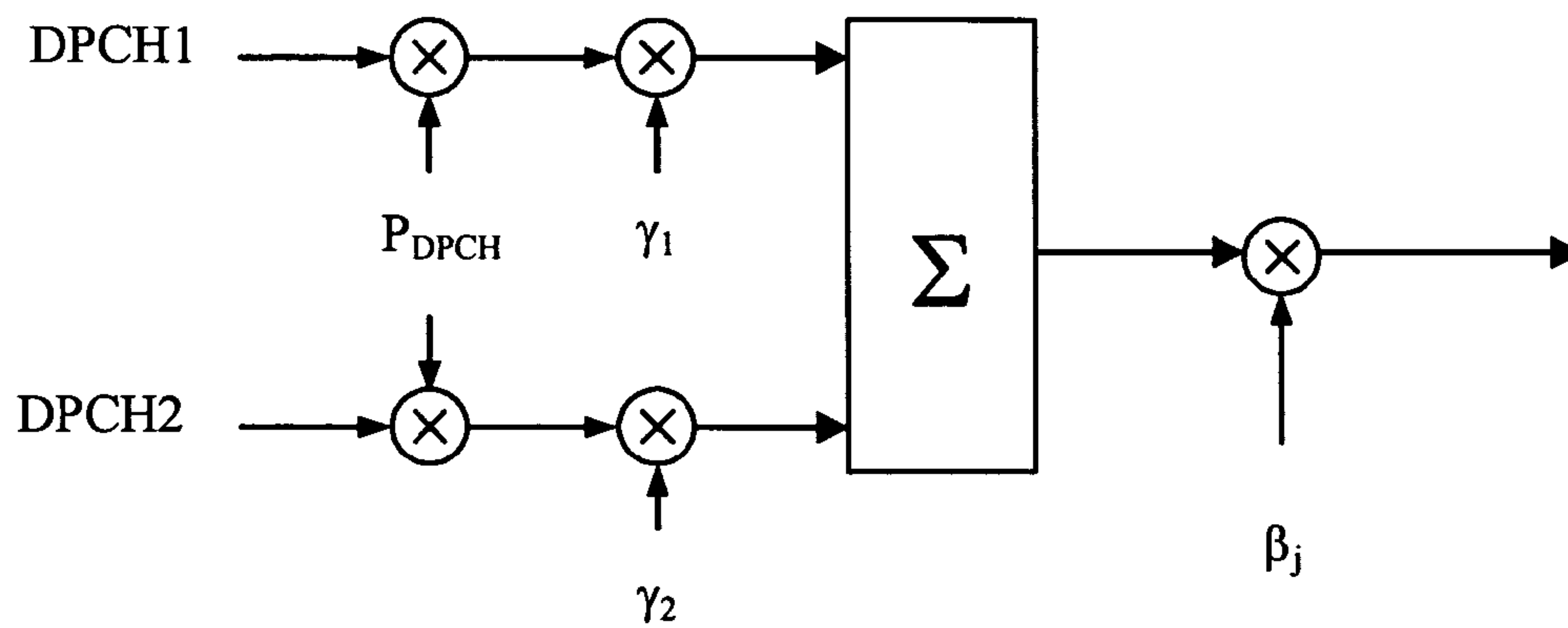
Figure 3 (Prior Art)
