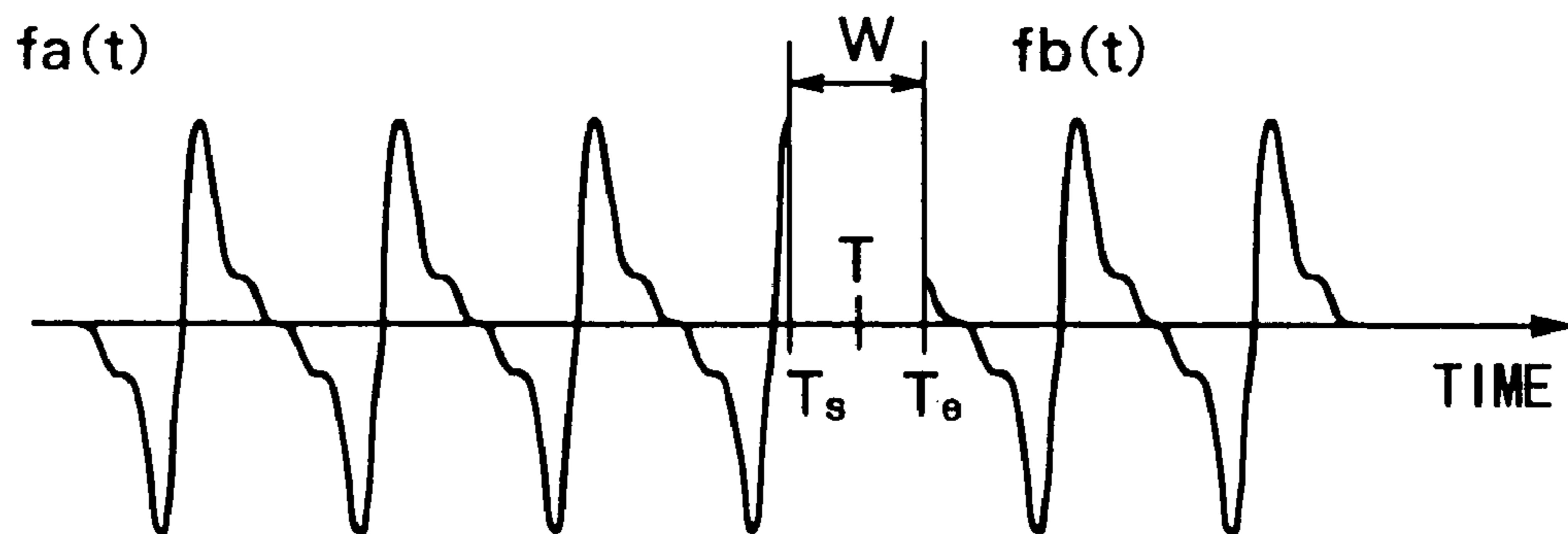
DELETE ANOMALY
