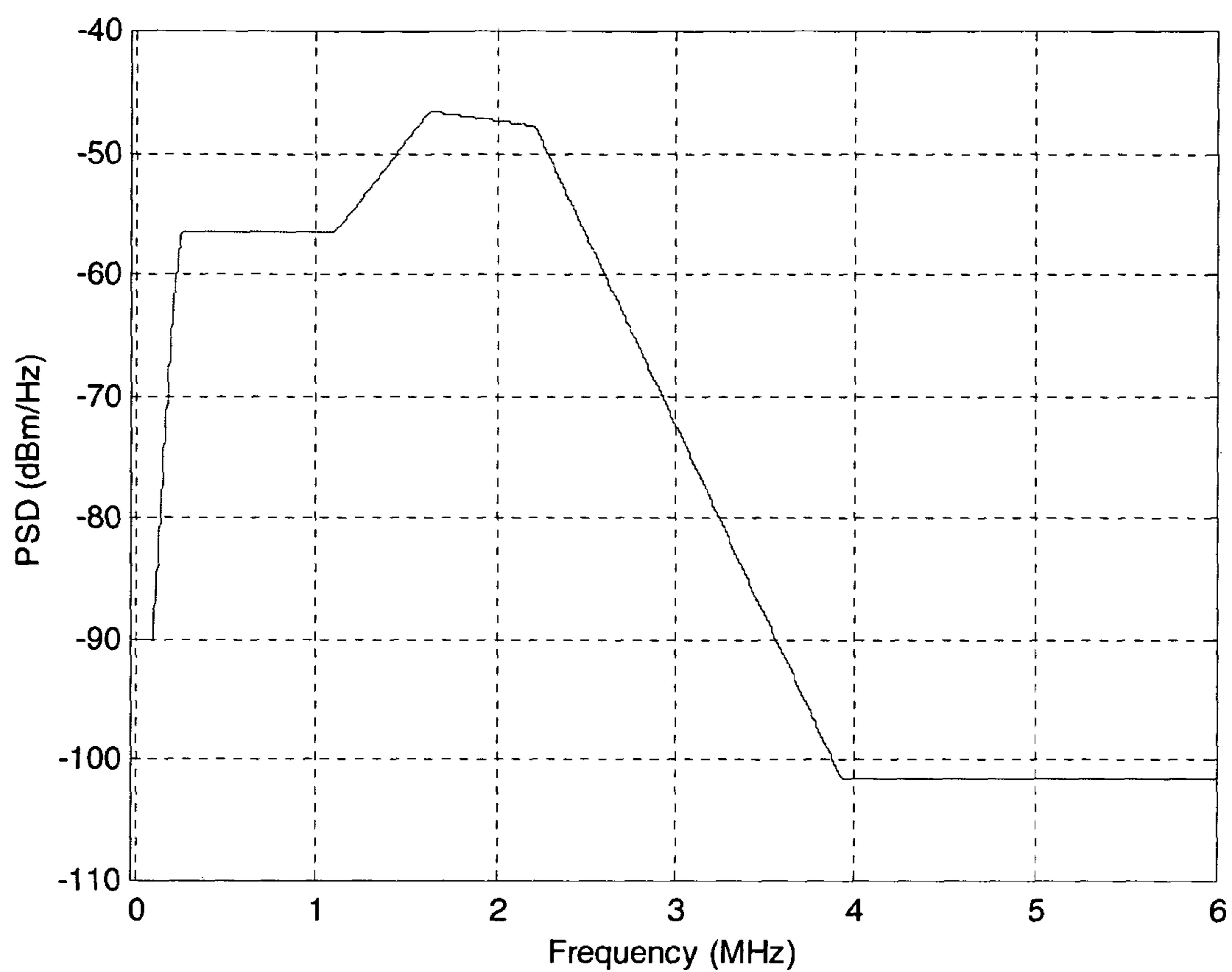
ADSL+ over ISDN PSD for Cabinet Deployment
