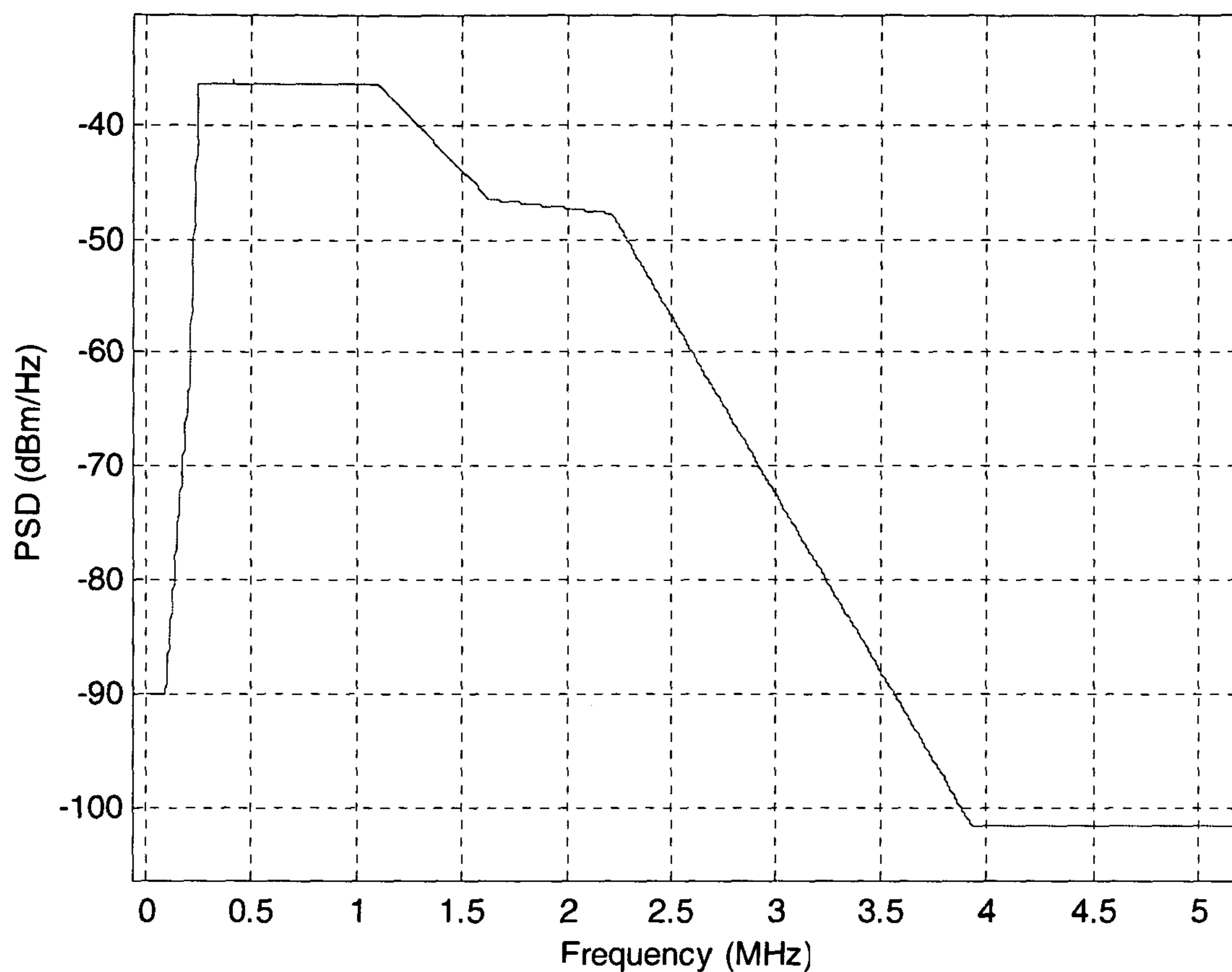
ADSL+ over ISDN PSD for CO Deployment
