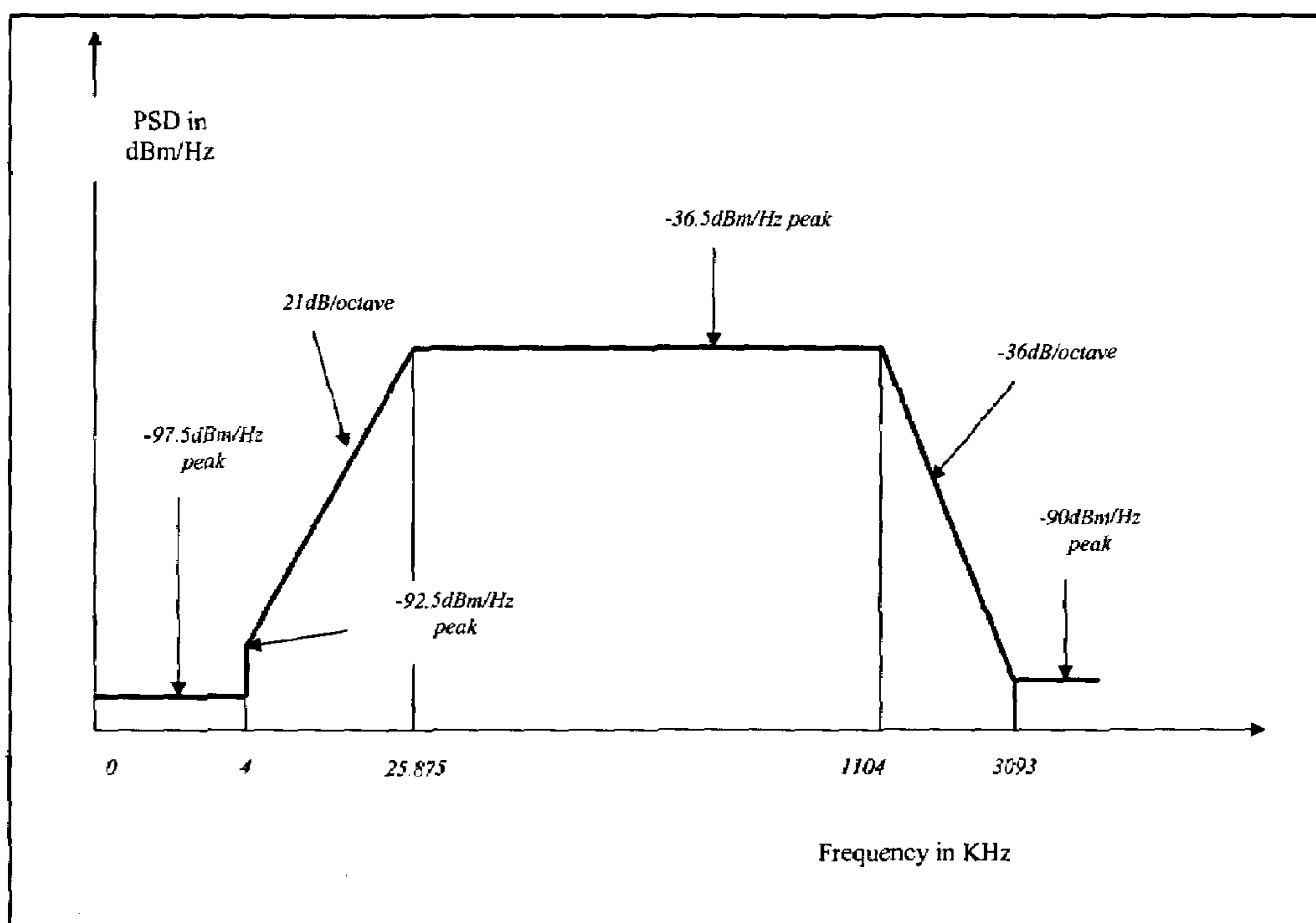
AOL Downstream Spectral Mask
