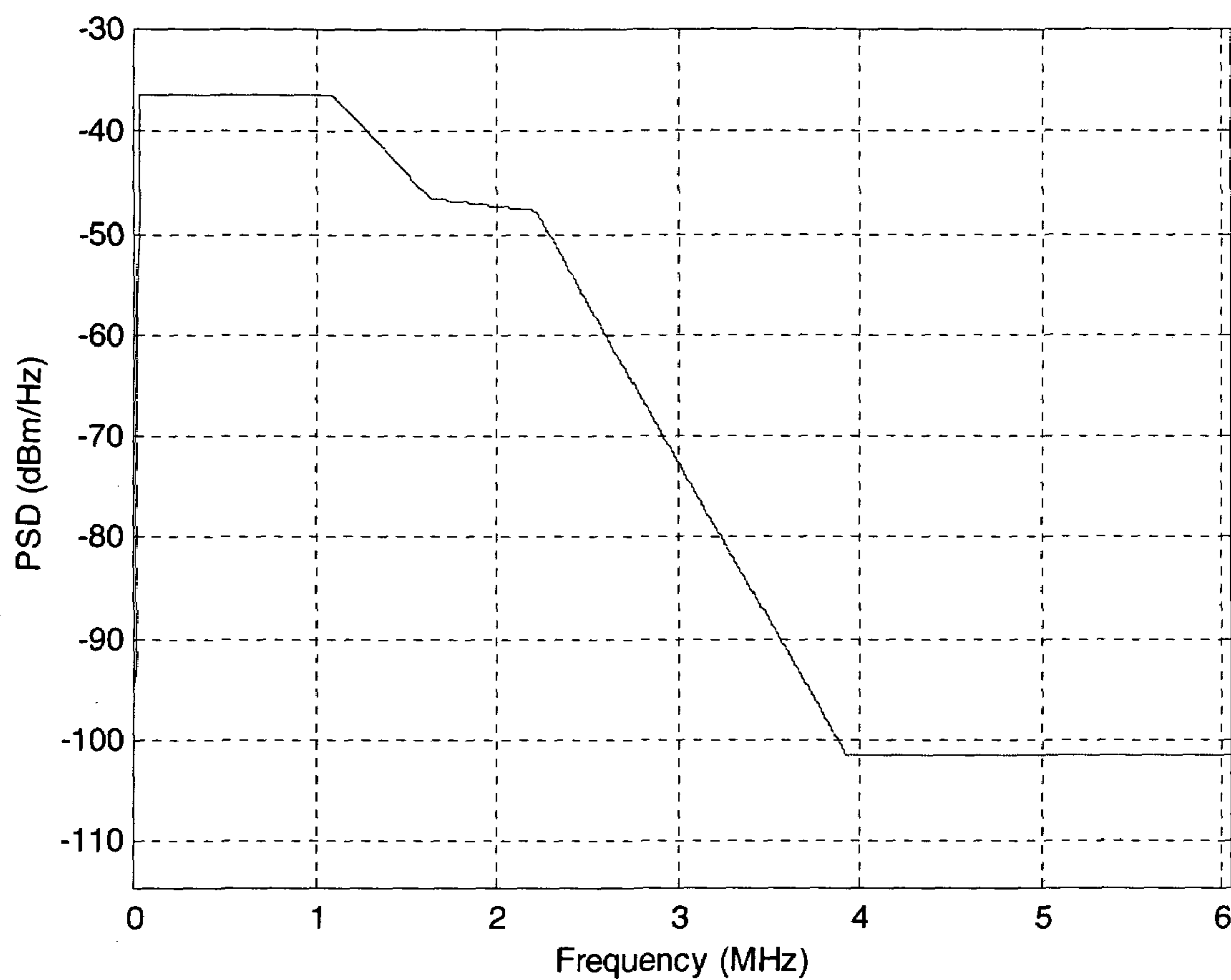
ADSL+ PSD for CO Deployment
