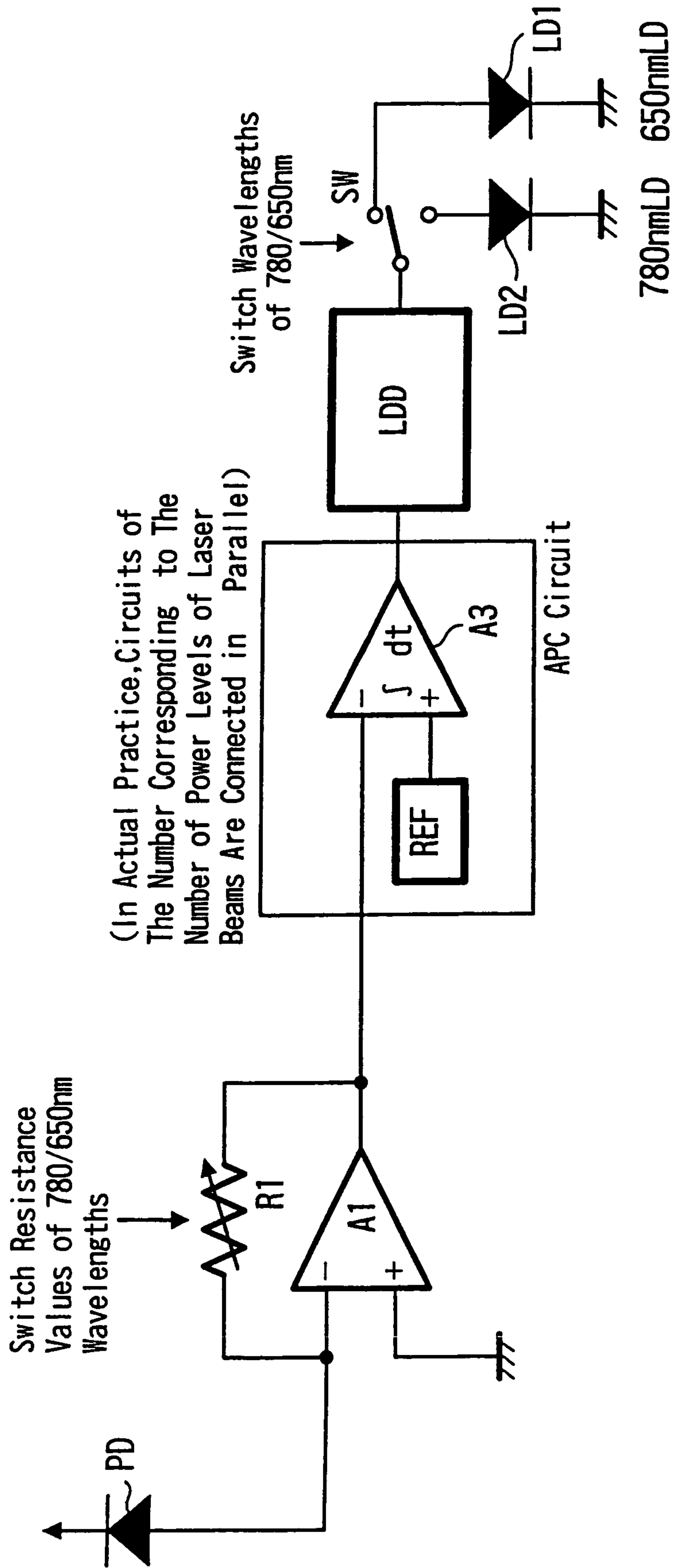
FIG. 1 (RELATED ART)
