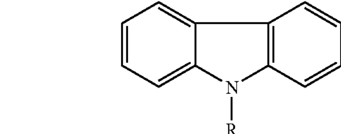
(R denotes hydrogen atom or alkyl group)
