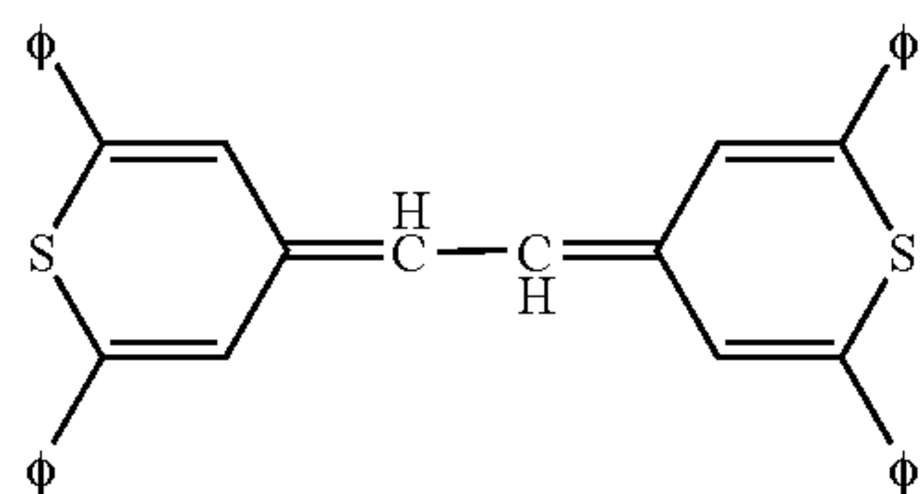
( \phi denotes phenyl group)
