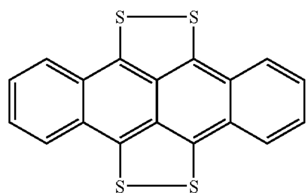
tetrathiotetracene (TTT)
