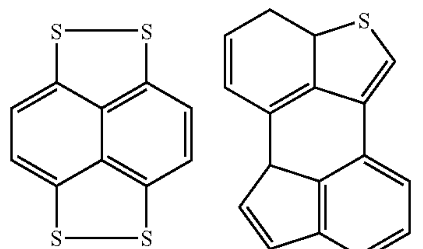
tetrathionaphthalene benzothiophene (BBT)
