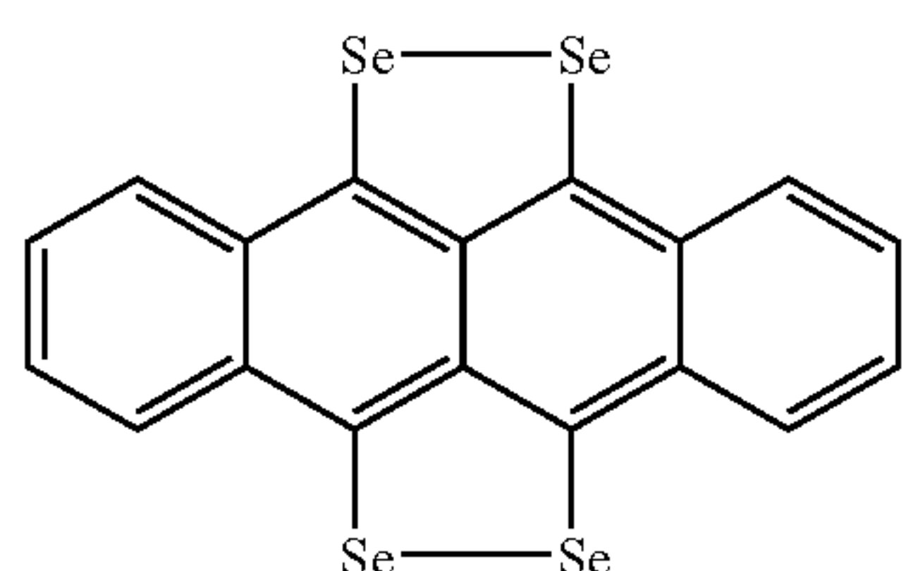
tetraselenatetracene (TST)
