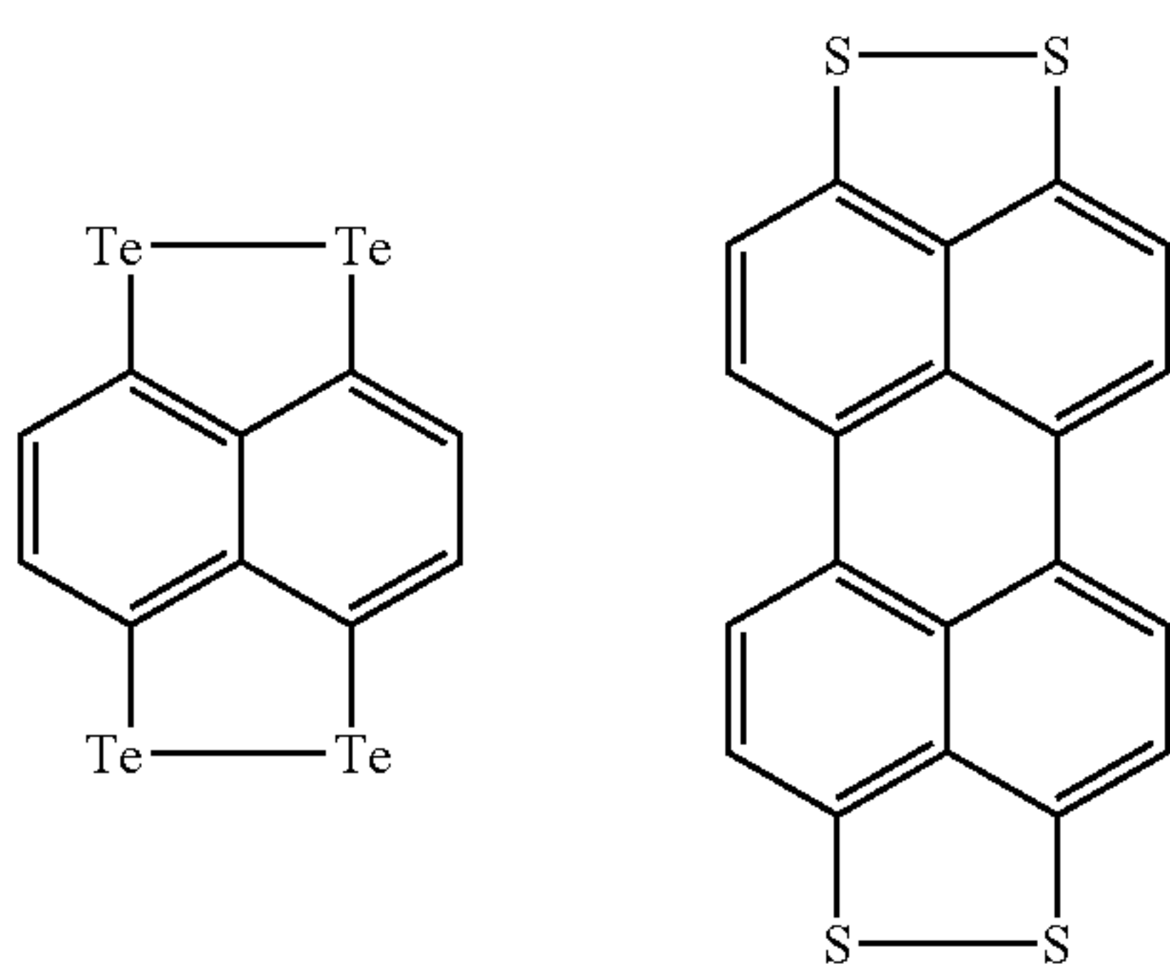
tetrathioerylene
