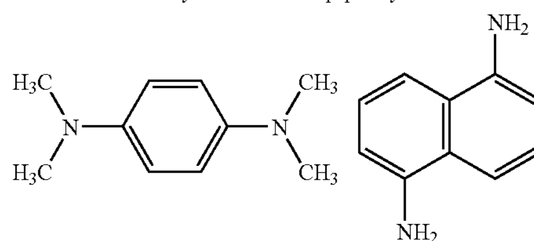
aniline N-methylaniline p-phenylenediamine
