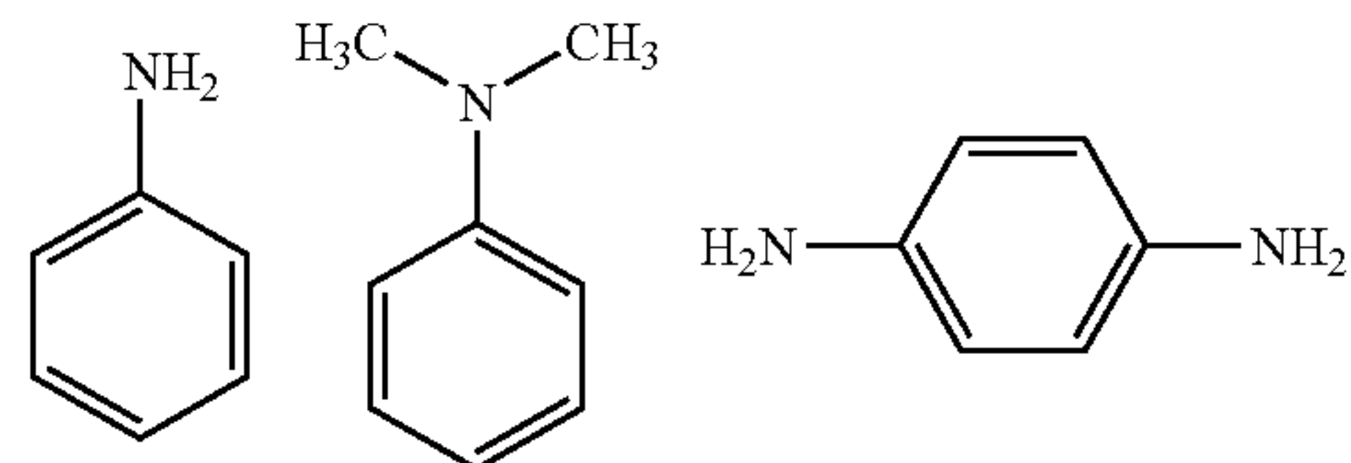
aniline N-methylaniline p-phenylenediamine
