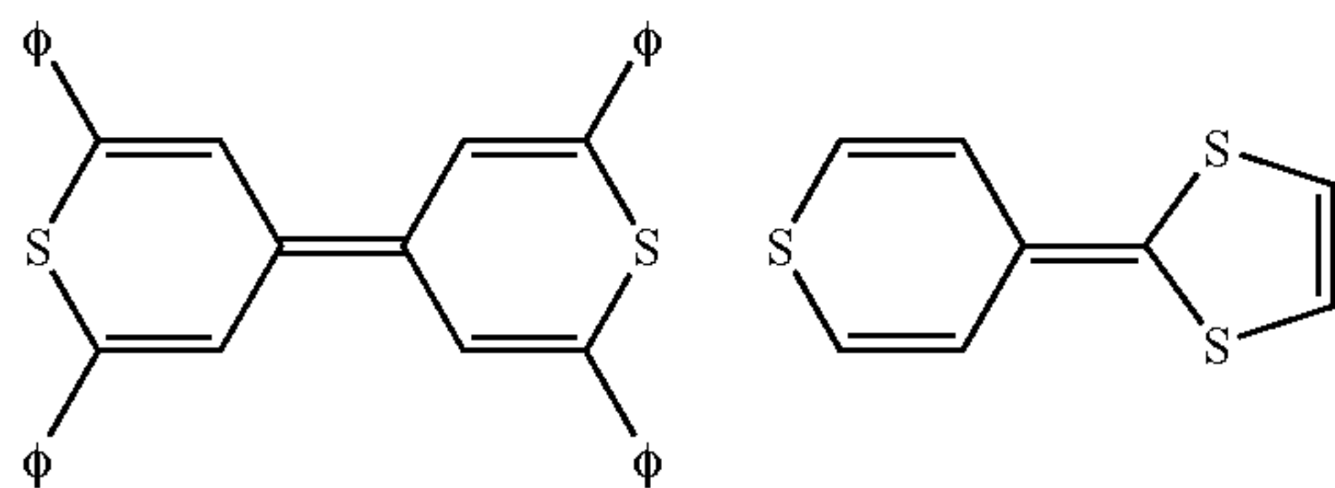
tetraphenylbithiopyranylidene (BTP)
