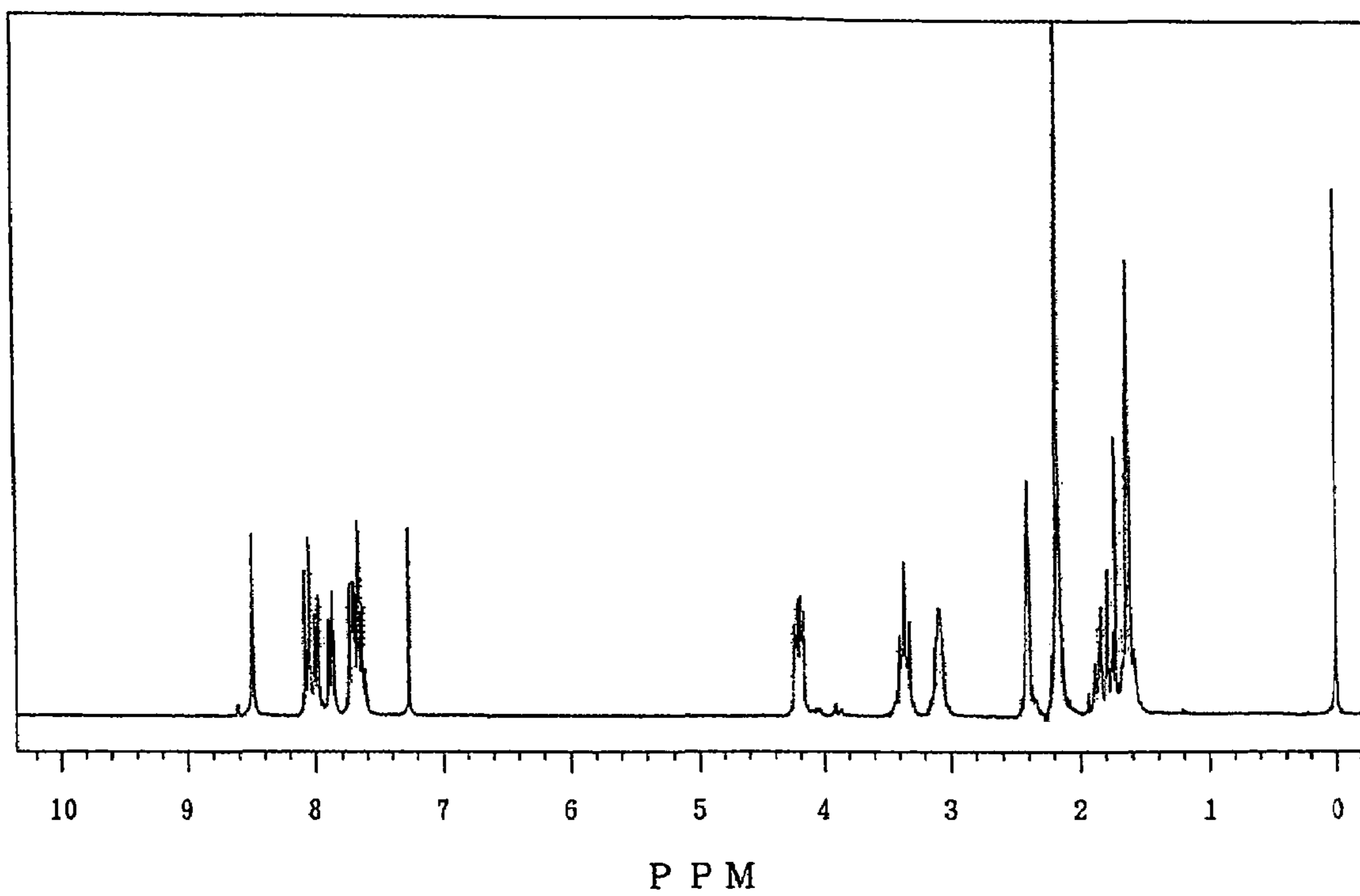
^1\text{H} -NMR spectrometry spectrum of the sulfonium salt (A-4)
