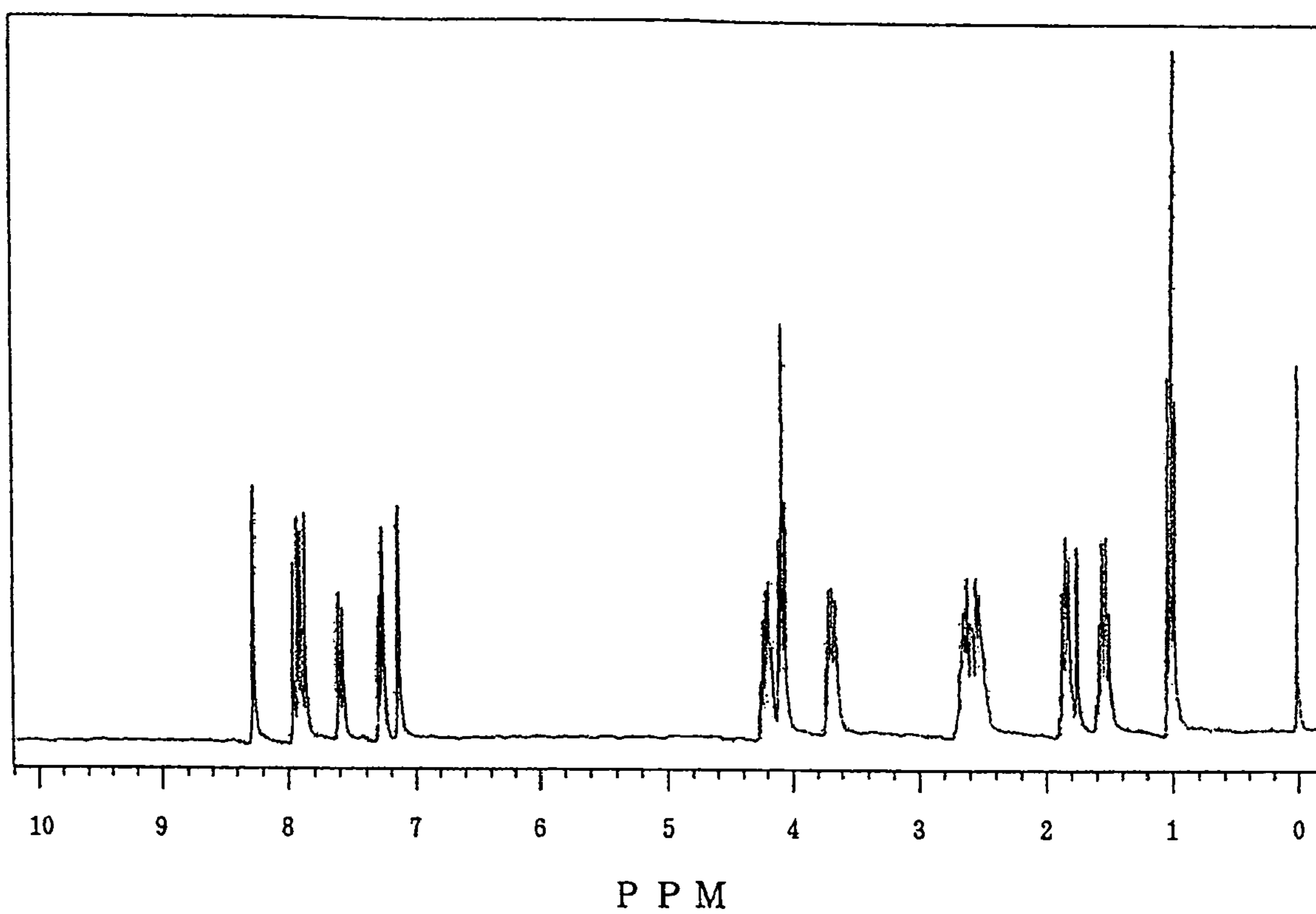
^1\text{H-NMR} spectrometry spectrum of the sulfonium salt (A-5)
