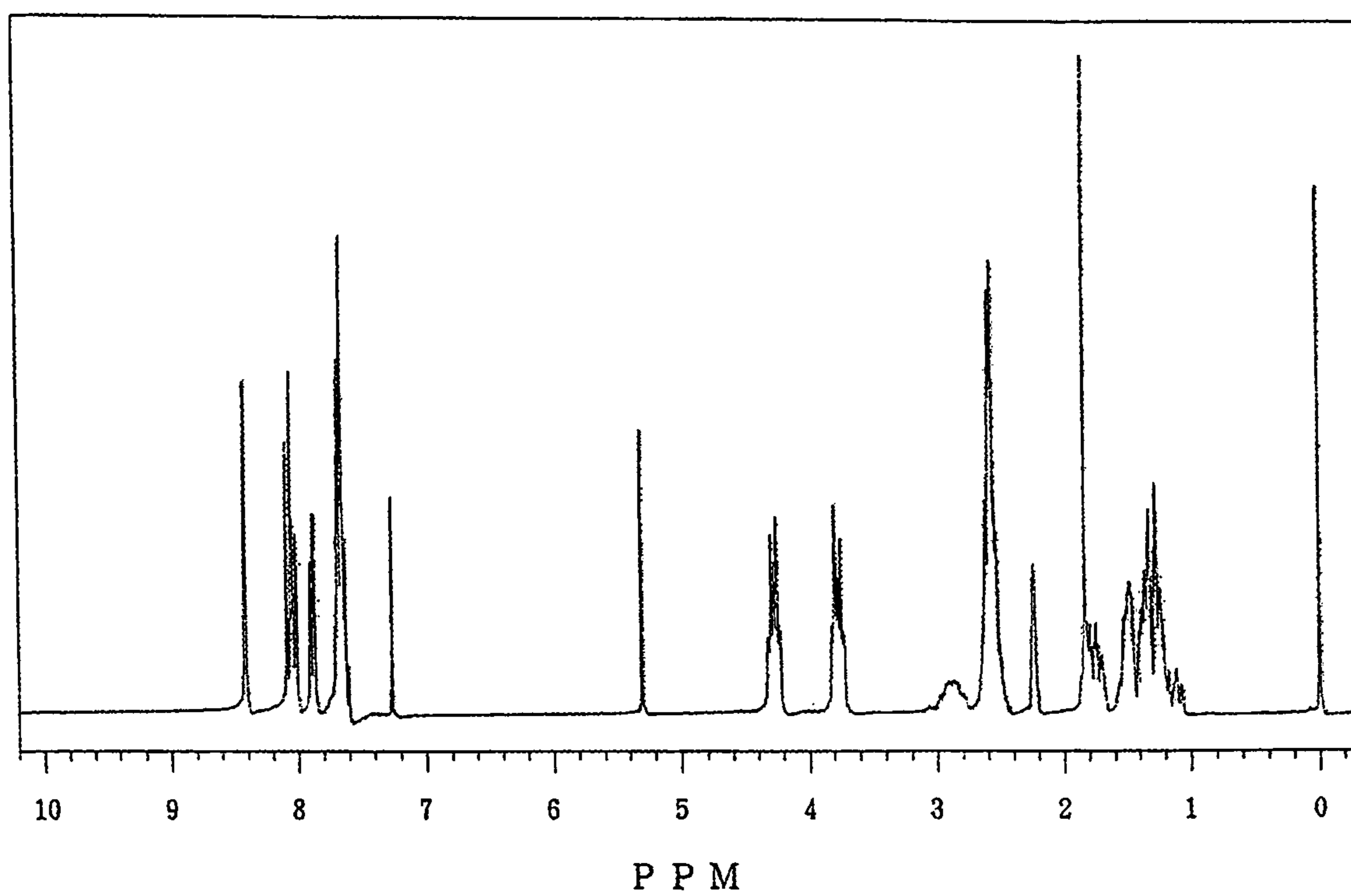
1 H-NMR spectrometry spectrum of the sulfonium salt (A-2)
