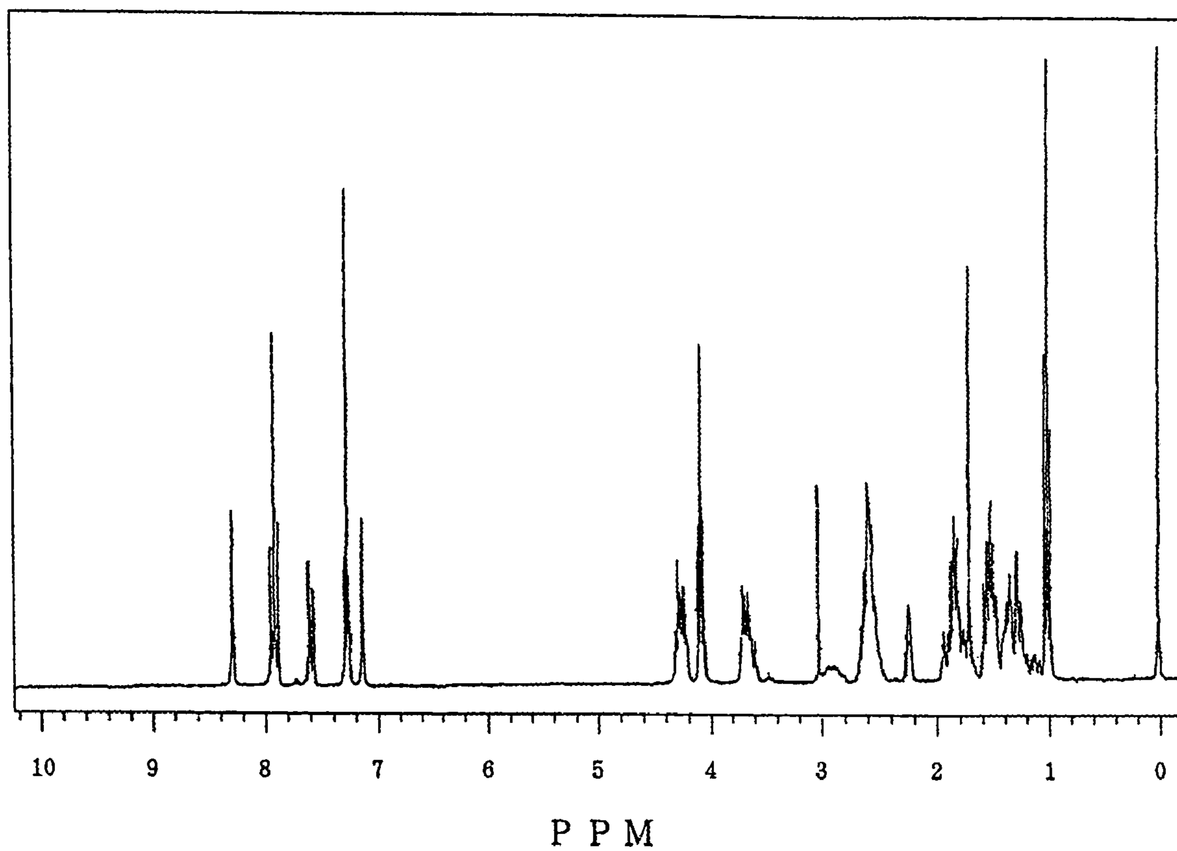
^1\text{H-NMR} spectrometry spectrum of the sulfonium salt (A-6)
