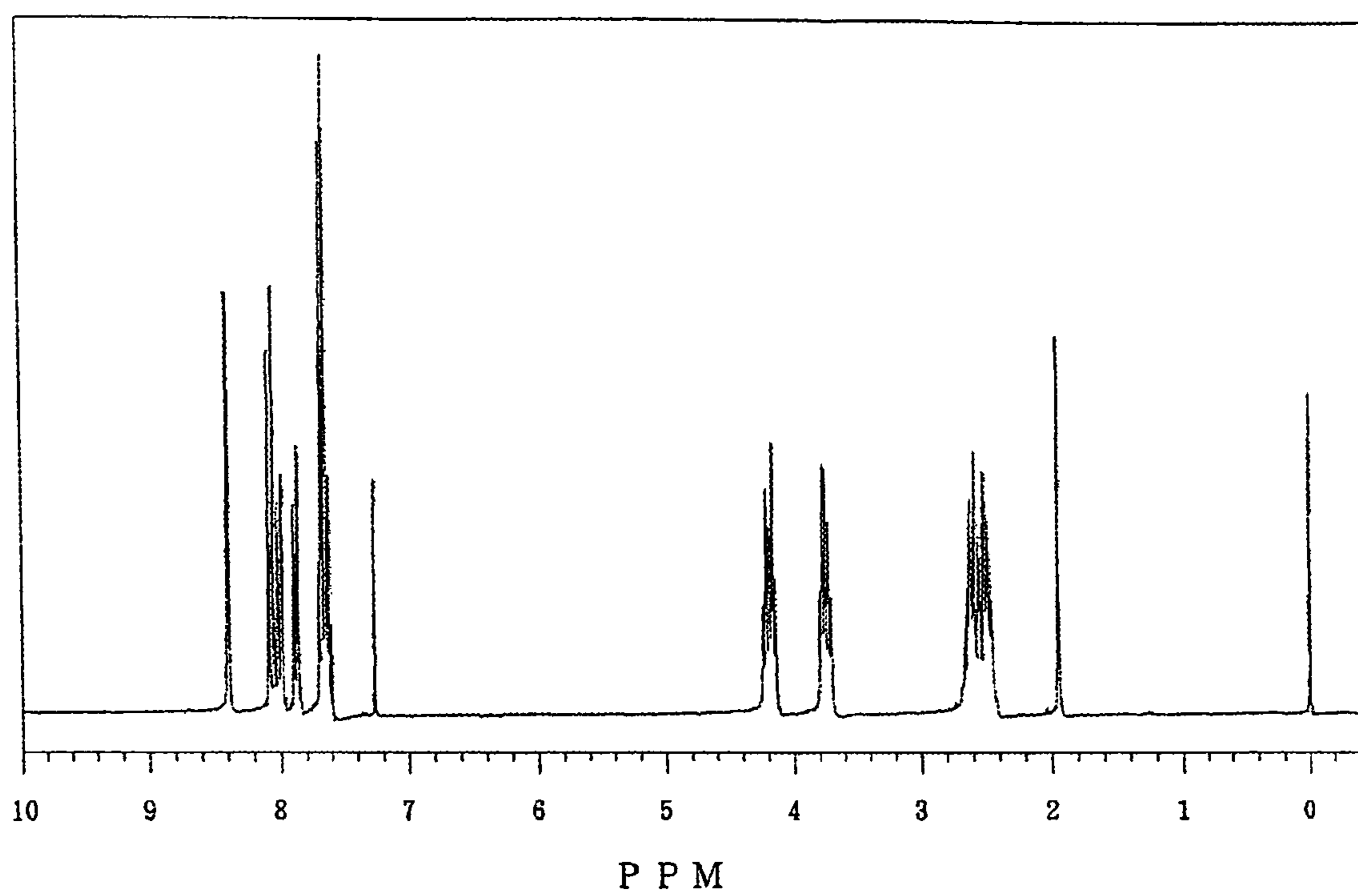
1 H-NMR spectrometry spectrum of the sulfonium salt (A-1)
