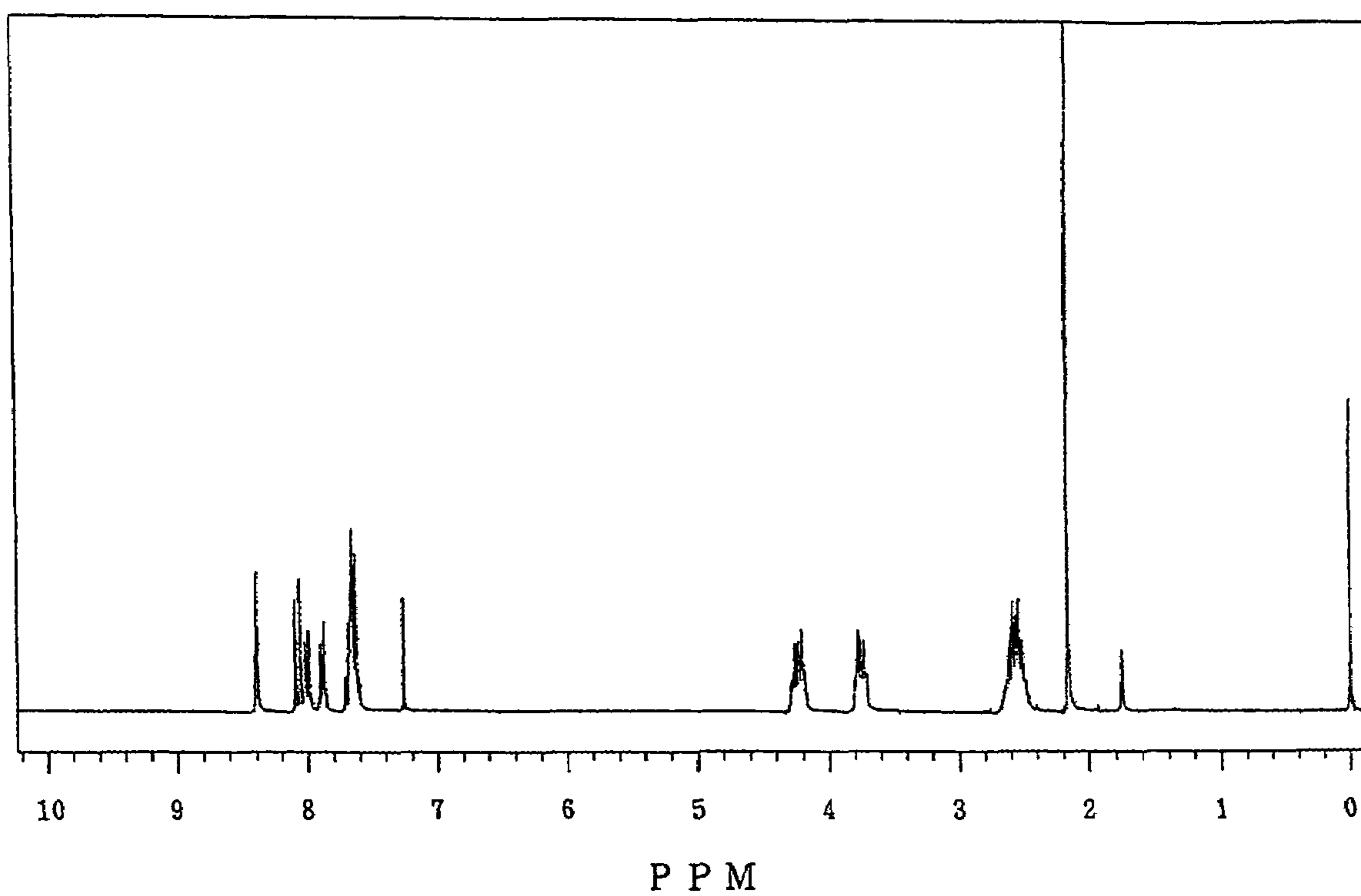
^1\text{H} -NMR spectrometry spectrum of the sulfonium salt (A-3)
