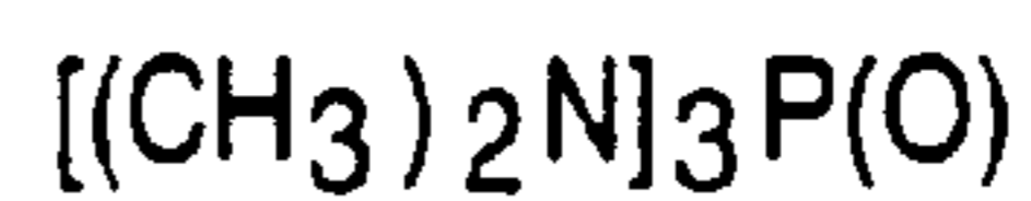
Hexamethylphosphoramide
