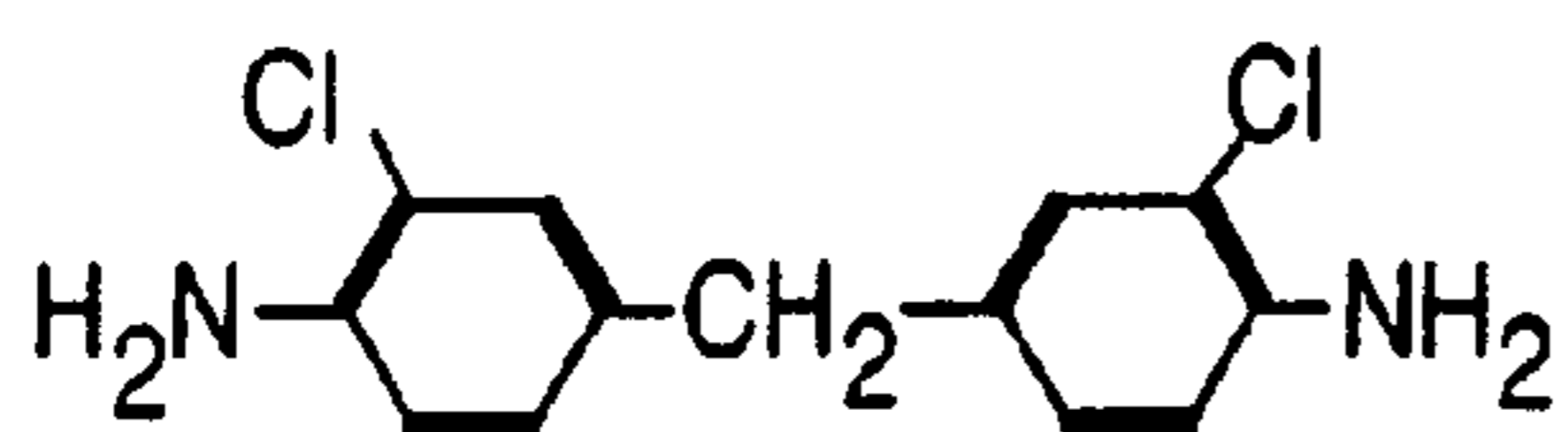
4,4'-Methylene bis[2-chloroaniline]
