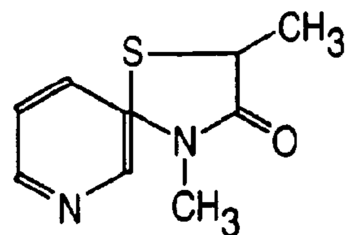
SM-12502
