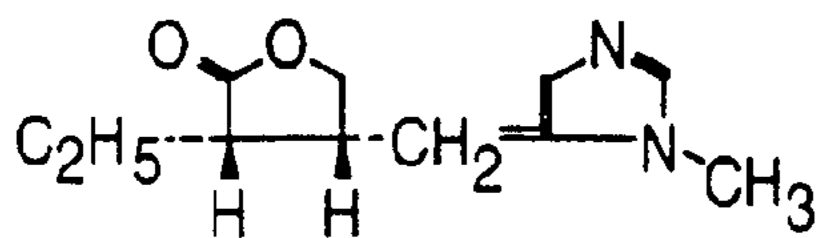
Pilocarpine
