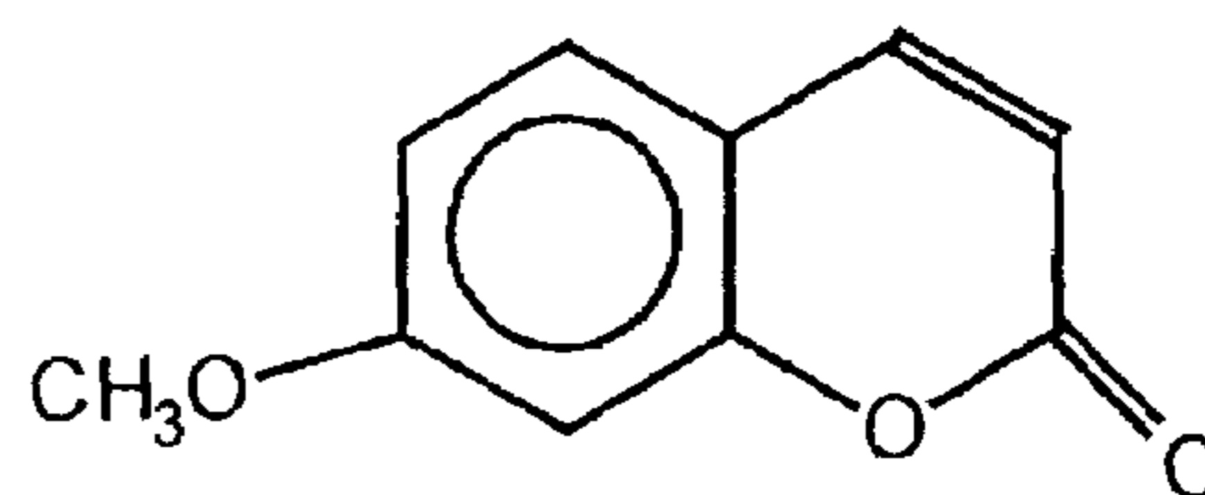
7-Methoxycoumarin
