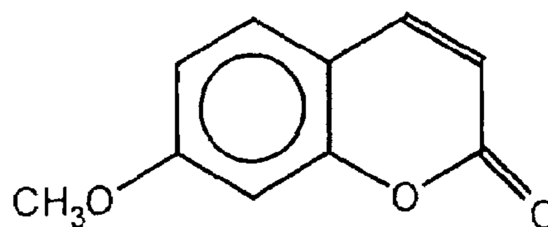
7-Methylcoumarin
