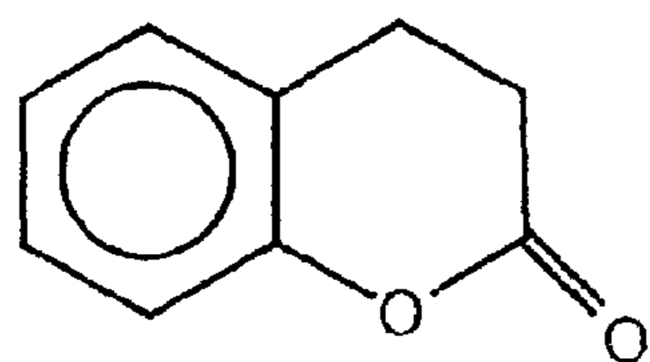
Dihydrocoumarin
