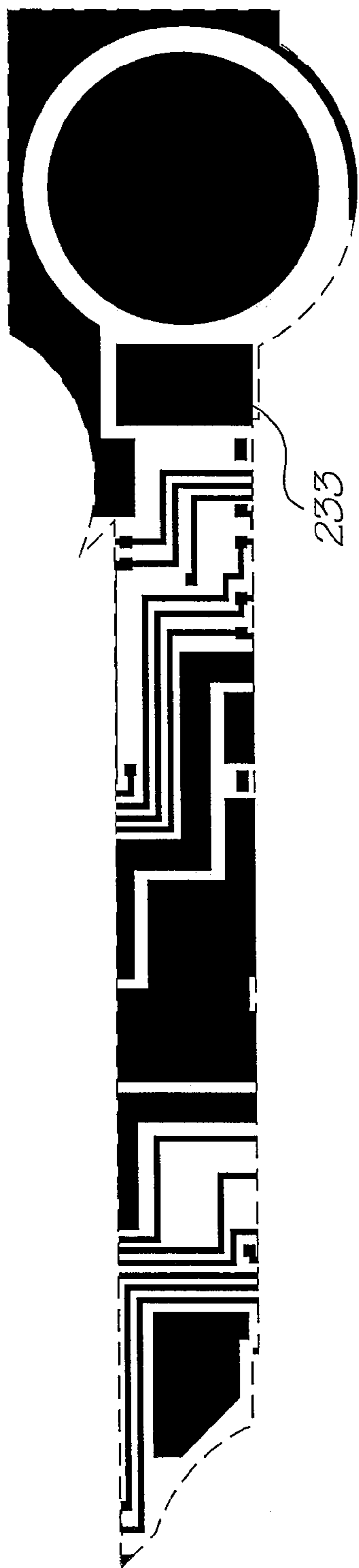
Metal 2 mask
