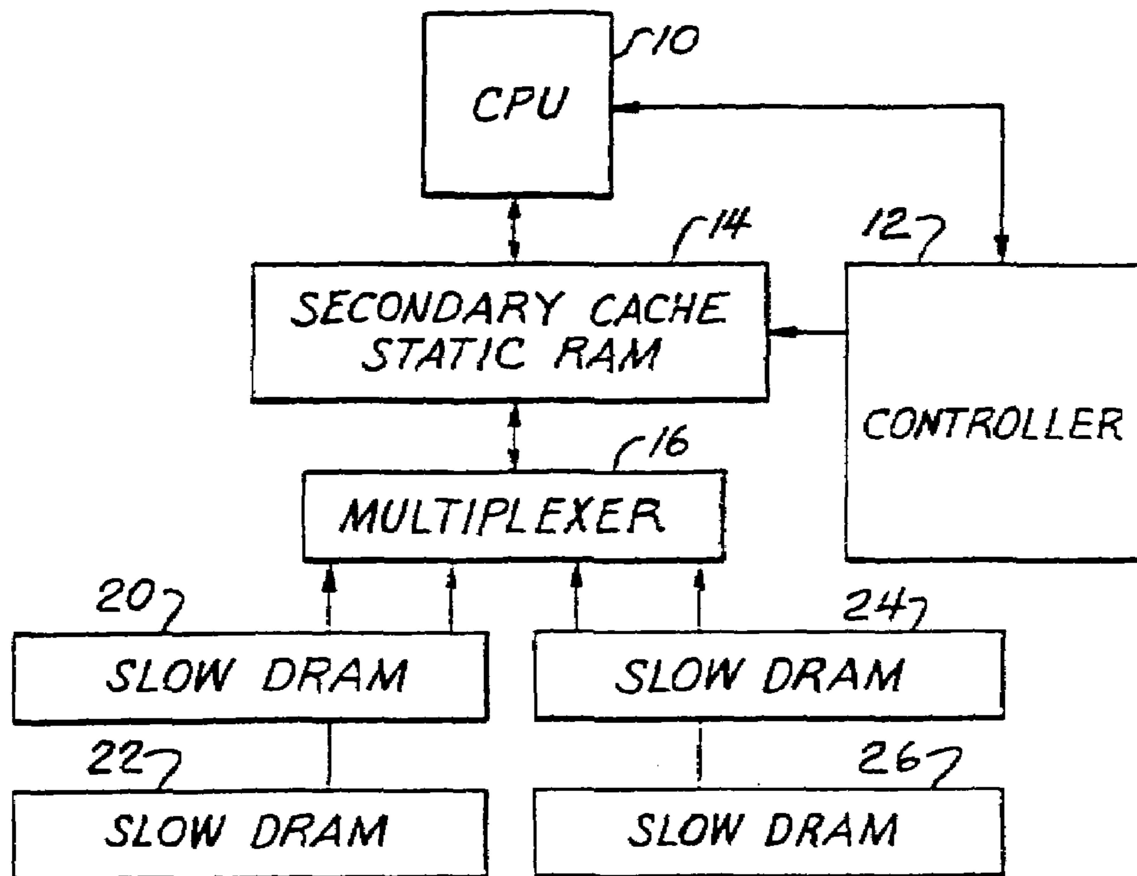
FIG. 1 PRIOR ART
