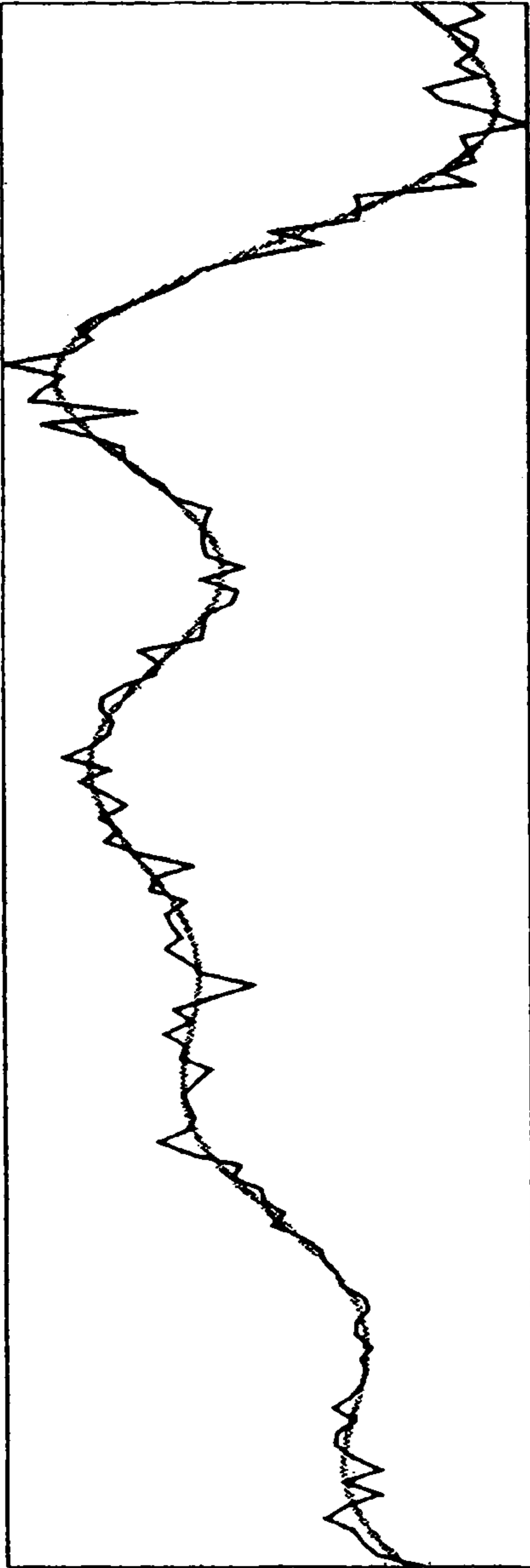
Signal & Reconstruction
