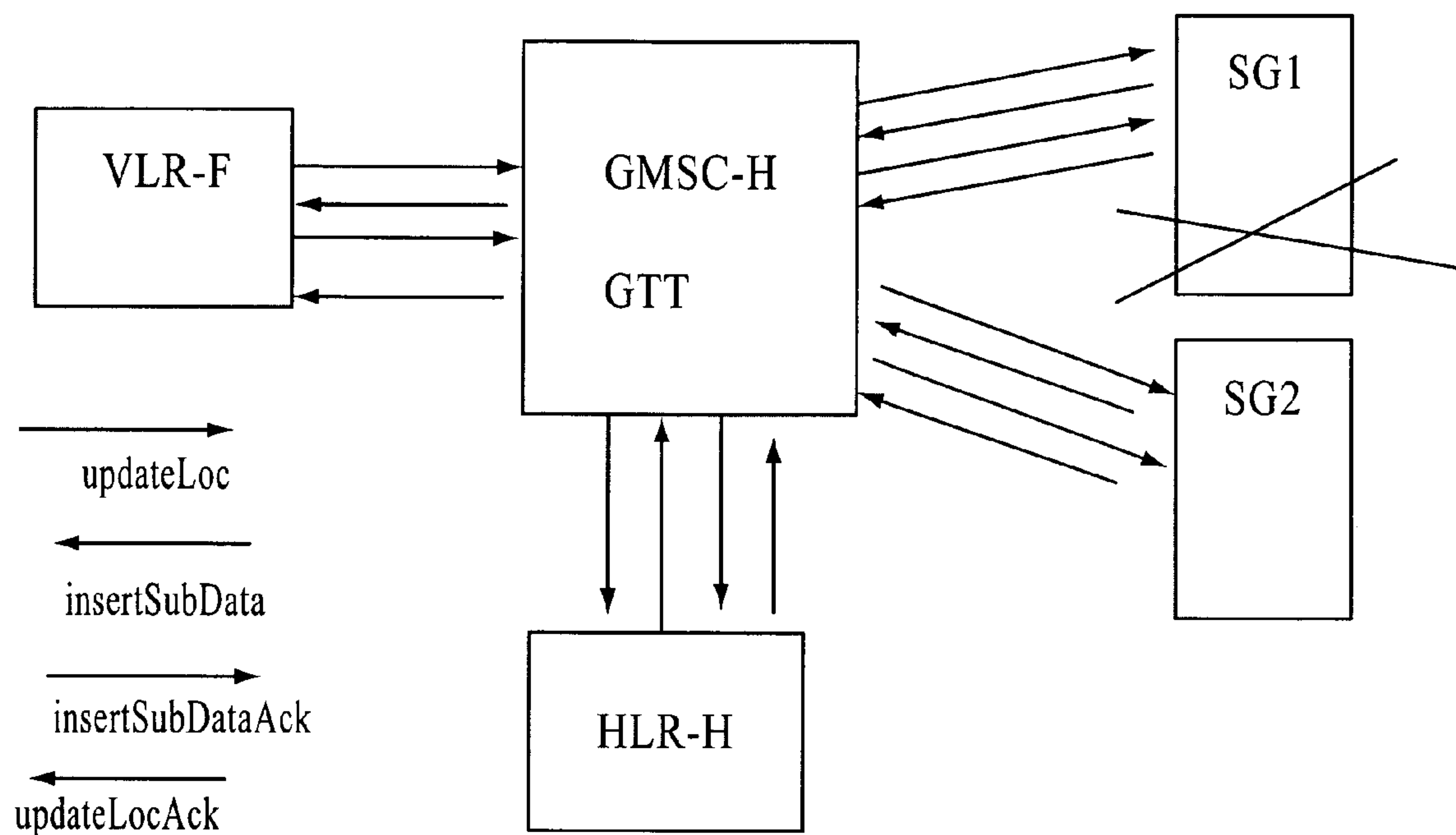
Update Location Transaction Flow When SG1 failed after insertSubData
