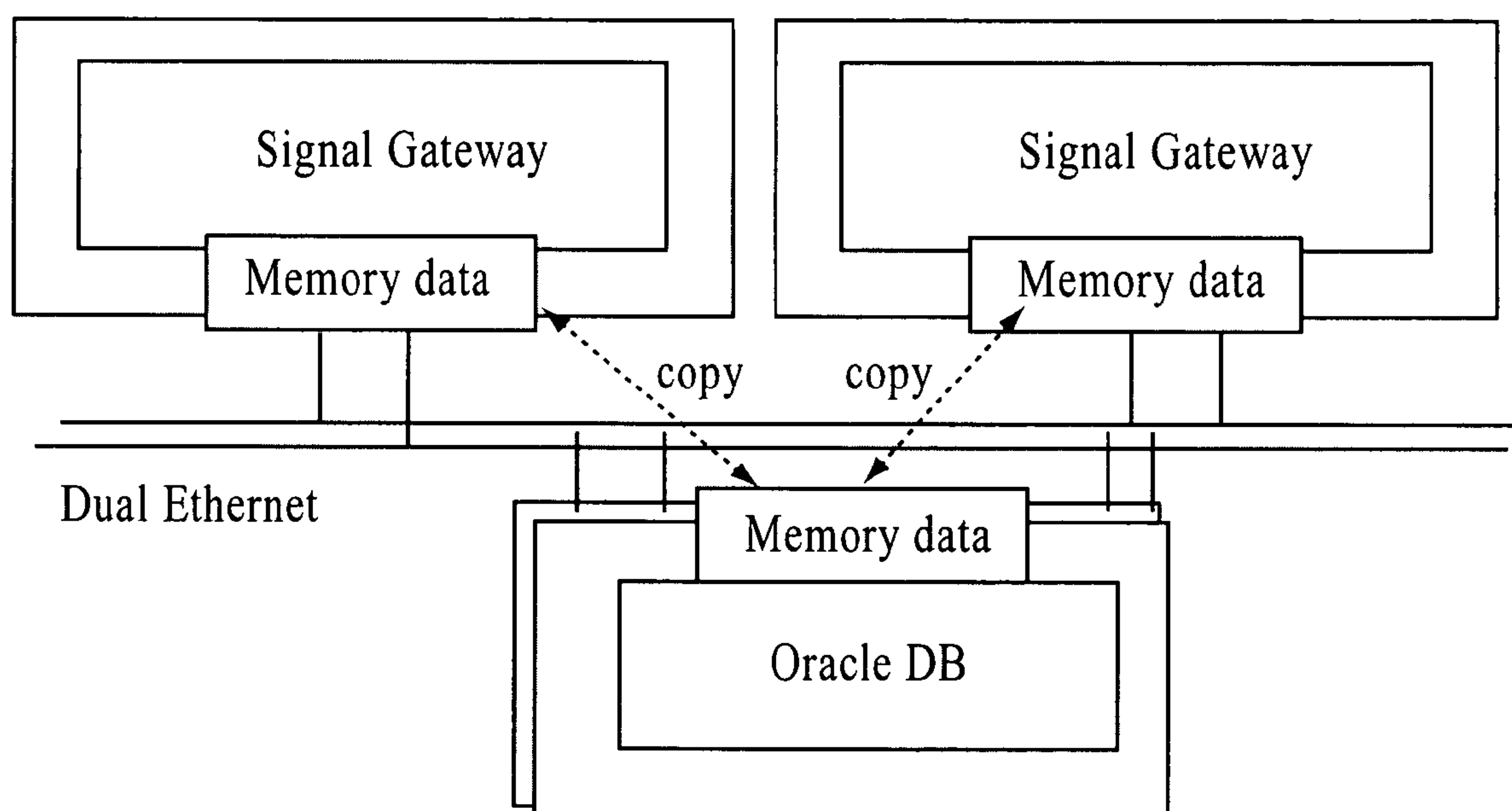
Signal gateway architecture
