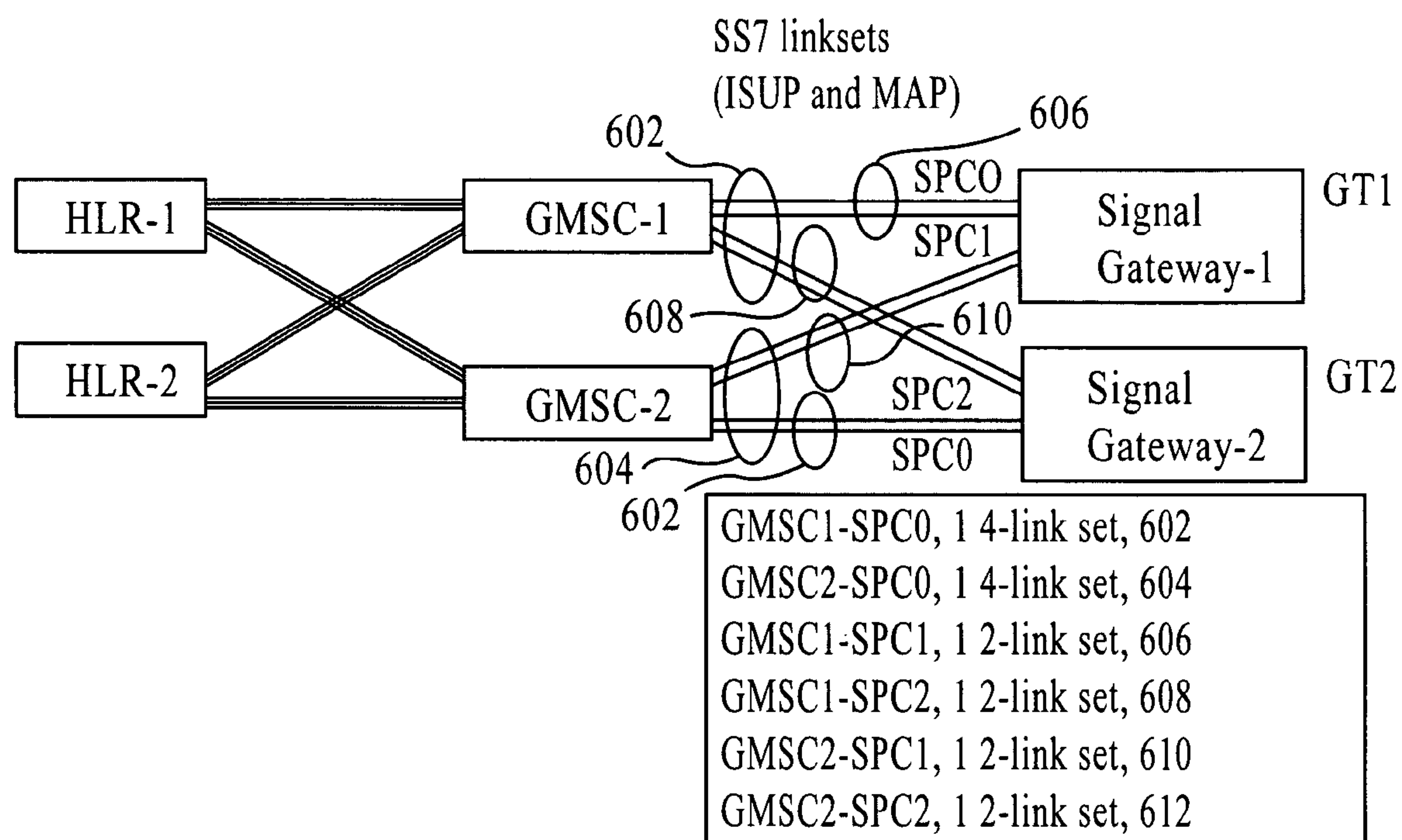
GT and SPC in one possible linkset configuration
