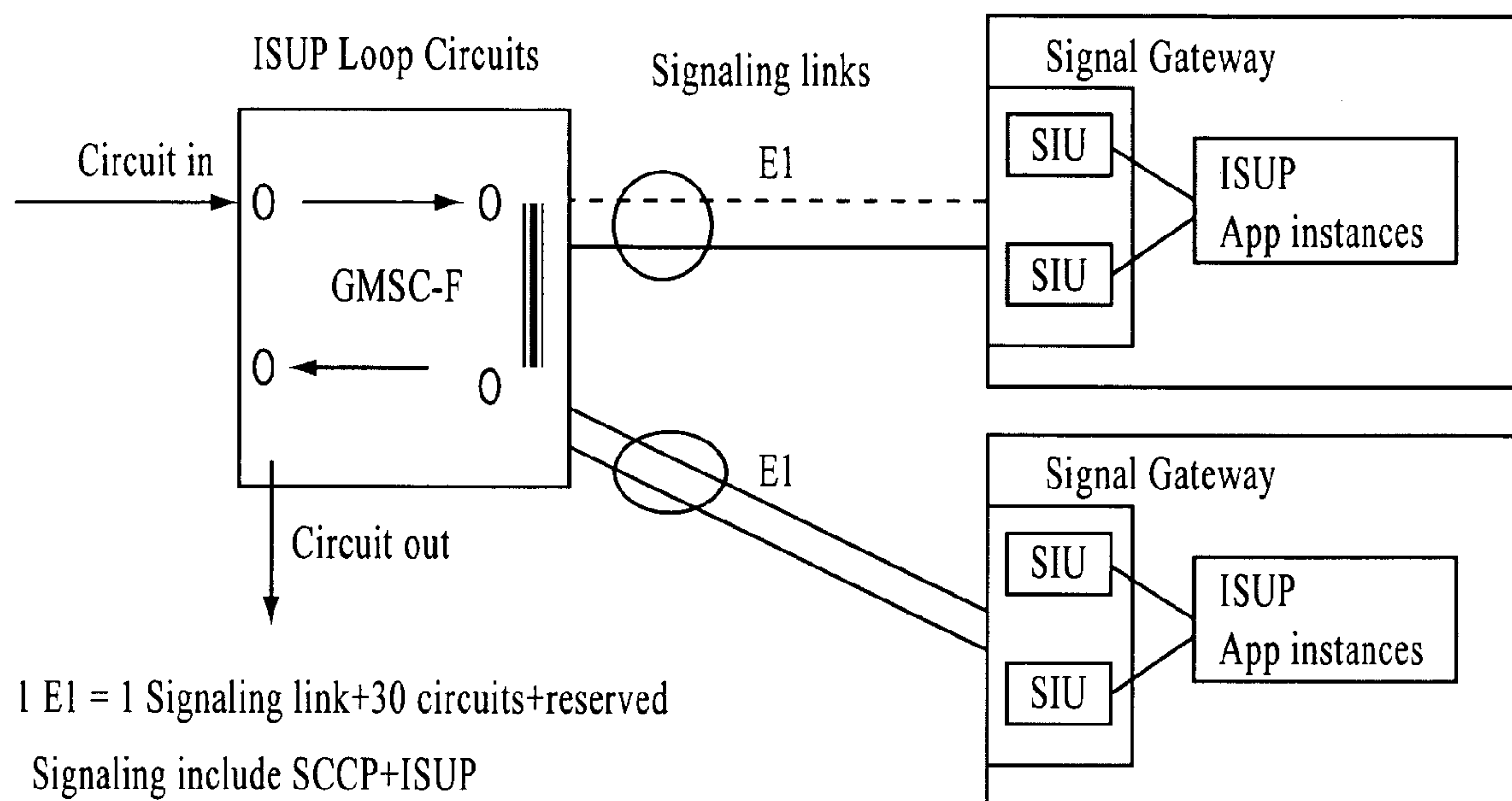
ISUP loopback circuits and Signaling
