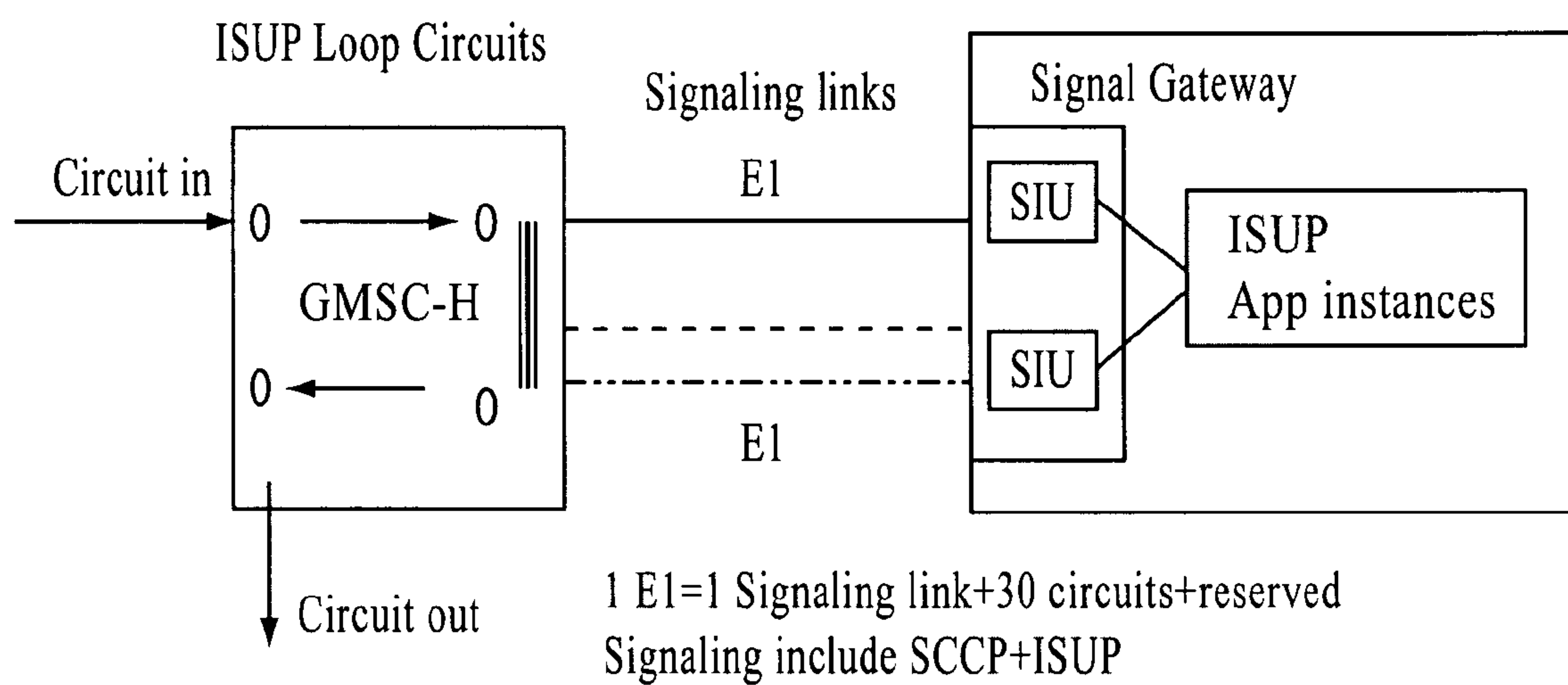
ISUPLoopbackcircuits and Signaling
