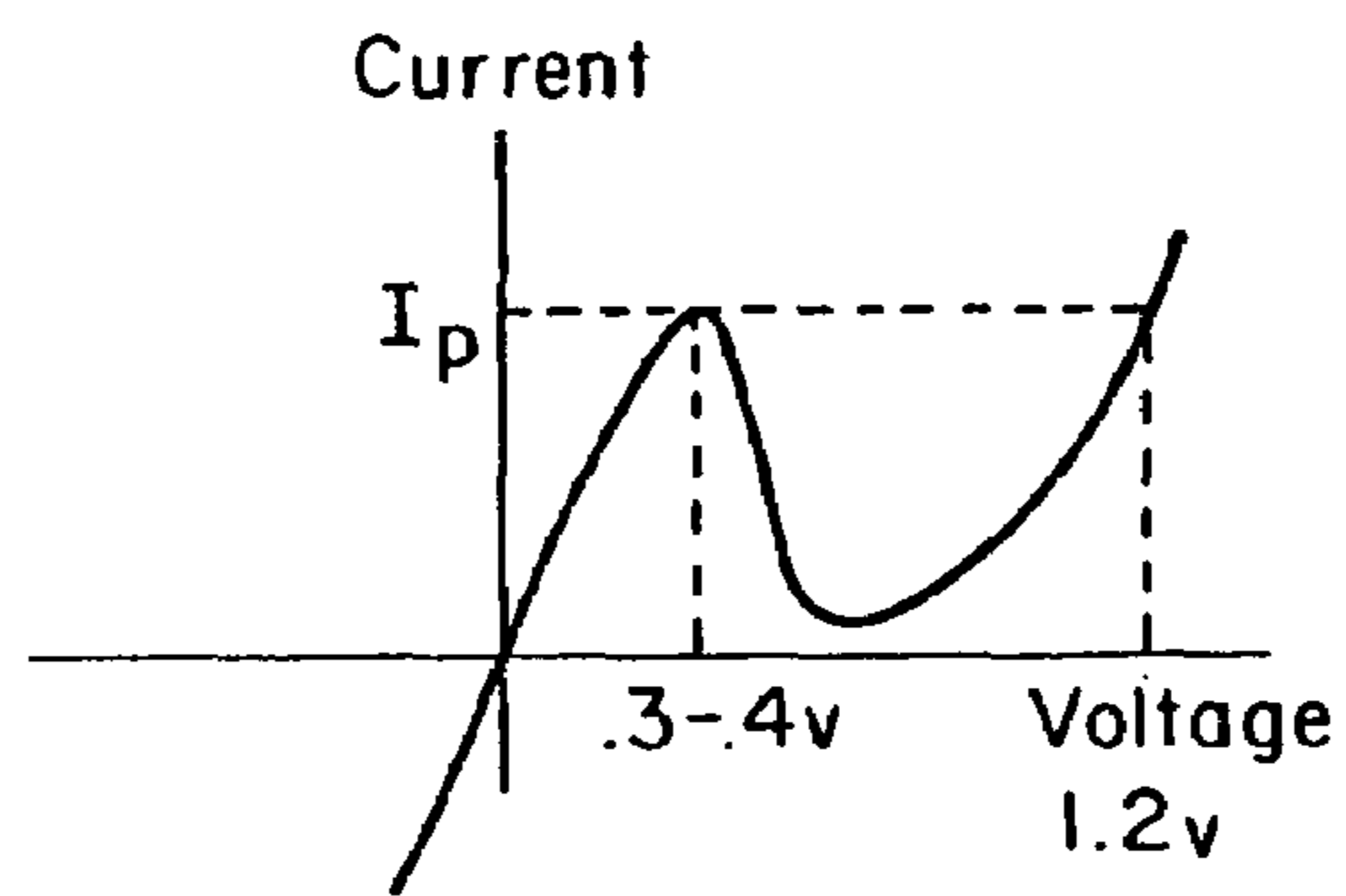
TUNNEL DIODE
