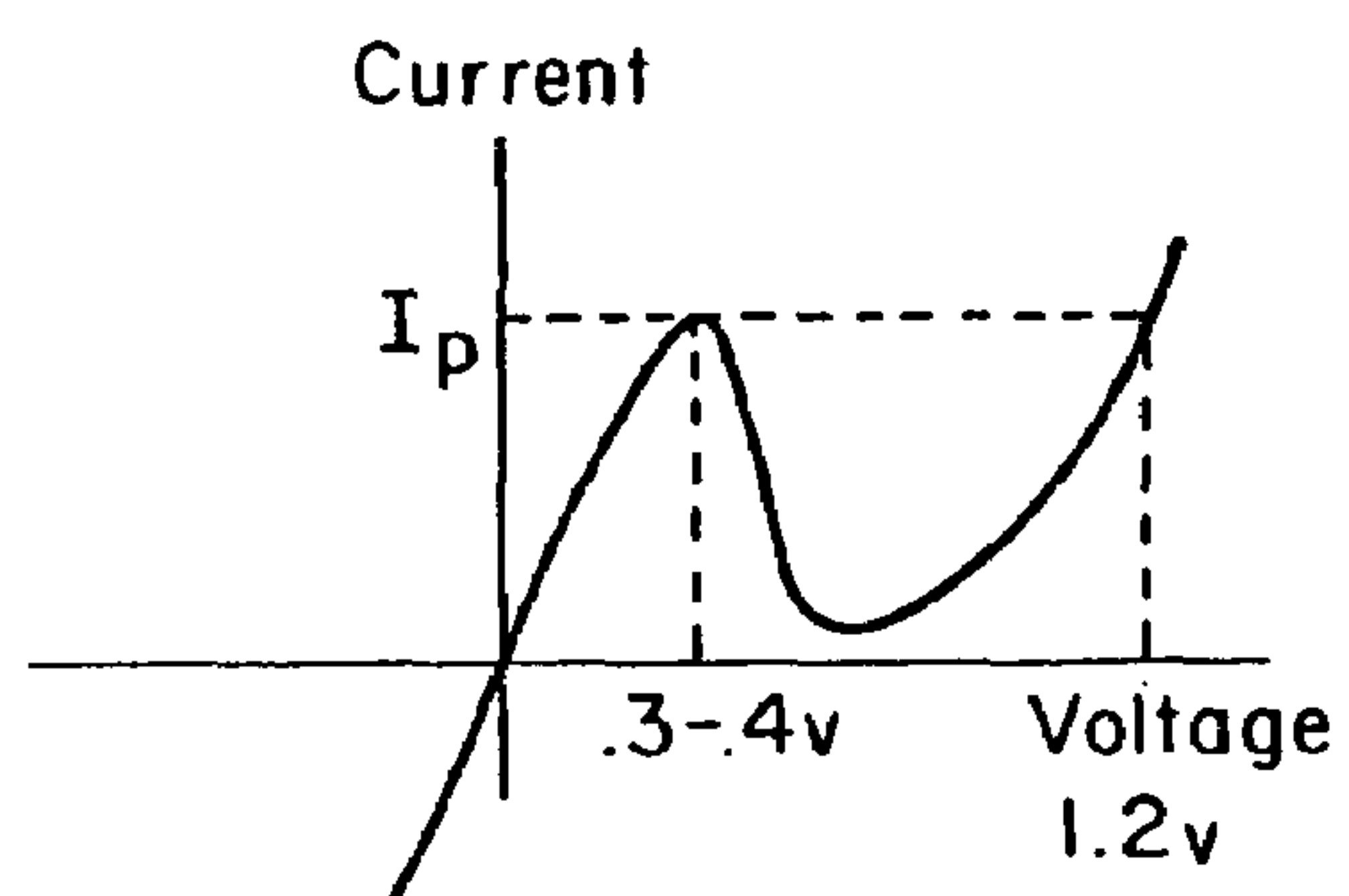
TUNNEL DIODE
