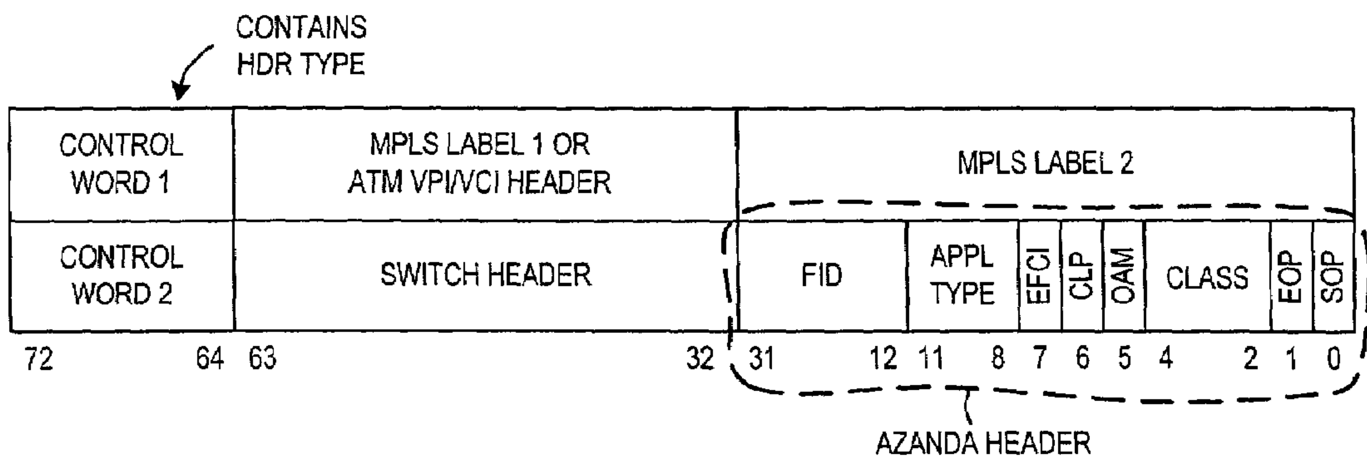
FORMAT OF ONE FID ENTRY IN HEADER TABLE
