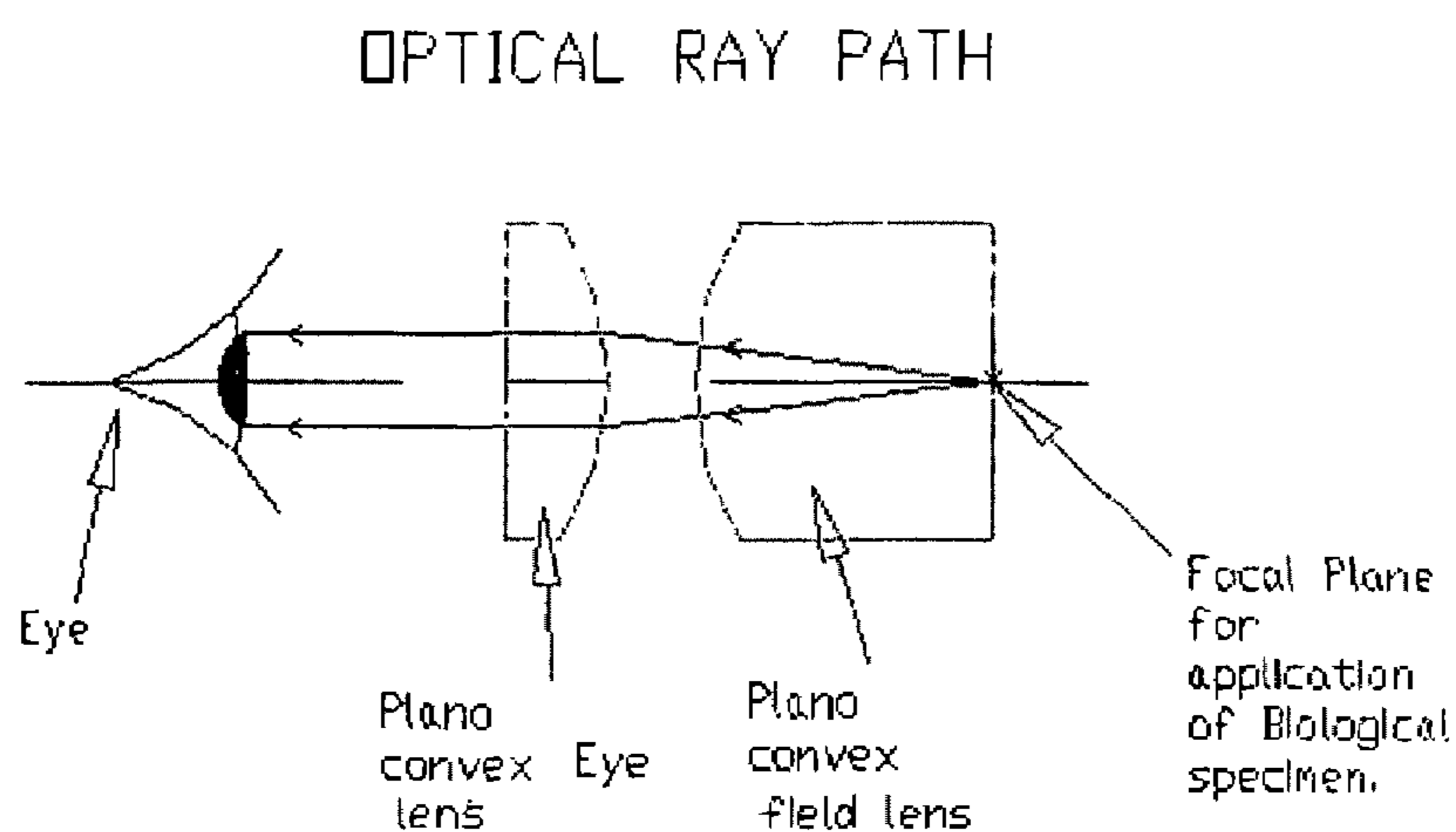
FIGURE 6(A): BASIC OPTICAL RAY PATH INSIDE THE EYEPIECE
