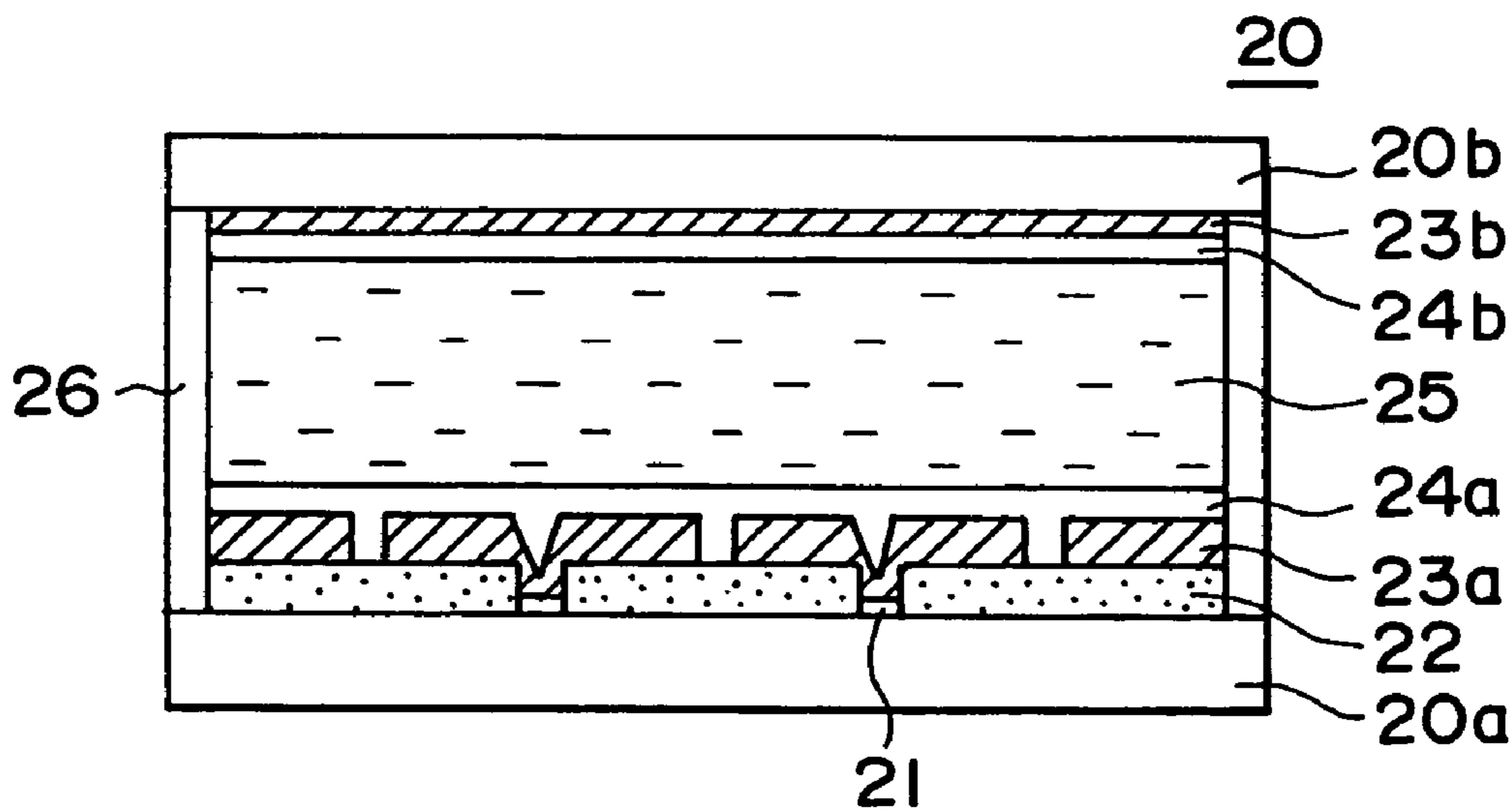
FIG.15 PRIOR ART
