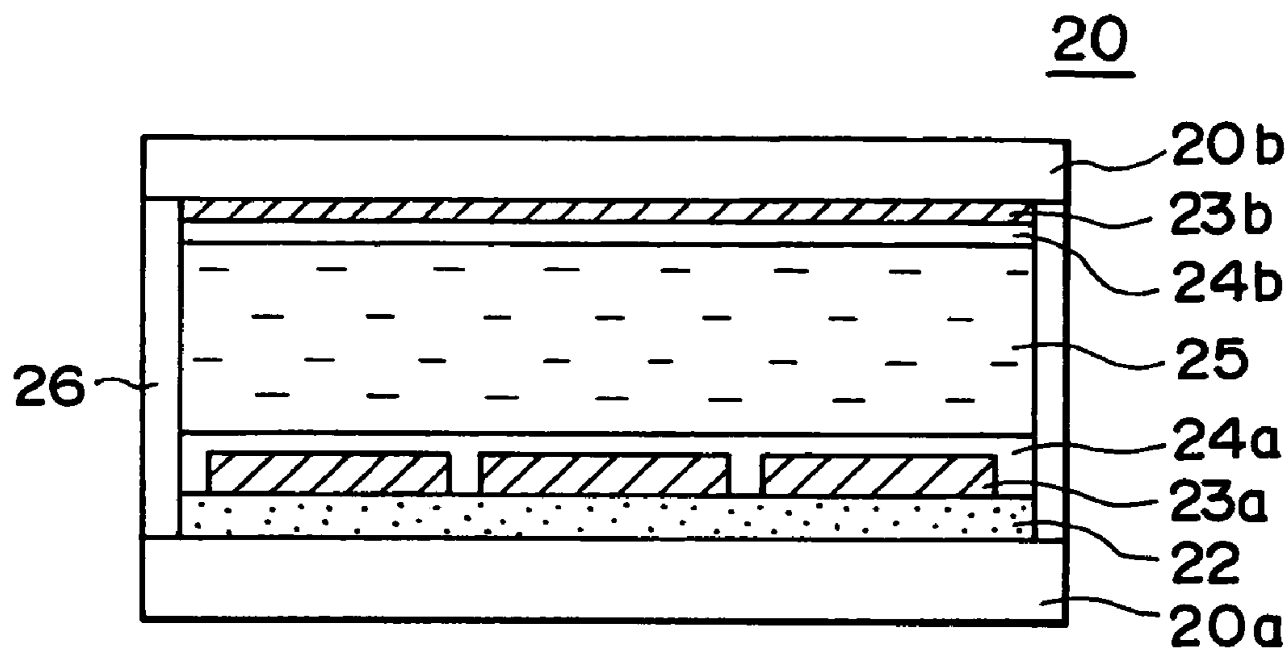
FIG.14 PRIOR ART
