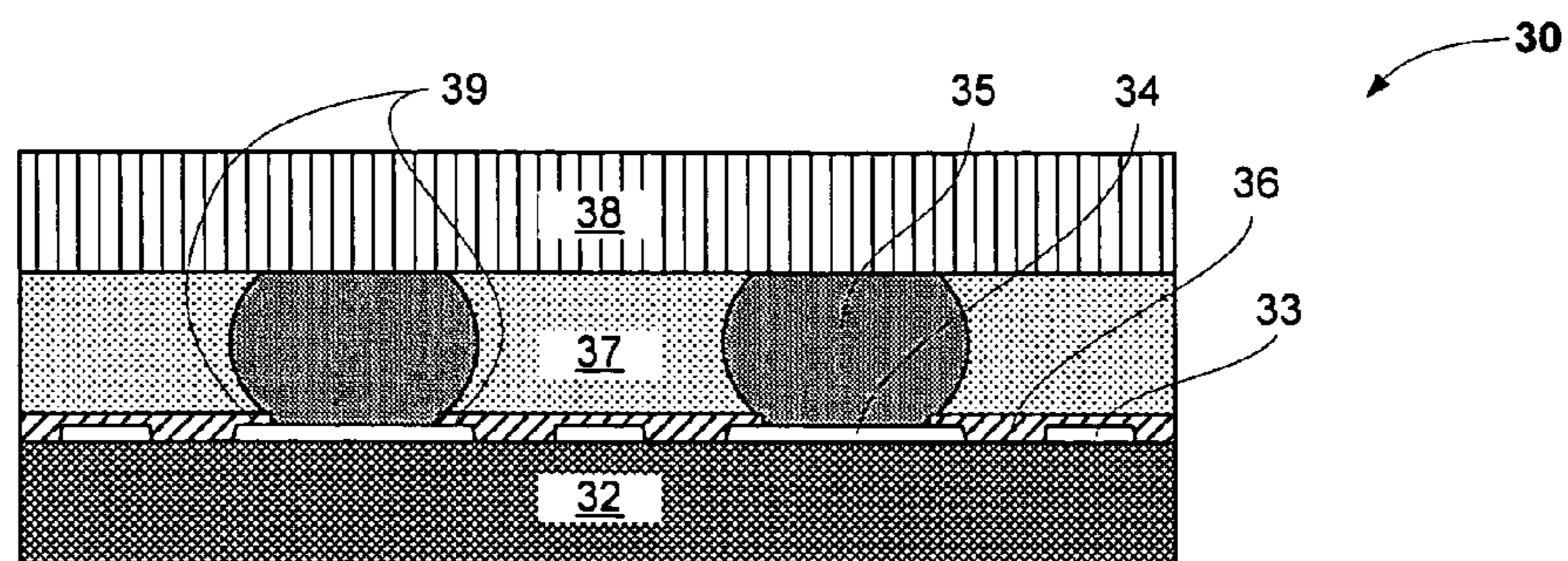
Fig. 3 (Prior Art)
