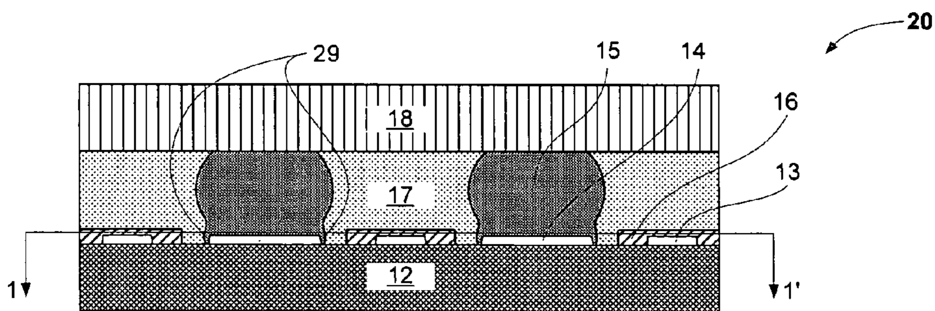
Fig. 2 (Prior Art)
