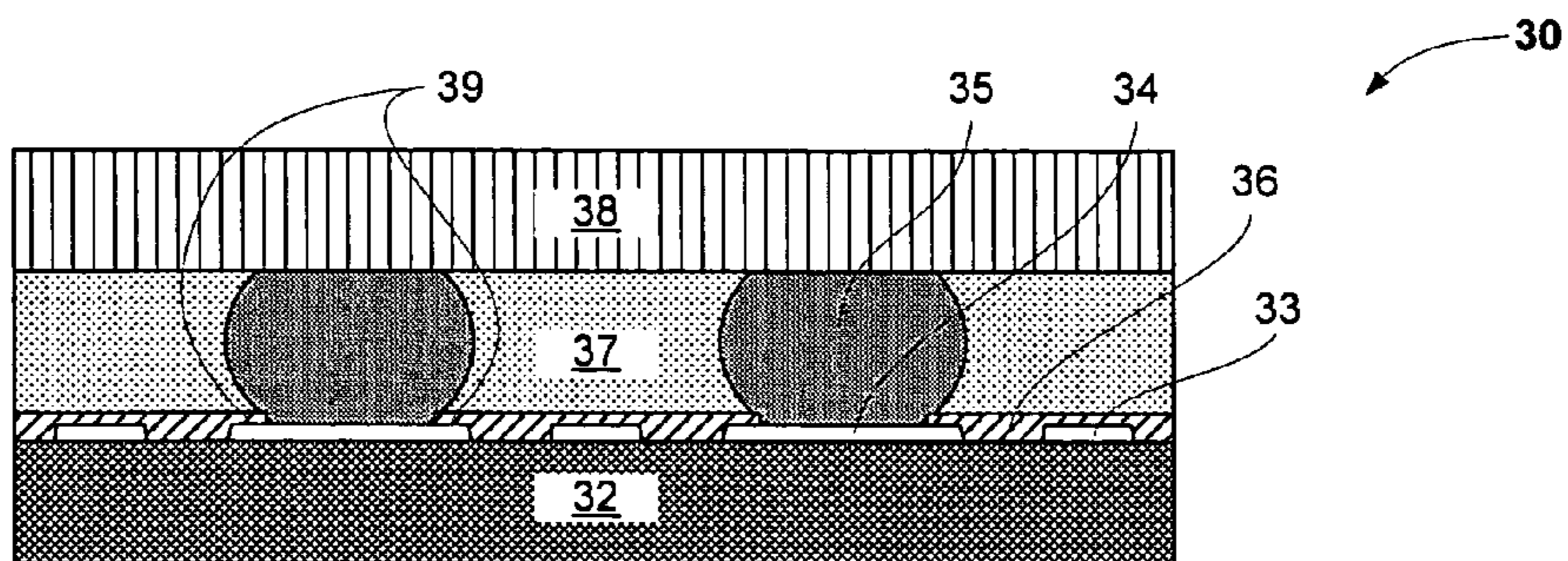
Fig. 3 (Prior Art)
