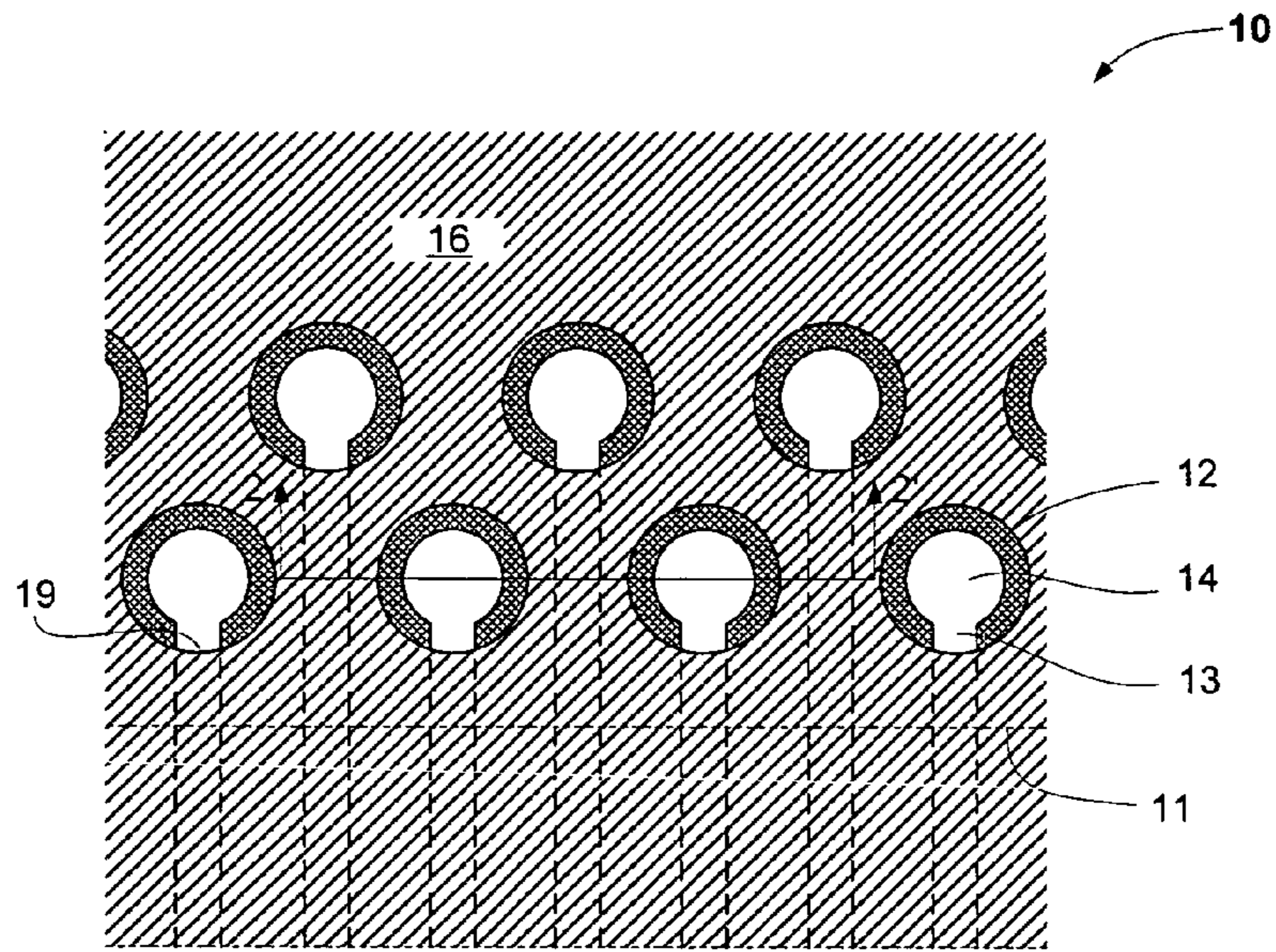
Fig. 1 (Prior Art)
