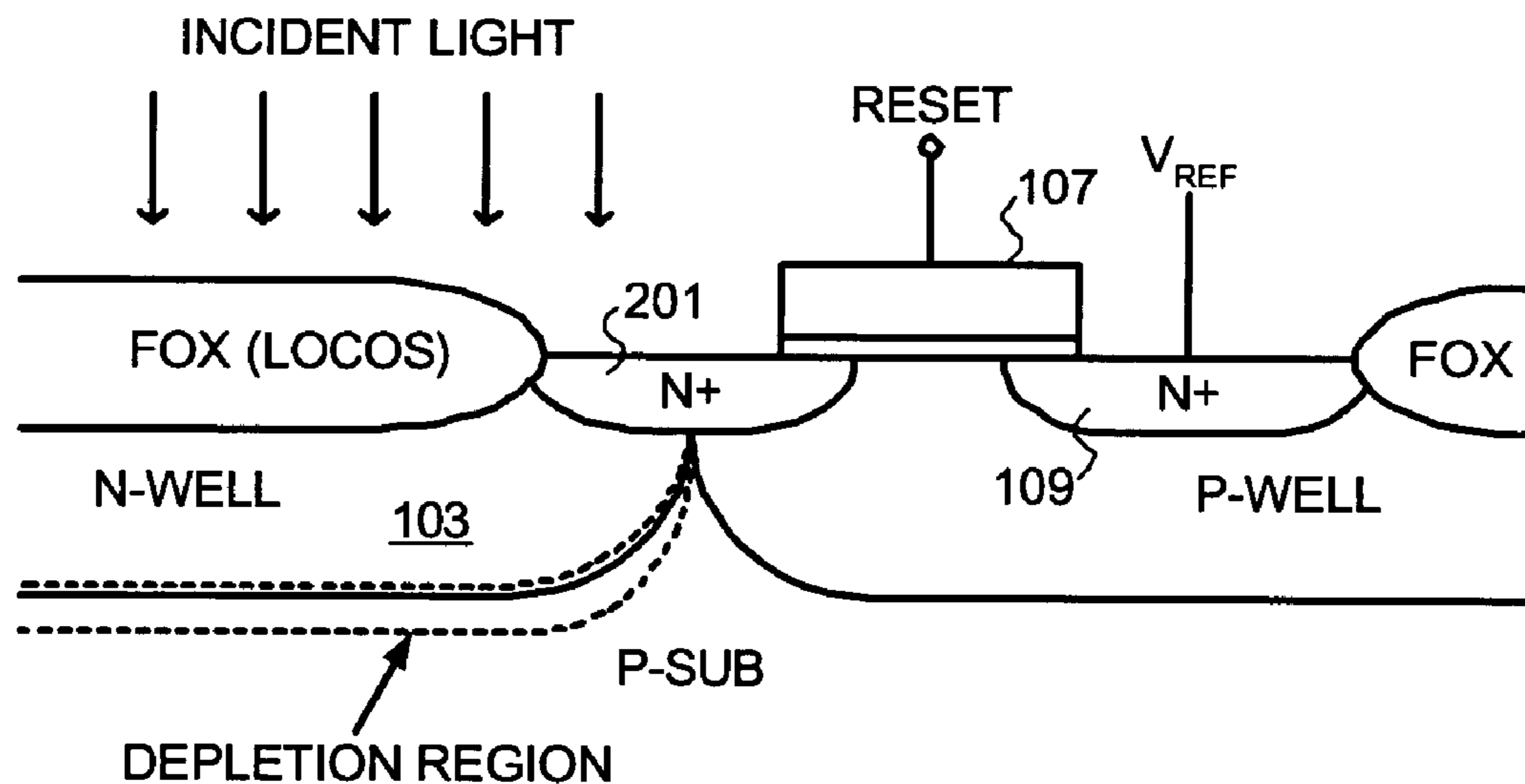
FIGURE 2 (PRIOR ART)
