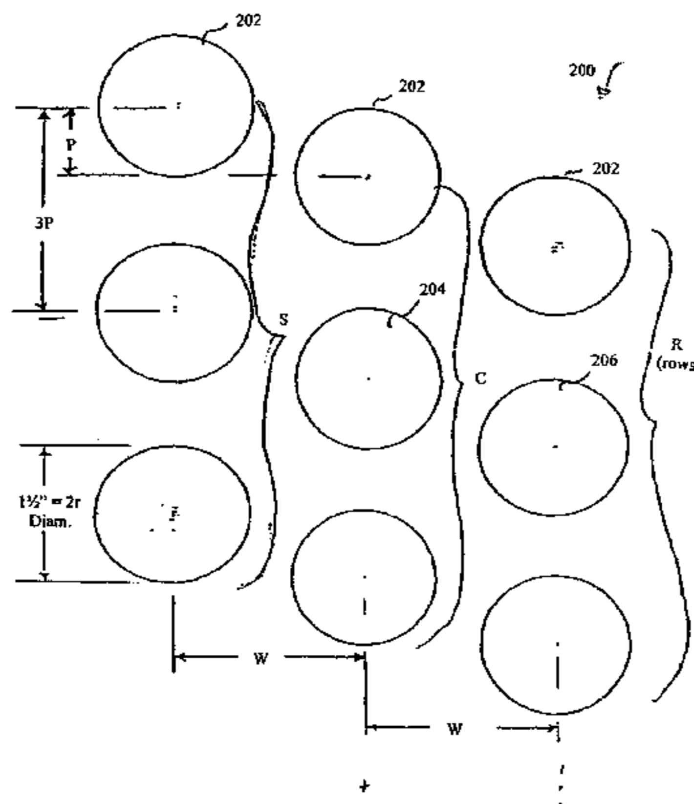
Detector Configuration: 3 Vertical Rows, 112 in Each Row
