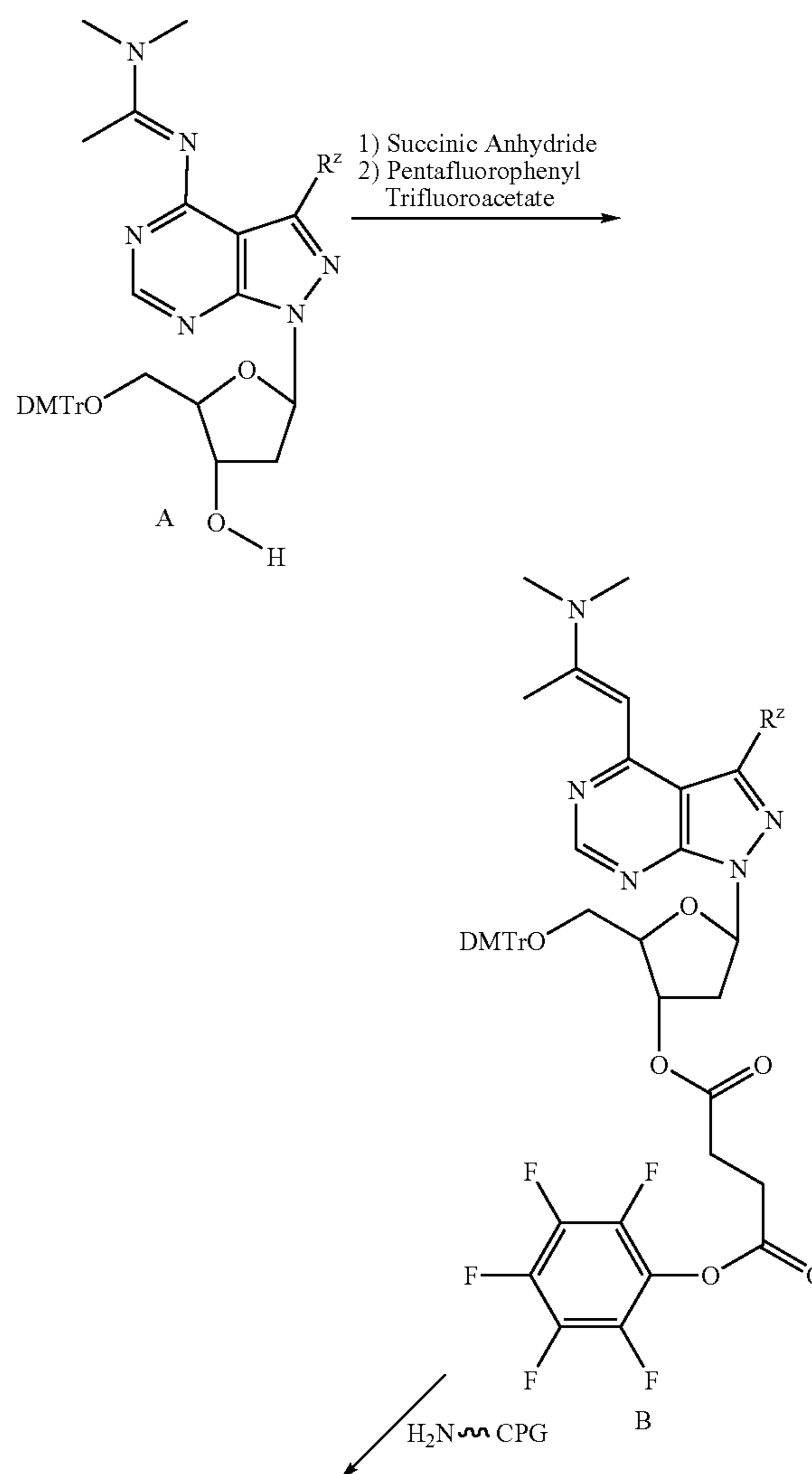
Reaction Scheme 11
