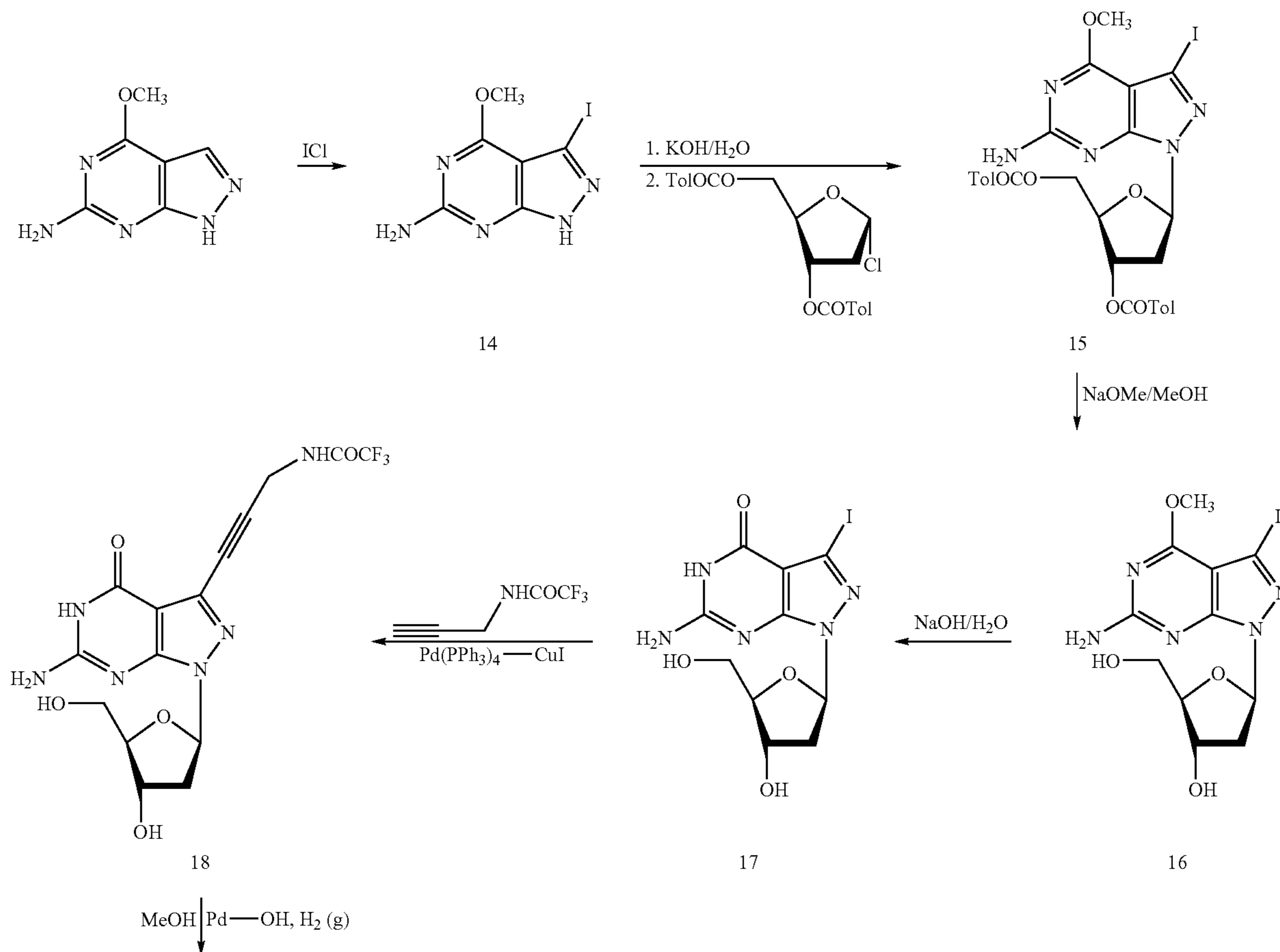
Reaction Scheme 4
