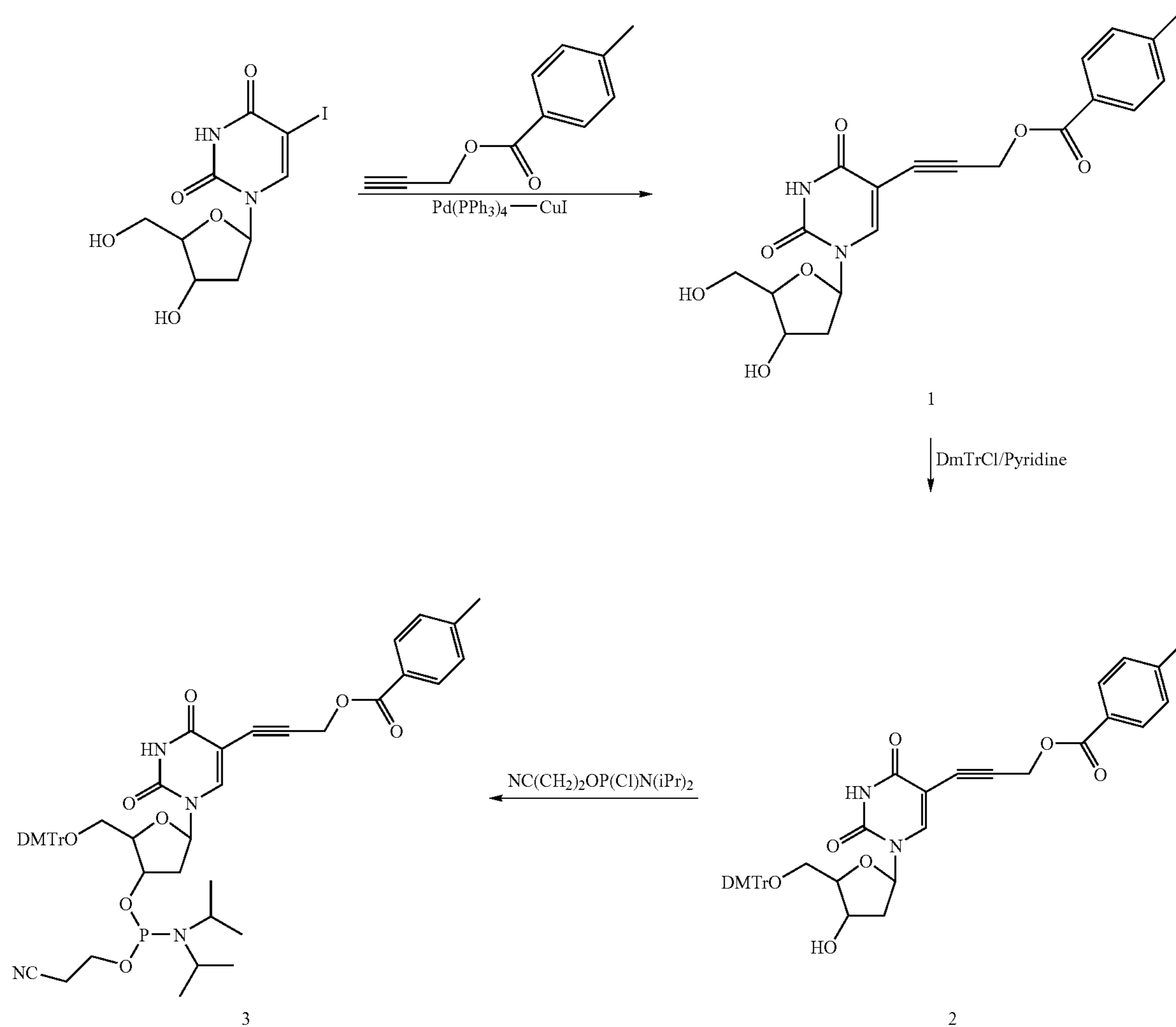
Reaction Scheme 1
