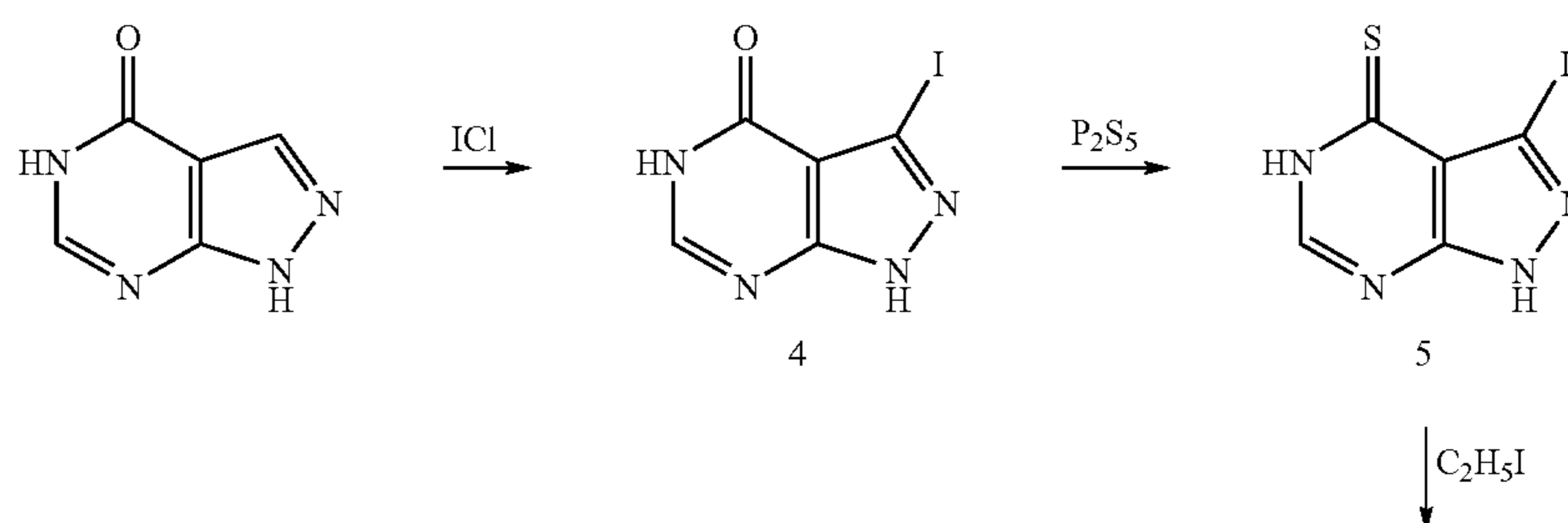
Reaction Scheme 2
