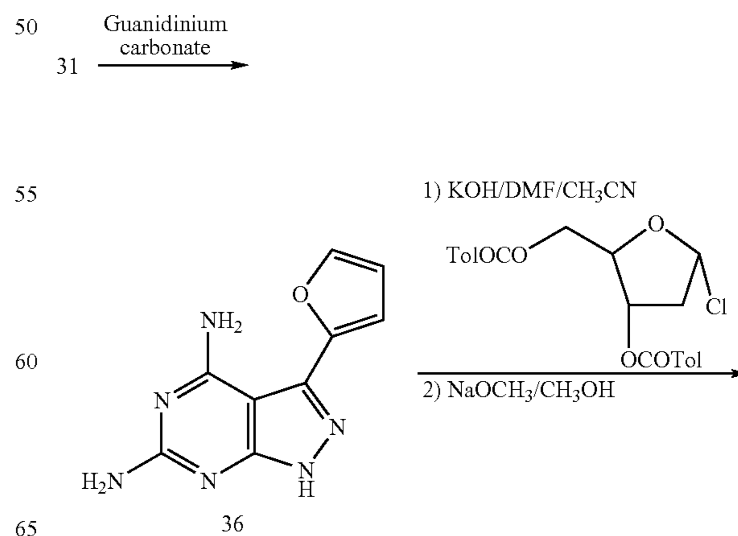
Reaction Scheme 9
