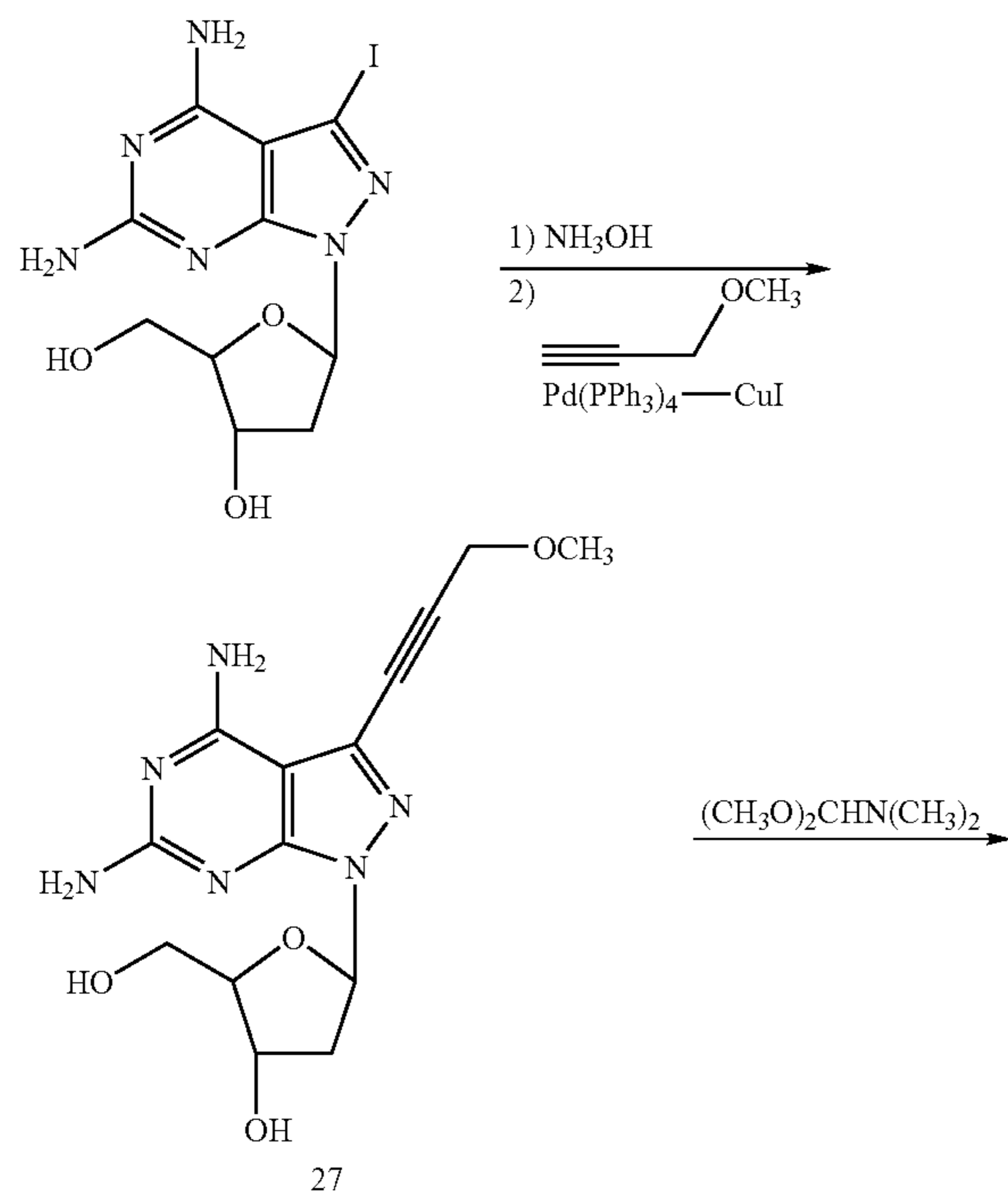
Reaction Scheme 7
