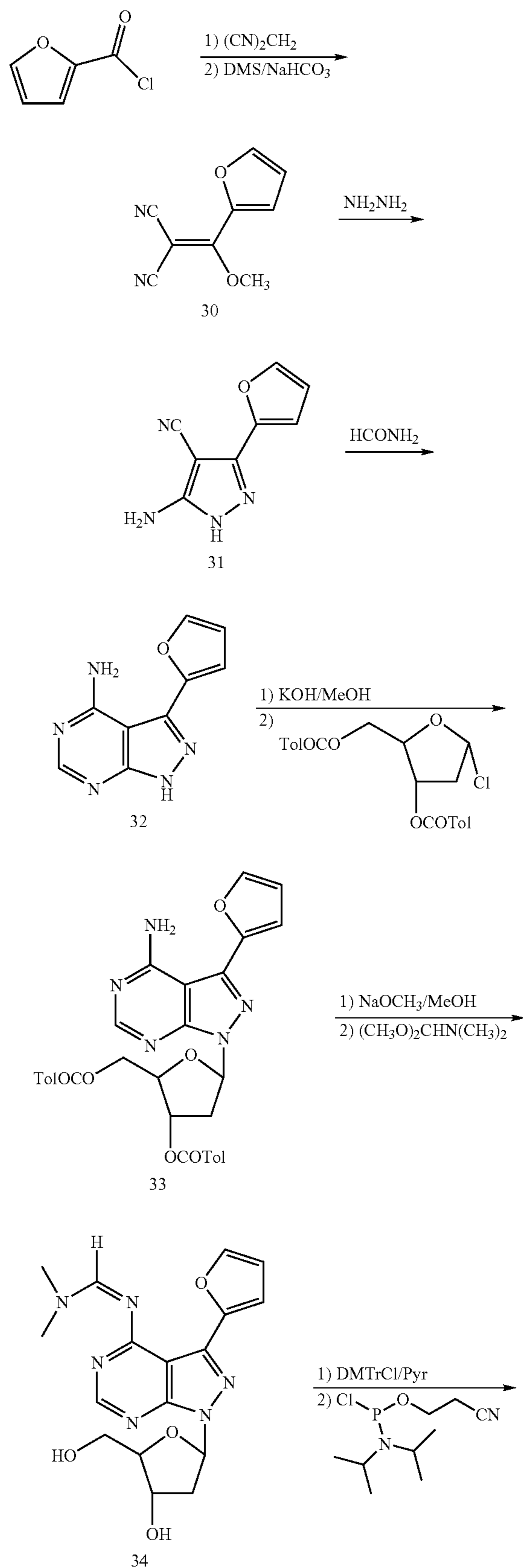
Reaction Scheme 8
