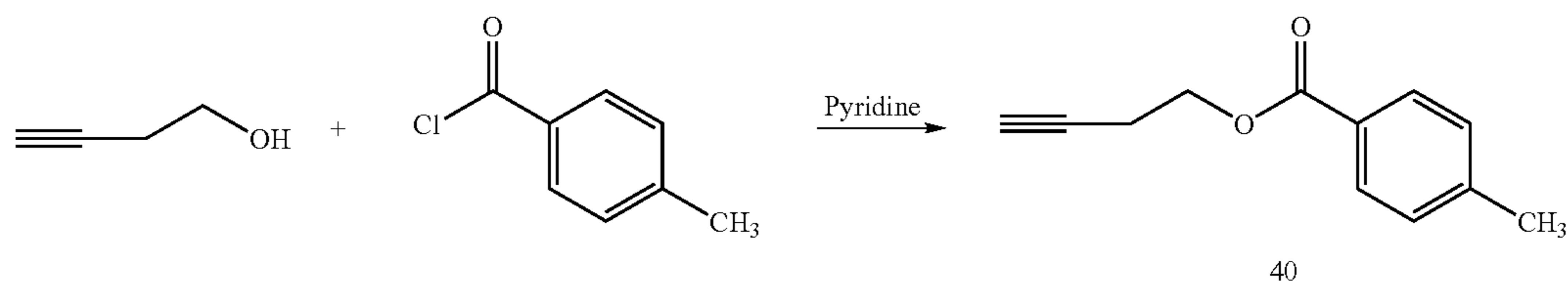
Reaction Scheme 10
