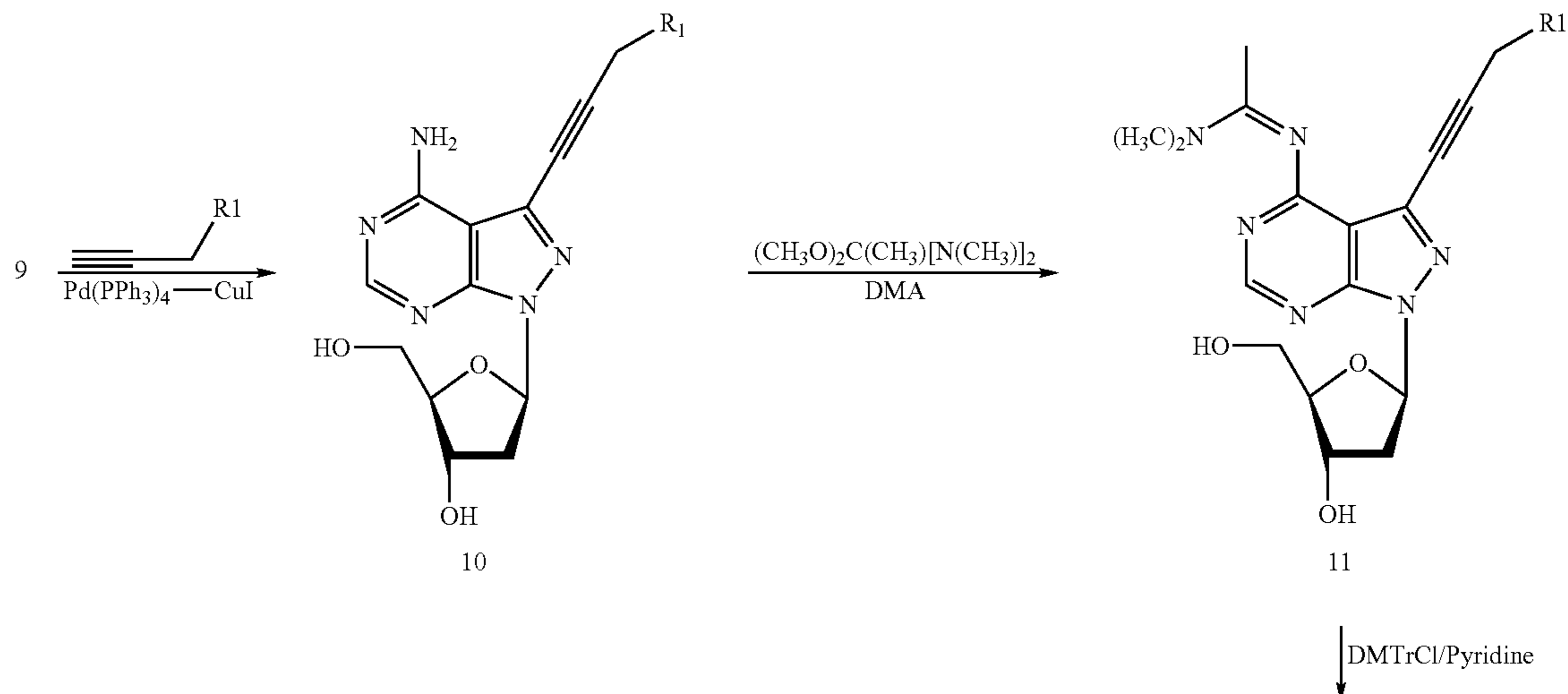
Reaction Scheme 3
