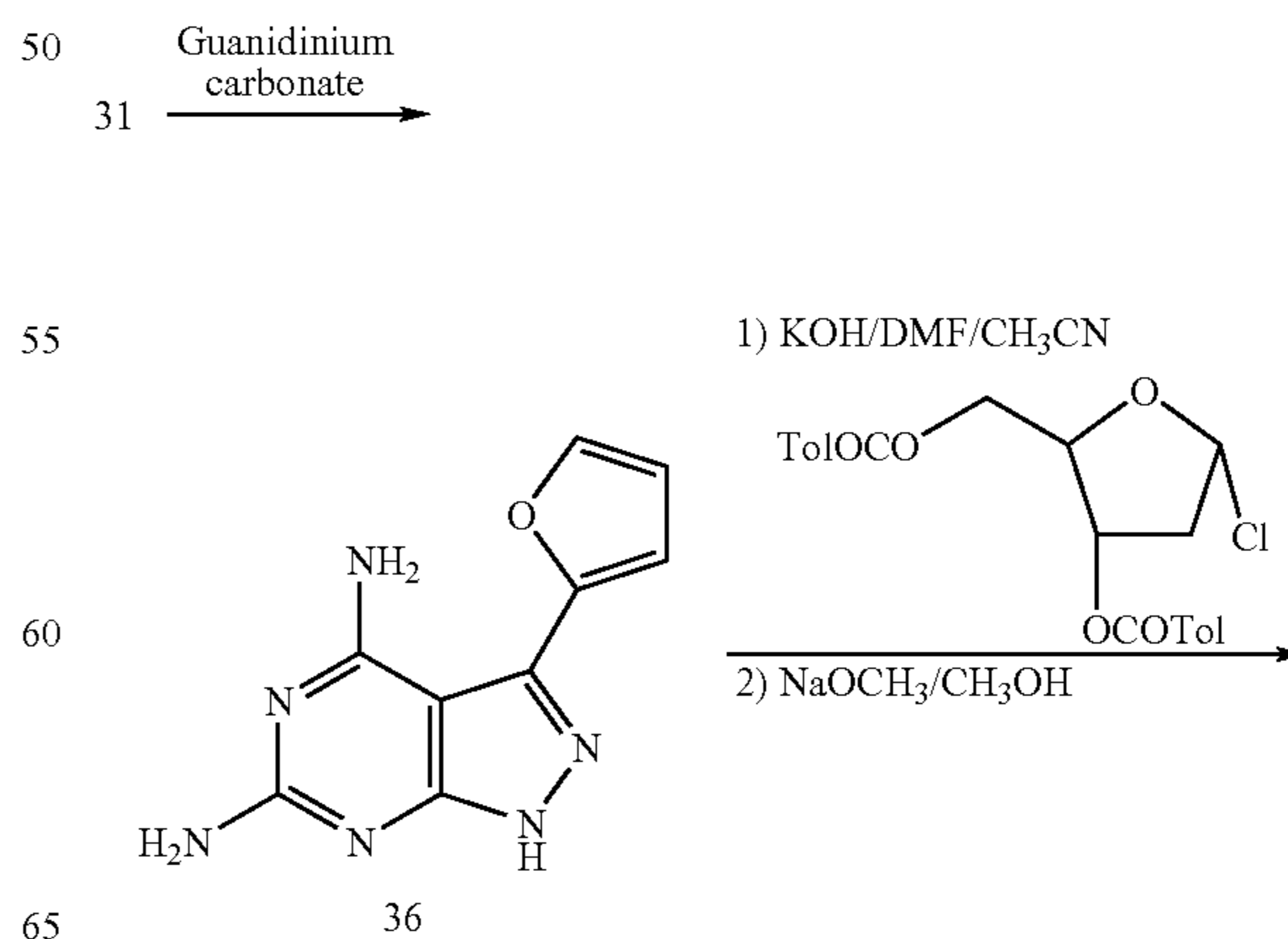
Reaction Scheme 9
