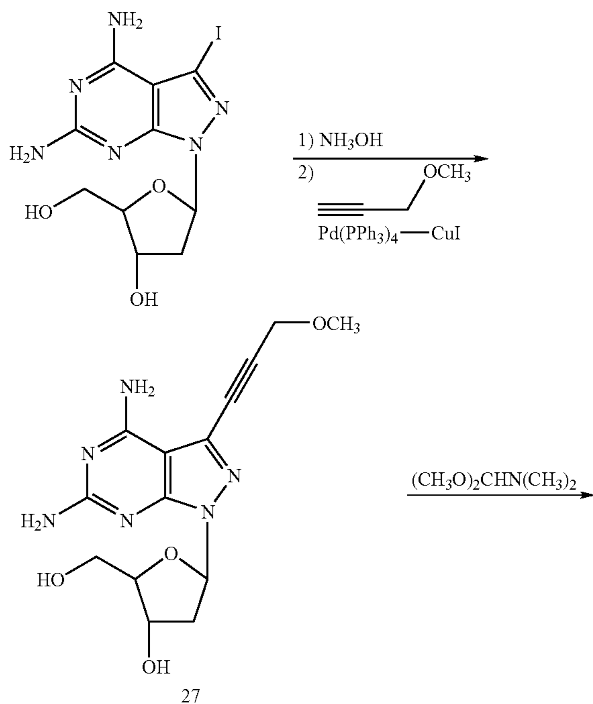
Reaction Scheme 7
