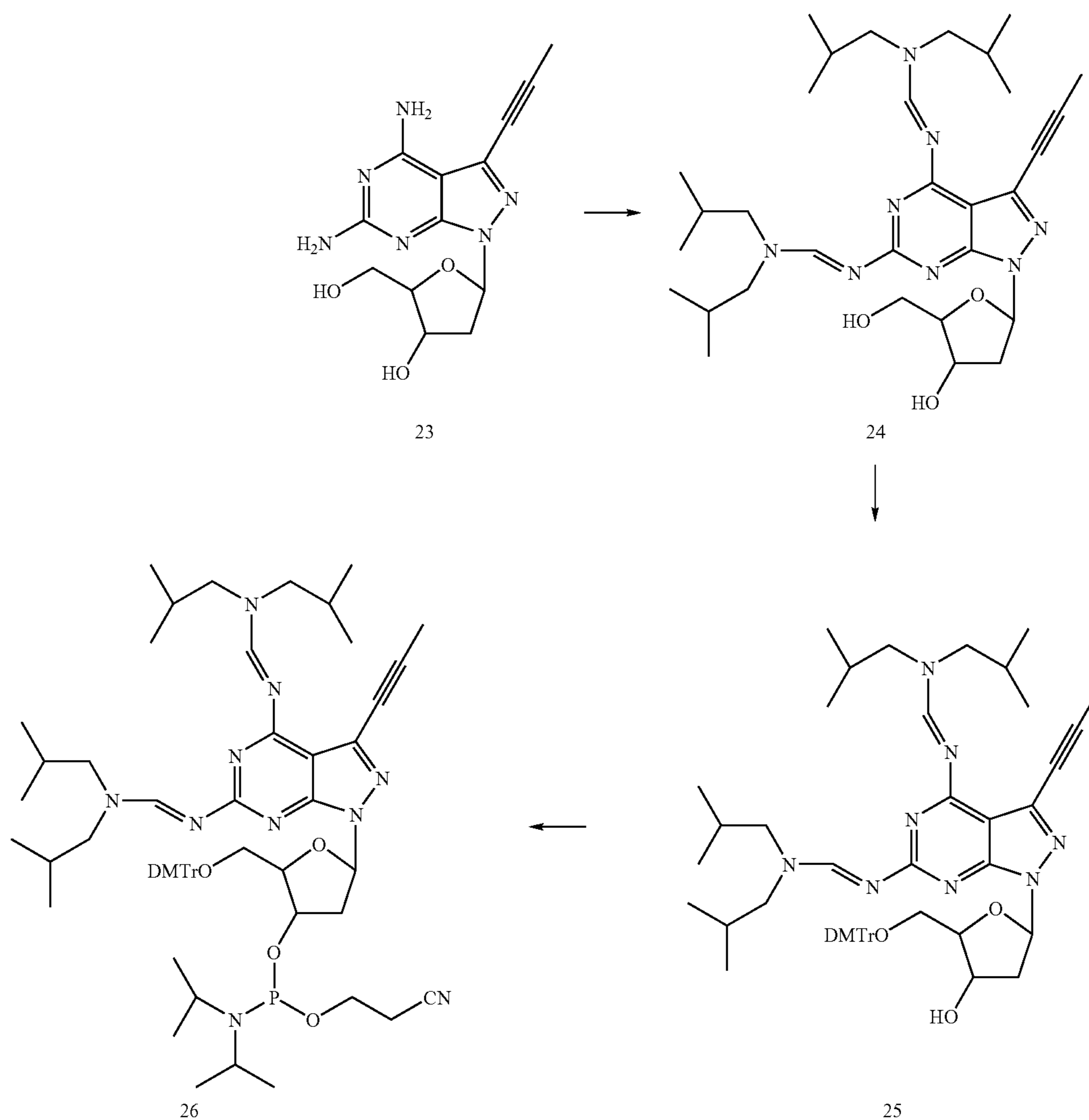
Reaction Scheme 5
