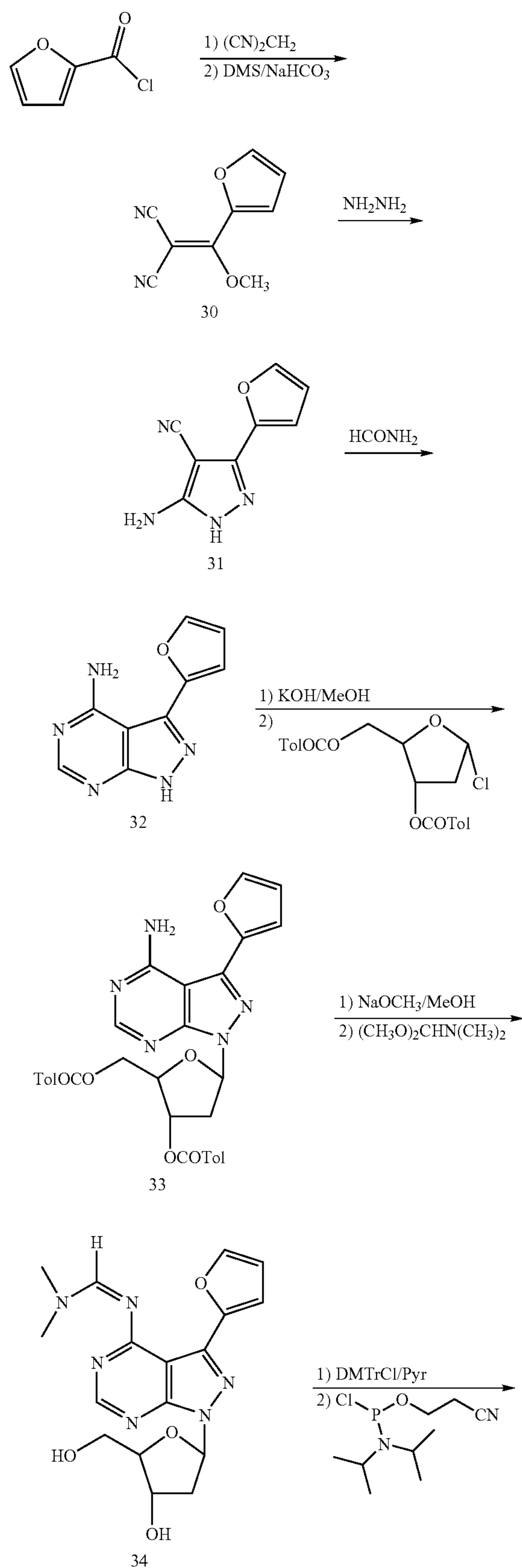
Reaction Scheme 8
