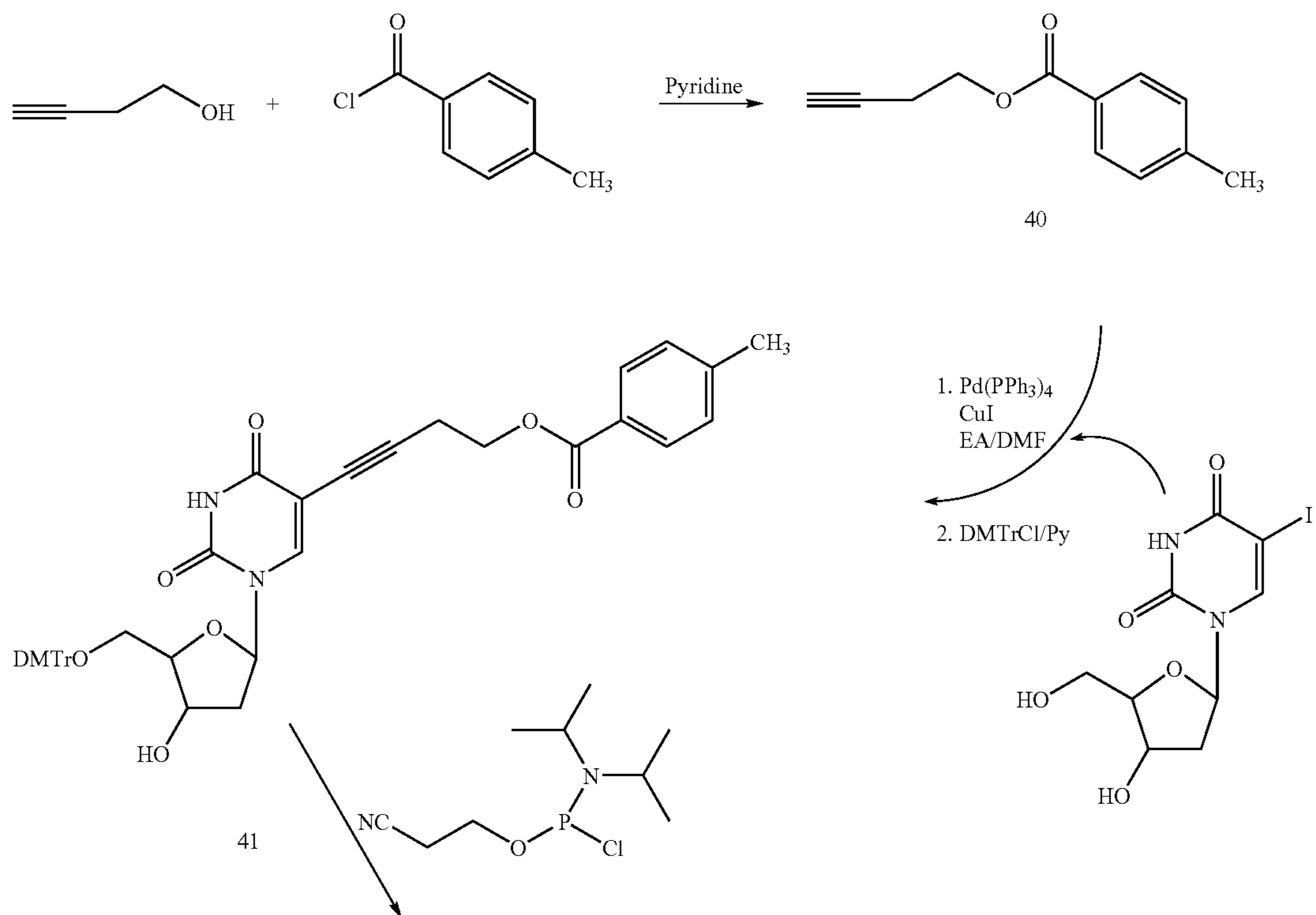
Reaction Scheme 10
