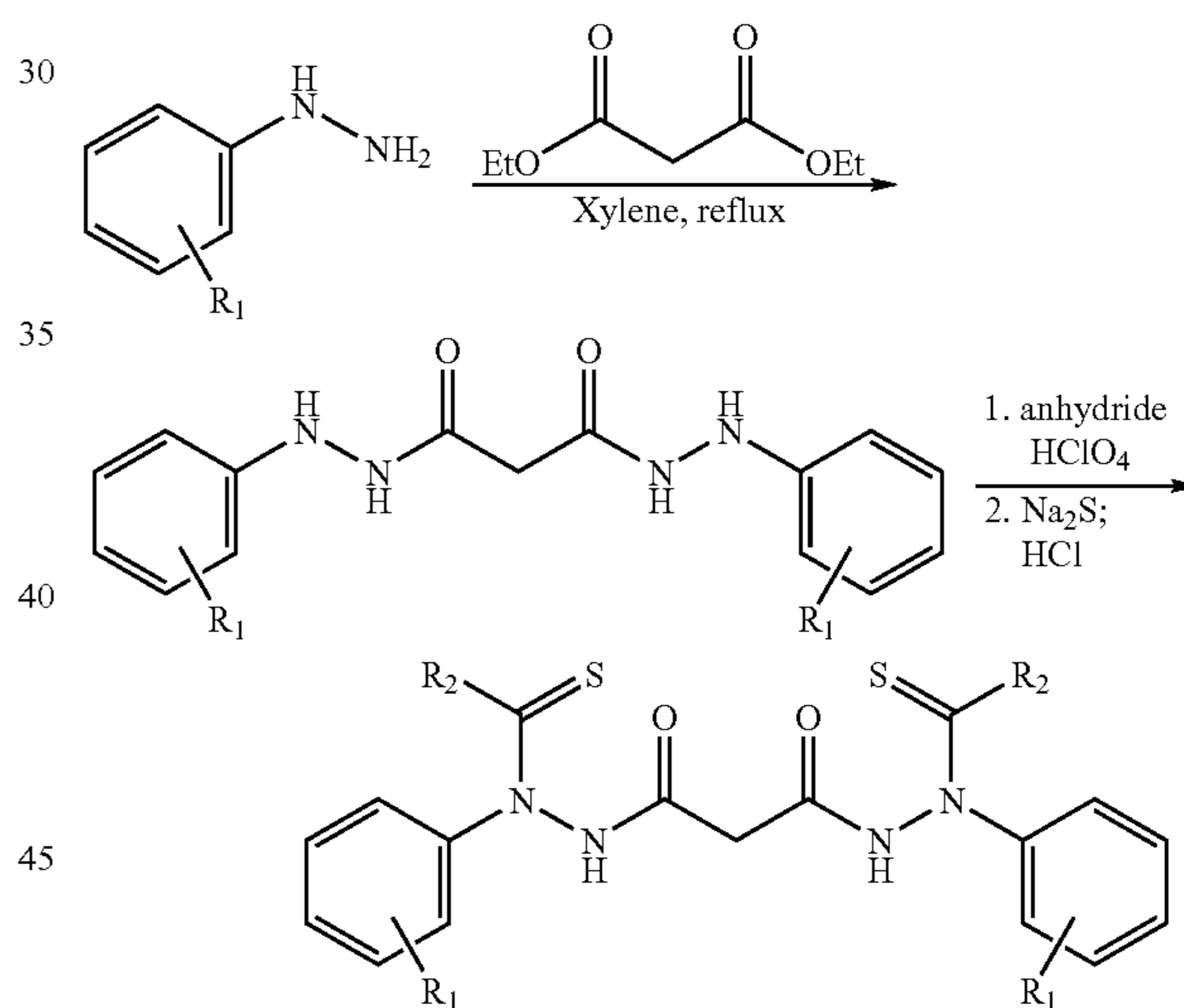
Preparation of N-Malonyl-bis[N'-phenyl-N'-(thioacetyl)hydrazide]
