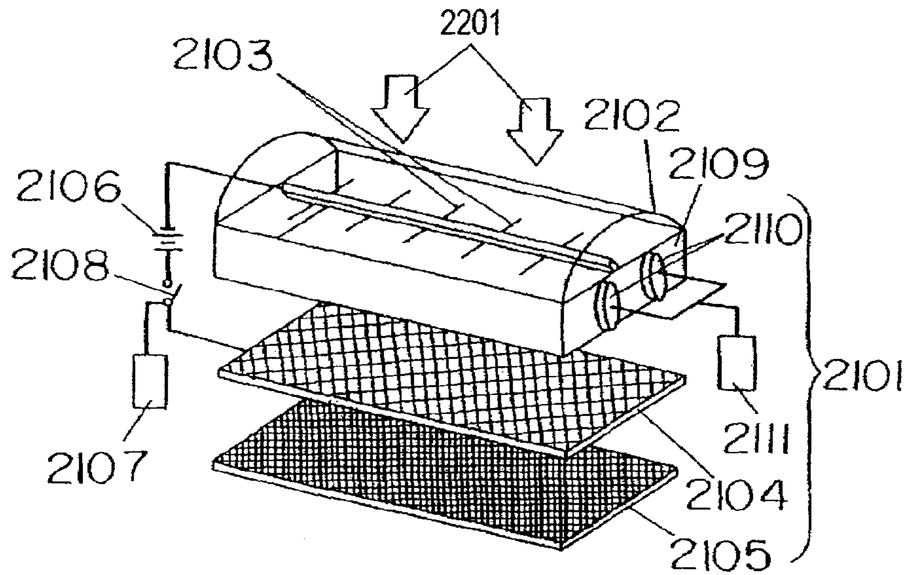
FIG. 59 PRIOR ART
