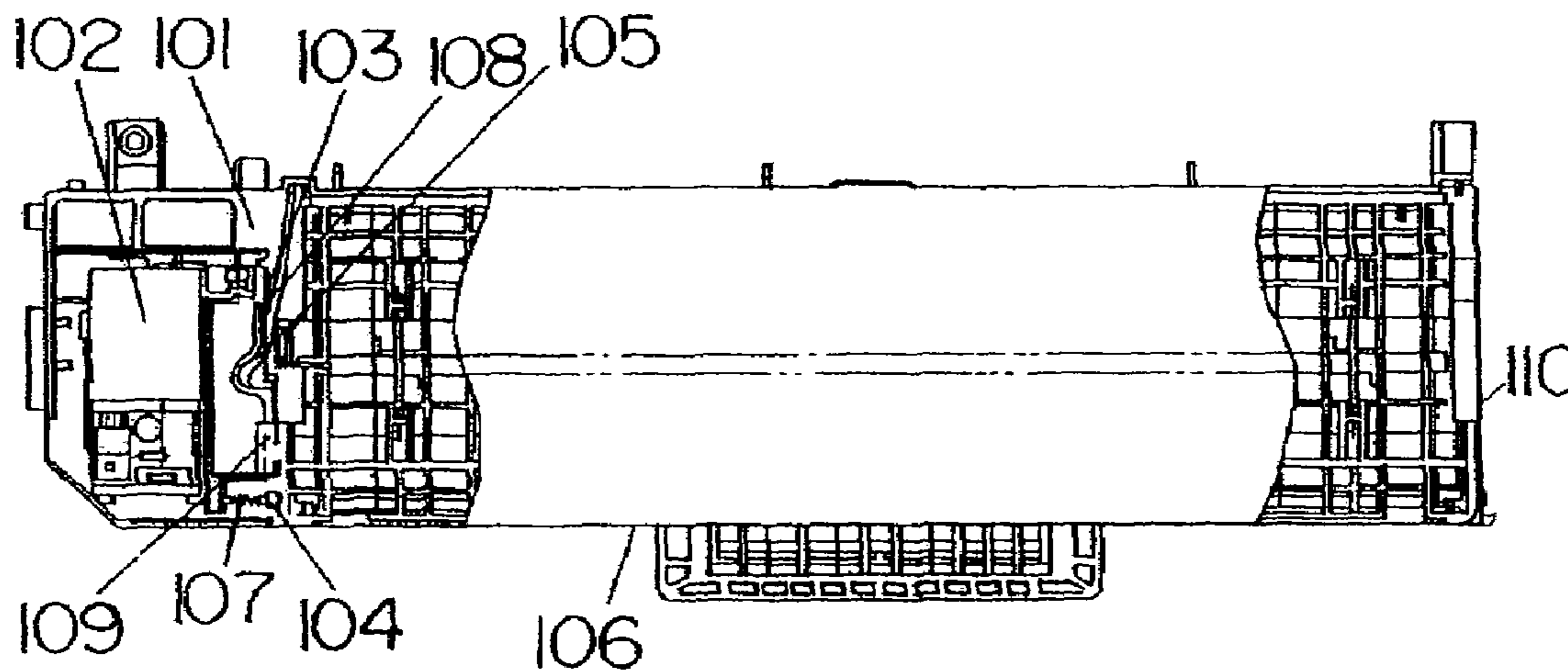
FIG. 53 PRIOR ART
