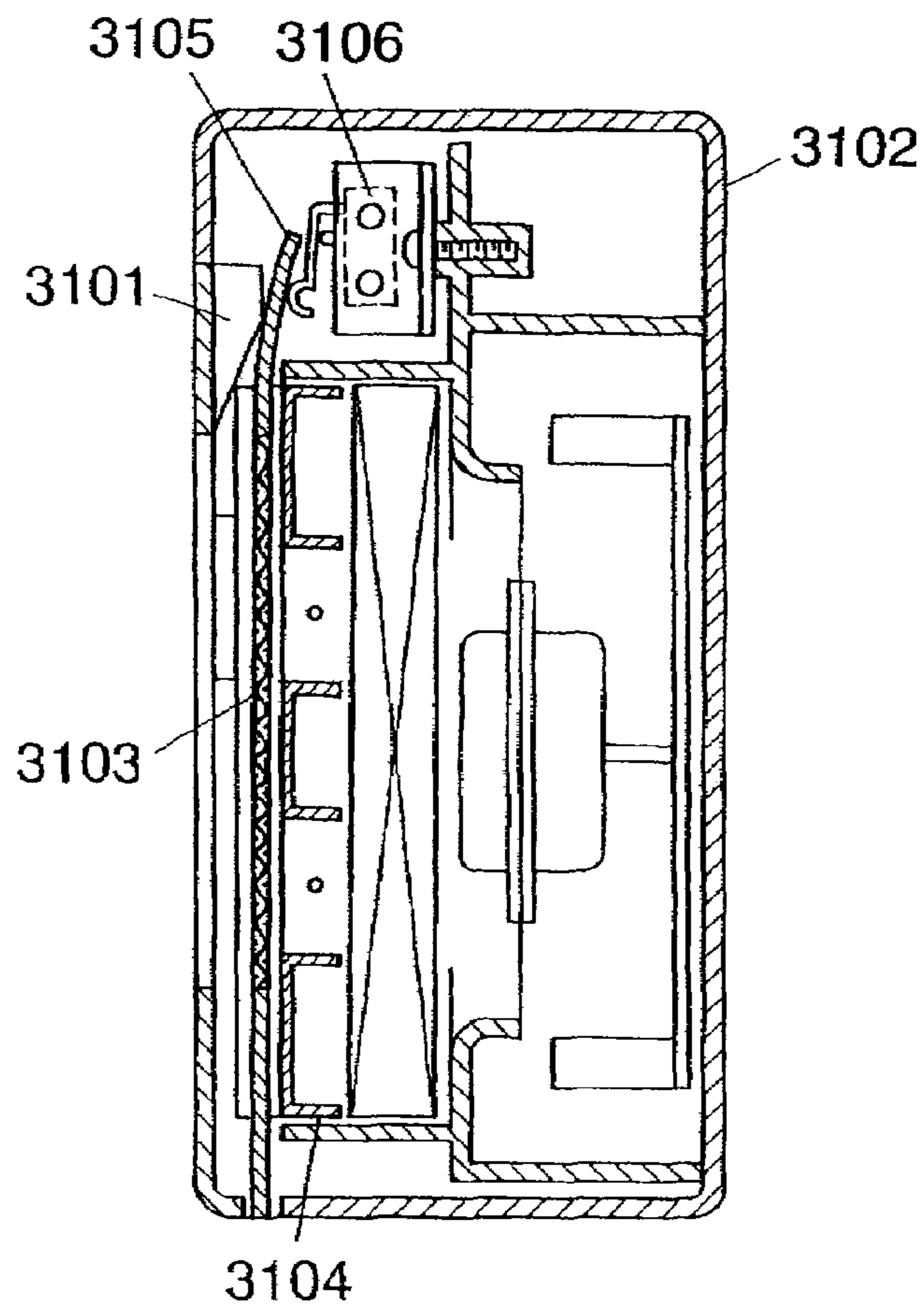
FIG. 60 PRIOR ART
