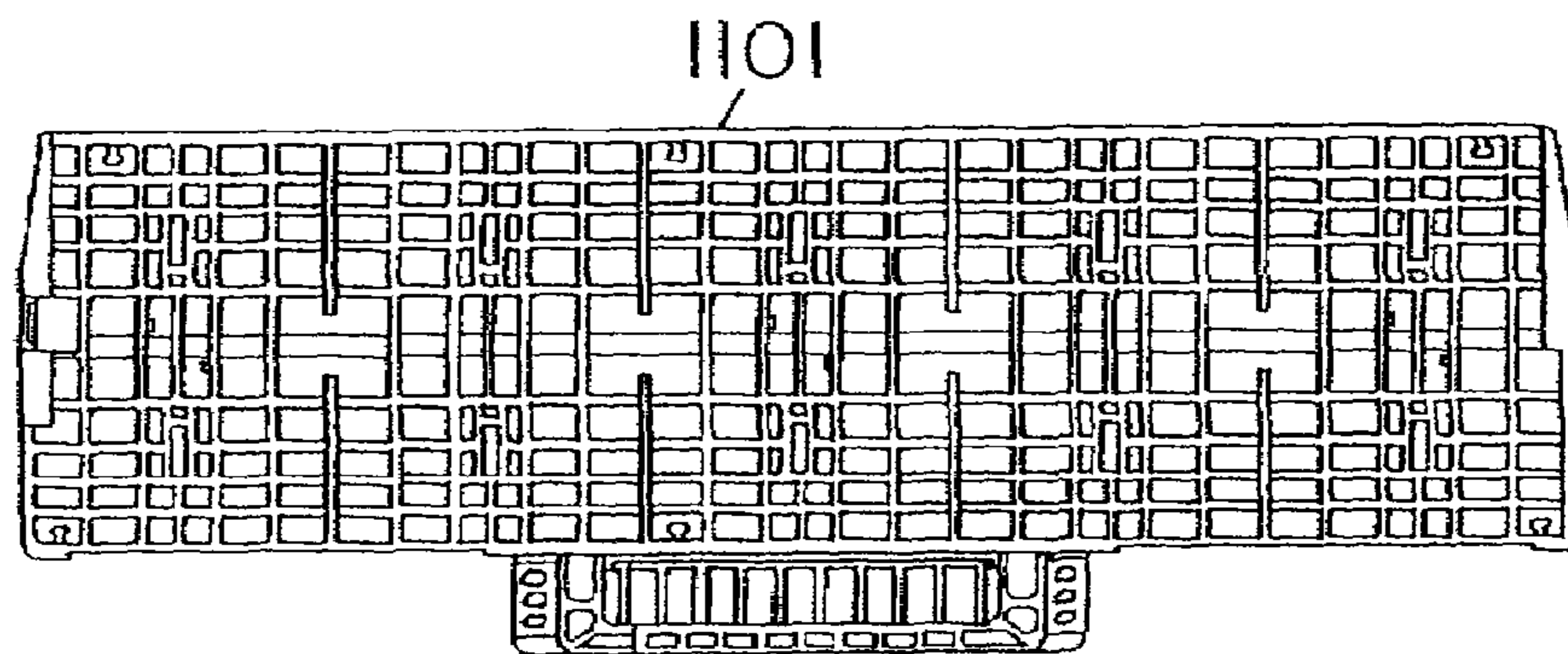
FIG. 57 PRIOR ART
