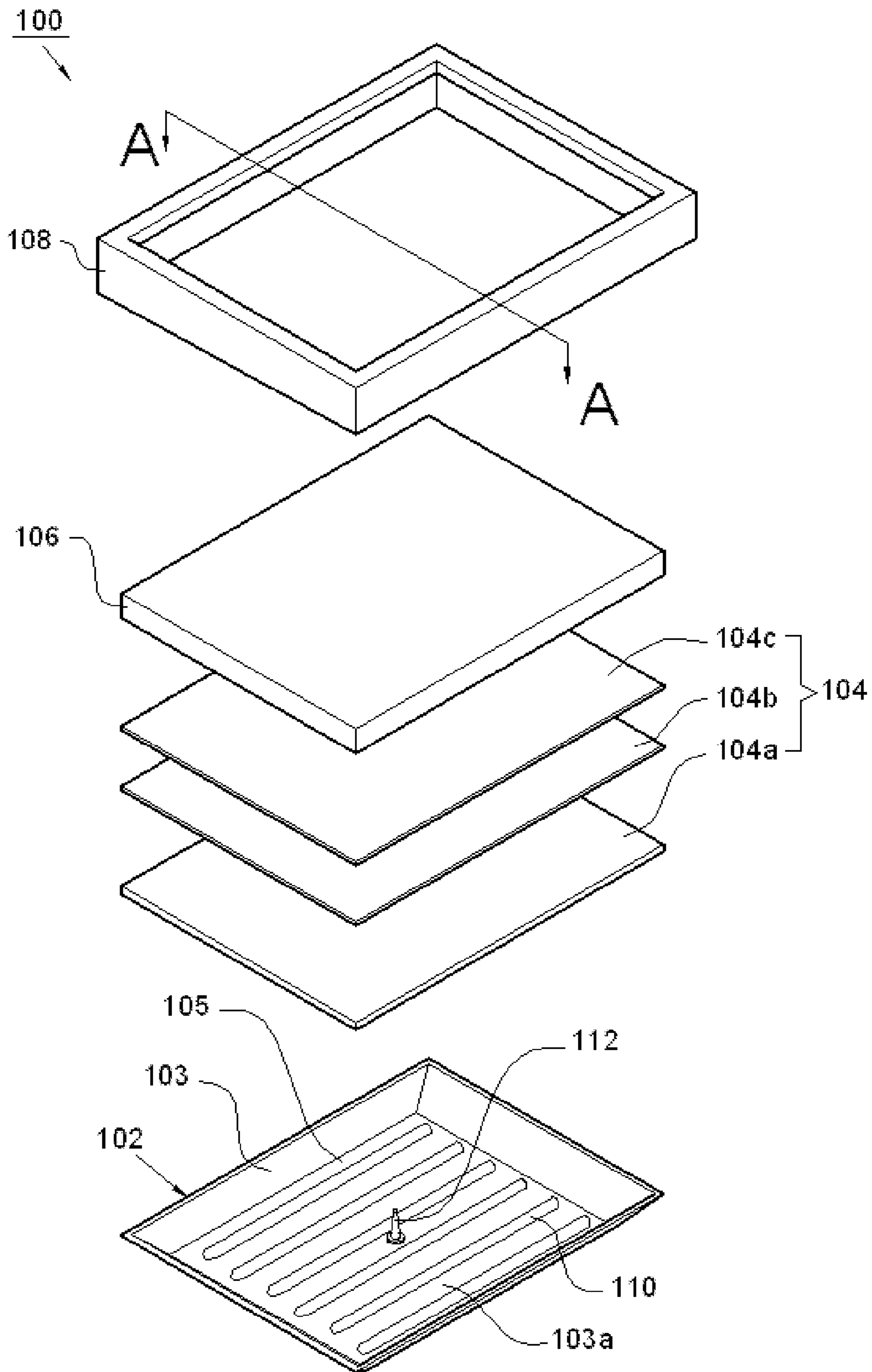
FIG. 1 (PRIOR ART)
