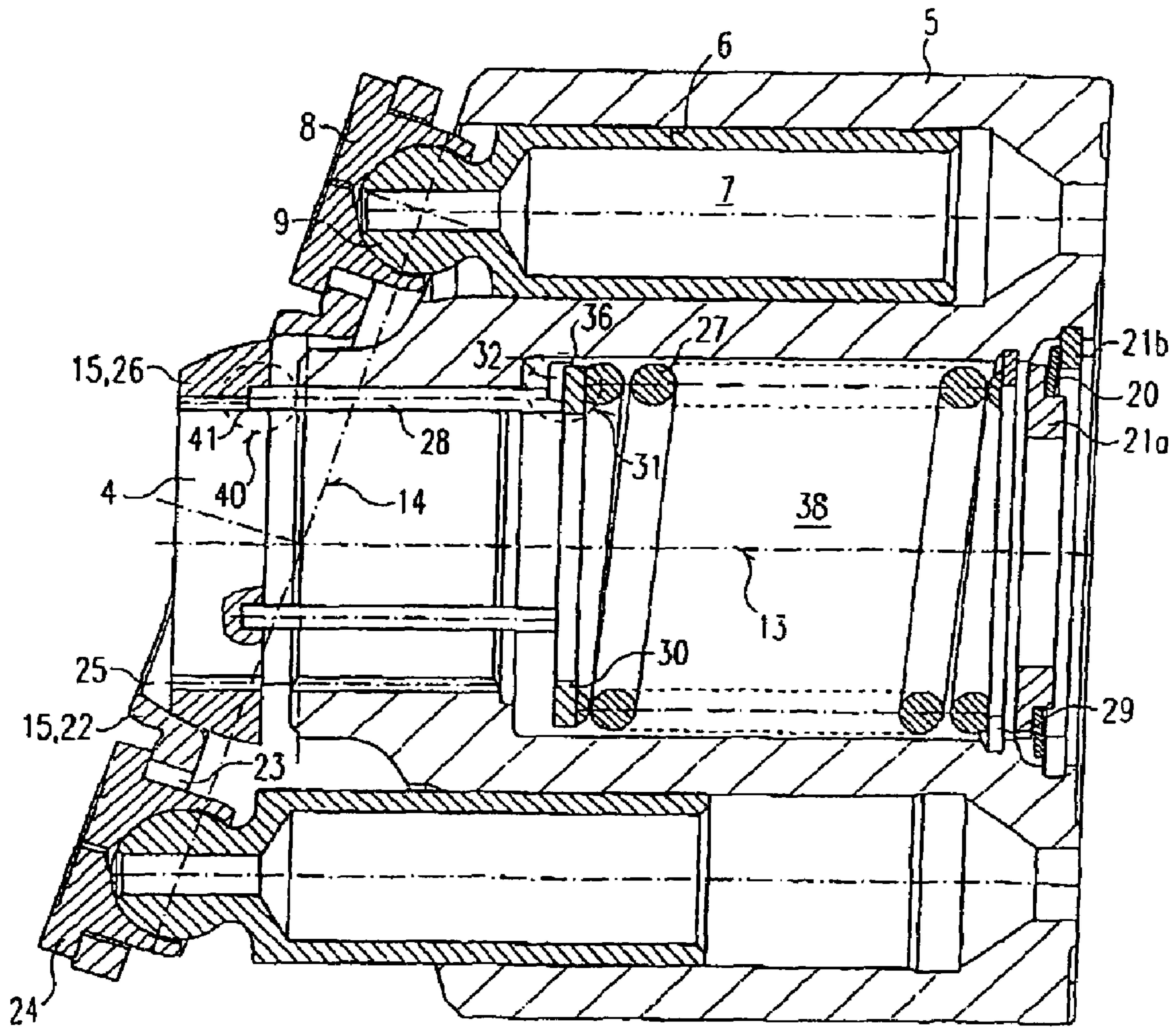
Fig. 2 Prior Art
