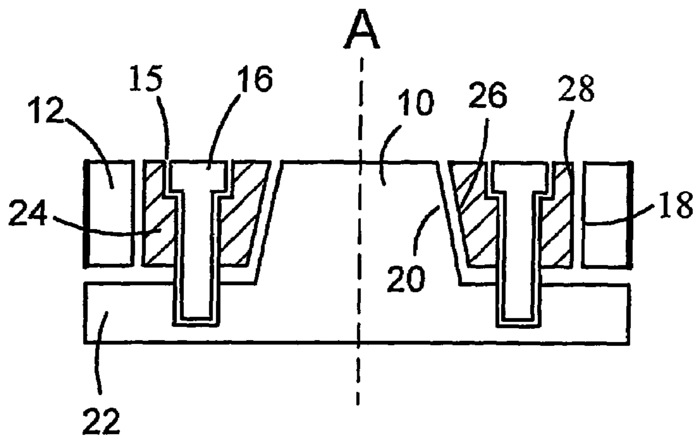
Fig 1 (PRIOR ART)
