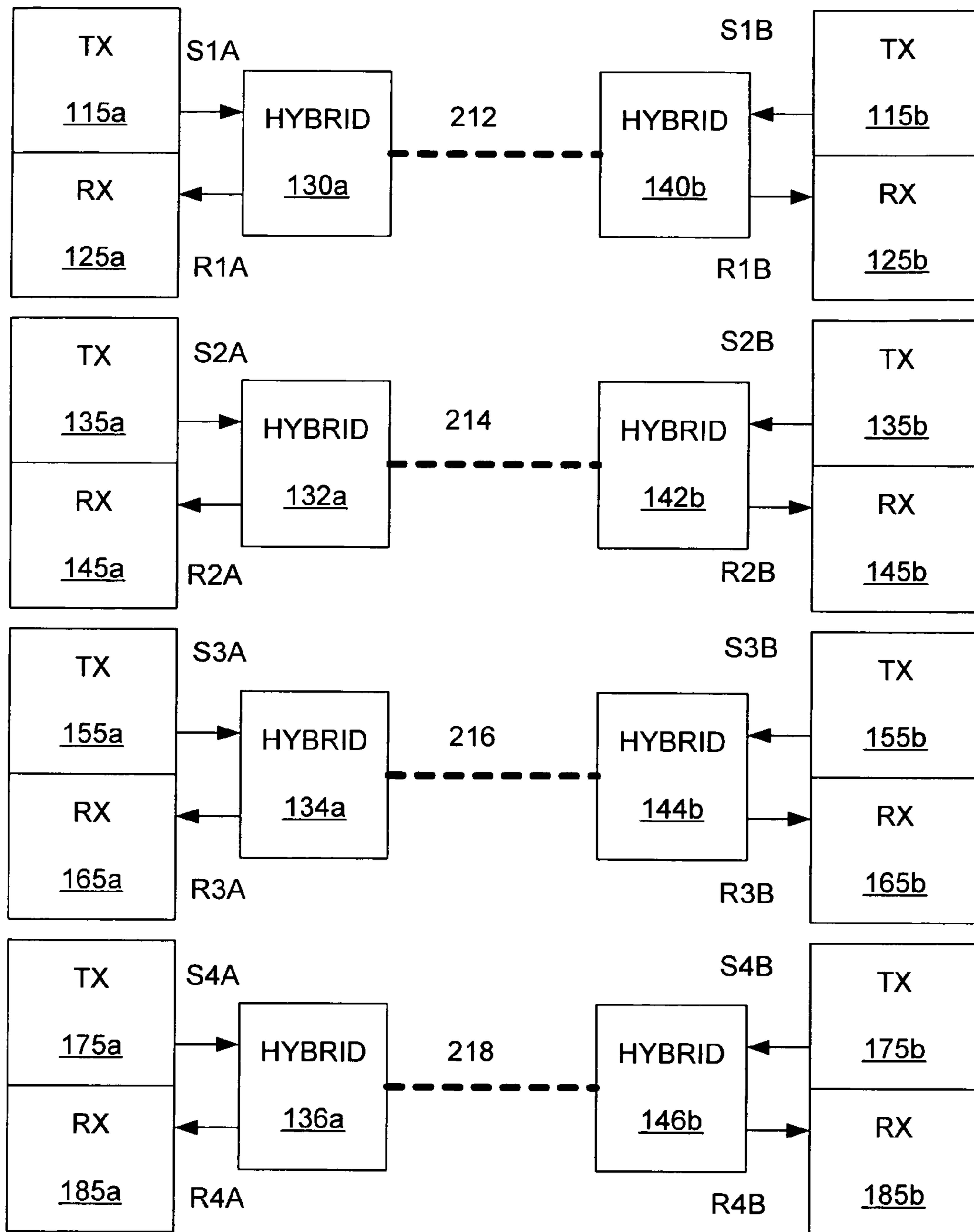
FIGURE 2 (PRIOR ART)
