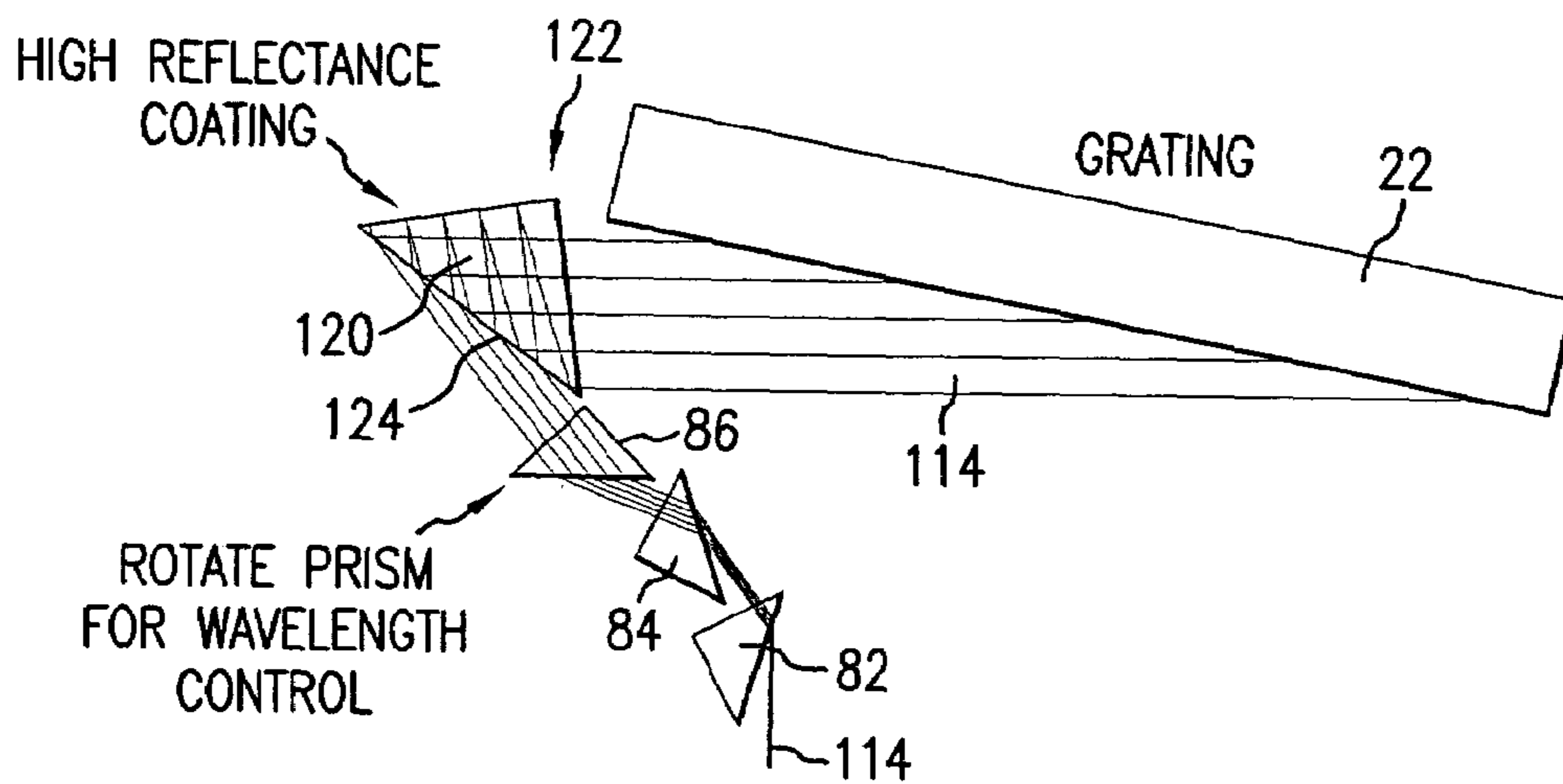
OPTICAL DESIGN FOR COMPACT LNM ROBERT BERGSTEDT 5/27/04
