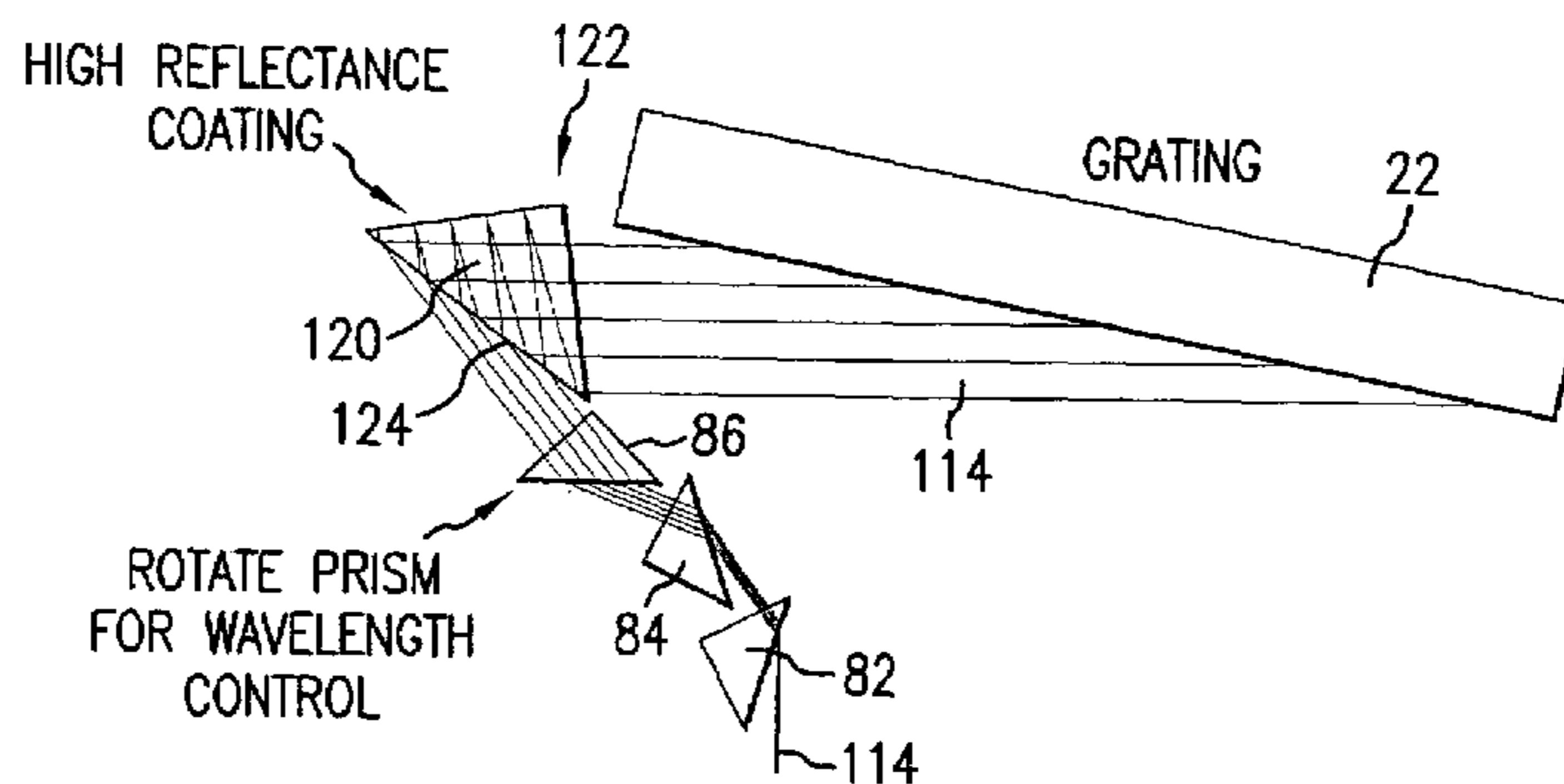
OPTICAL DESIGN FOR COMPACT LNM ROBERT BERGSTEDT 5/27/04
