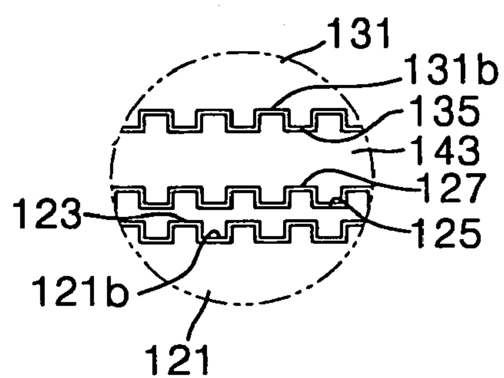
FIG. 1C (PRIOR ART)
