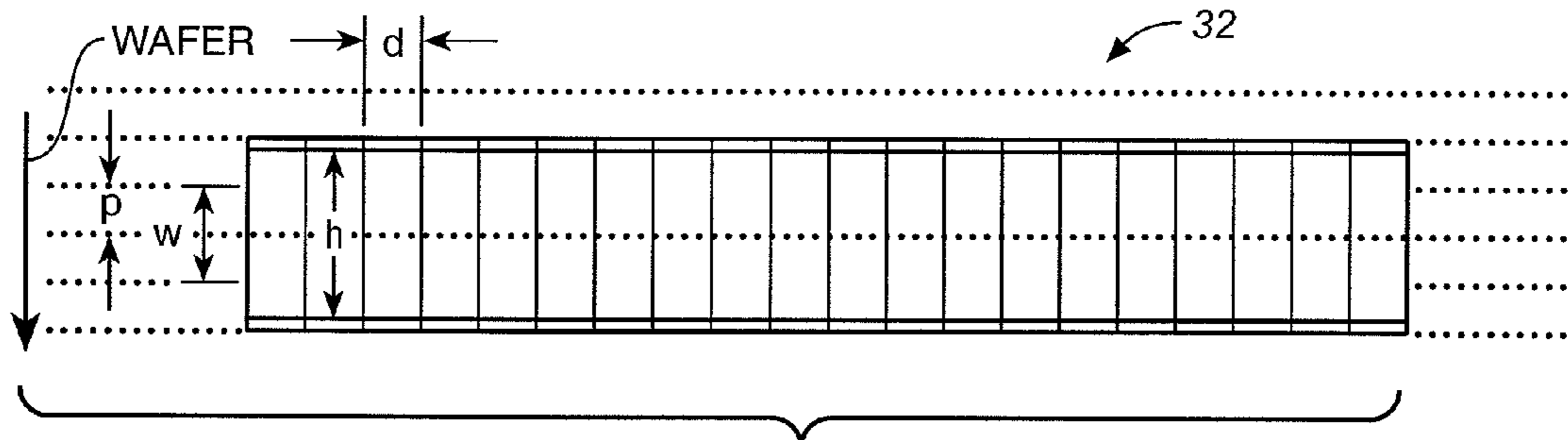
FIG. 5 (PRIOR ART)
