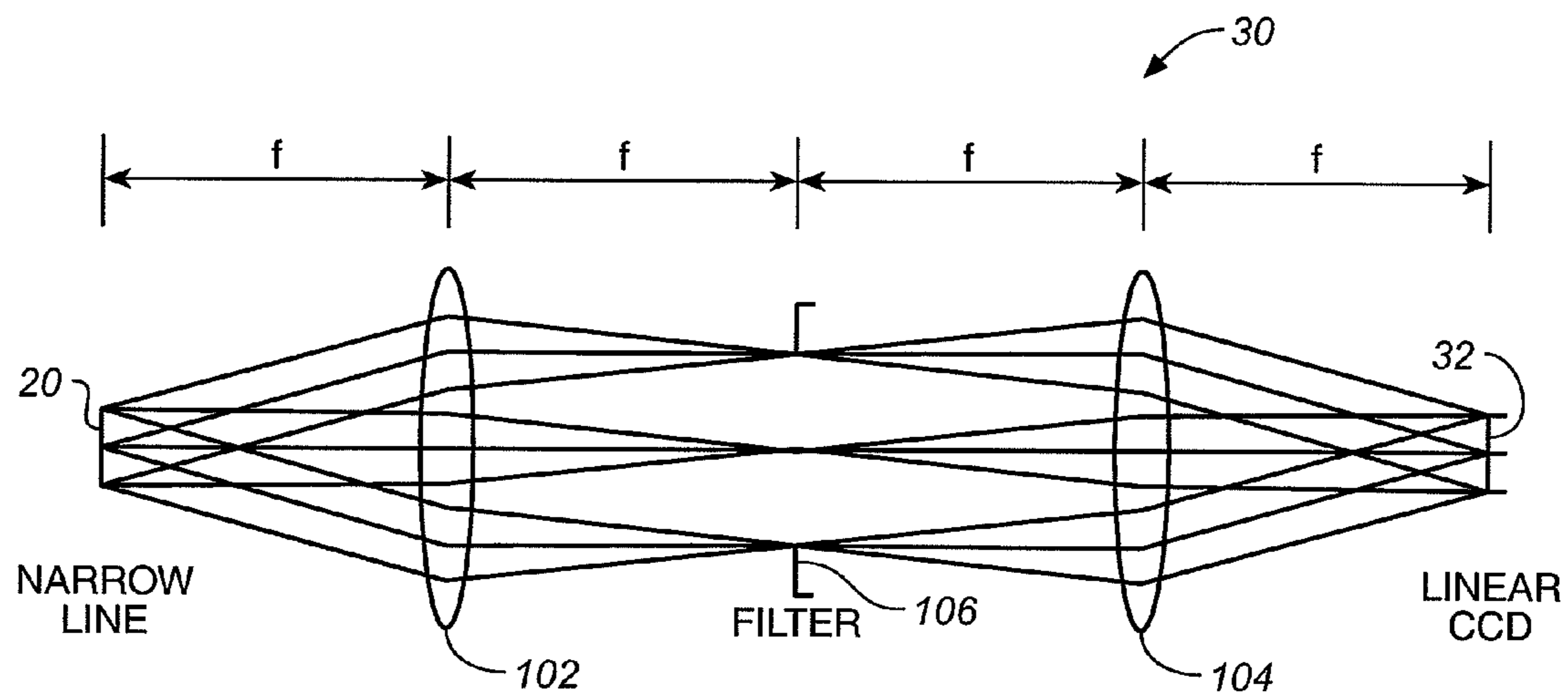
FIG. 8 (PRIOR ART)
